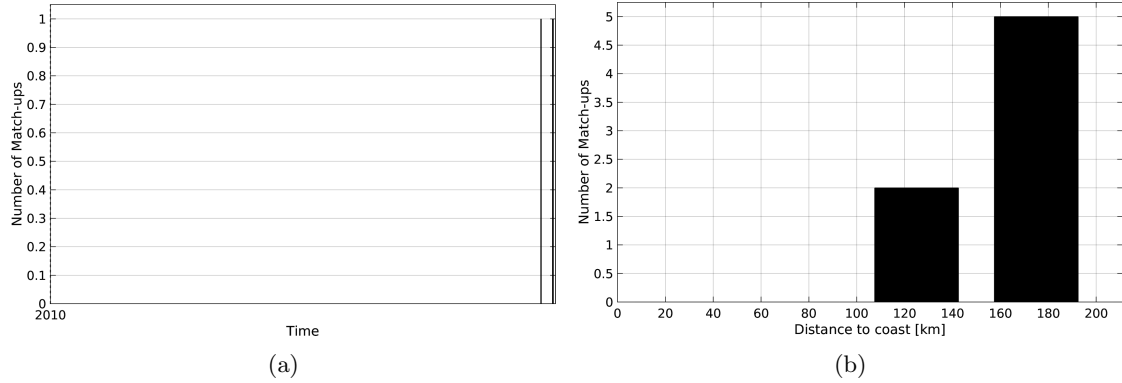
Figure 1: Number of match-ups between Sea mammals and SMOS-L3-CATDS-CECOS-IFREMER-V2-1DAY-0.5deg SSS as a function of time (a) and as function of the distance to coast (b) over the Arctic Ocean Pi-MEP region and for the full satellite product period.
