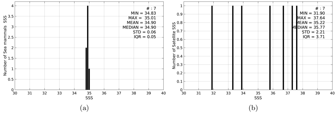
Figure 2: Histograms of SSS from Sea mammals (a) and SMOS-L3-CATDS-CECOS-IFREMER-V2-1DAY-0.5deg (b) considering all match-up pairs per bins of 0.1 over the Arctic Ocean Pi-MEP region and for the full satellite product period.
