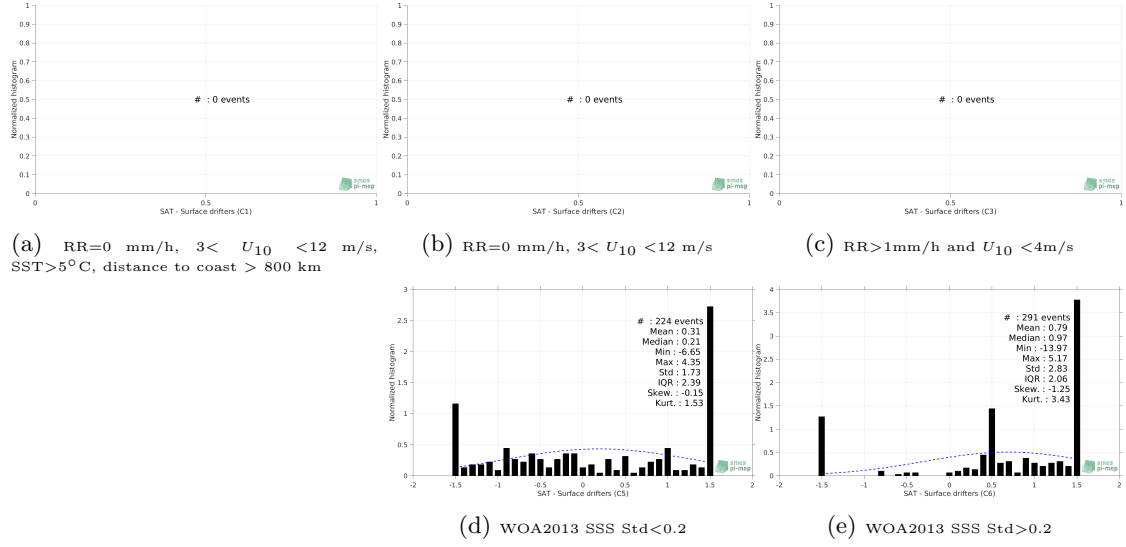
Figure 12: Normalized histogram of \Delta\text{SSS} (SMOS SSS L3 v2 - Daily - 0.5 Deg (CATDS-CECOS-IFREMER) - Surface drifters) for 5 different subdatasets corresponding to: RR=0 mm/h, 3 < U_{10} < 12 m/s, SST > 5^\circ\text{C} , distance to coast > 800 km (a), RR=0 mm/h, 3 < U_{10} < 12 m/s (b), RR > 1\text{mm/h} and U_{10} < 4\text{m/s} (c), WOA2013 SSS Std<0.2 (d), WOA2013 SSS Std>0.2 (e).
