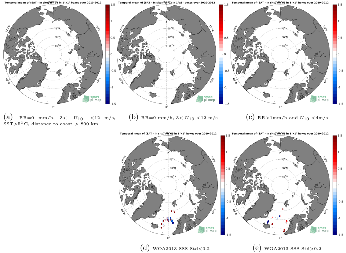
Figure 11: Temporal mean gridded over spatial boxes of size 1^{\circ}\times 1^{\circ} of \Delta\text{SSS} (SMOS L3 v2 - Daily - 0.5 Deg (CATDS-CECOS-IFREMER) - Surface drifters) for 5 different subdatasets corresponding to: \text{RR}=0 mm/h, 3 < U_{10} < 12 m/s, \text{SST} > 5^{\circ}\text{C} , distance to coast > 800 km (a), \text{RR}=0 mm/h, 3 < U_{10} < 12 m/s (b), \text{RR} > 1 mm/h and U_{10} < 4 m/s (c), WOA2013 SSS Std < 0.2 (d), WOA2013 SSS Std > 0.2 (e).
