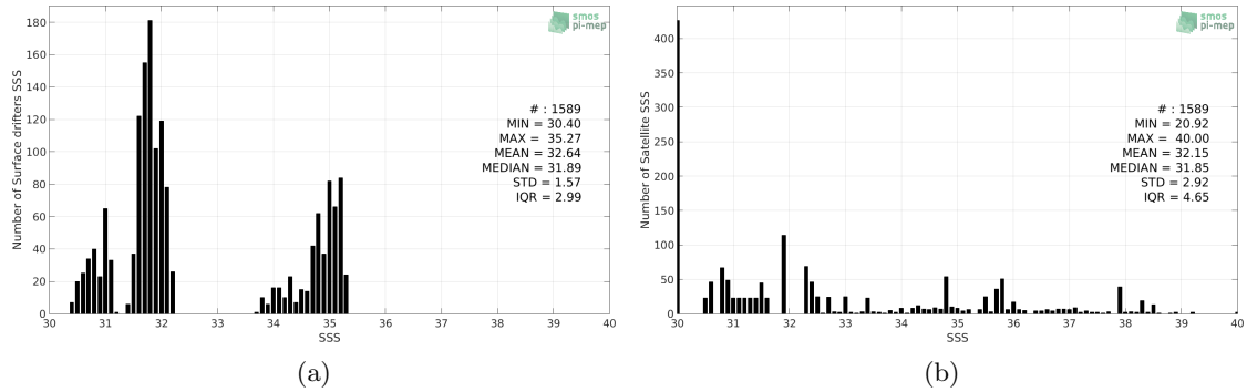
Figure 2: Histograms of SSS from Surface drifters (a) and SMOS-L3-CATDS-CECOS-IFREMER-V2-1DAY-0.5DEG (b) considering all match-up pairs per bins of 0.1 over the Arctic Ocean Pi-MEP region and for the full satellite product period.
