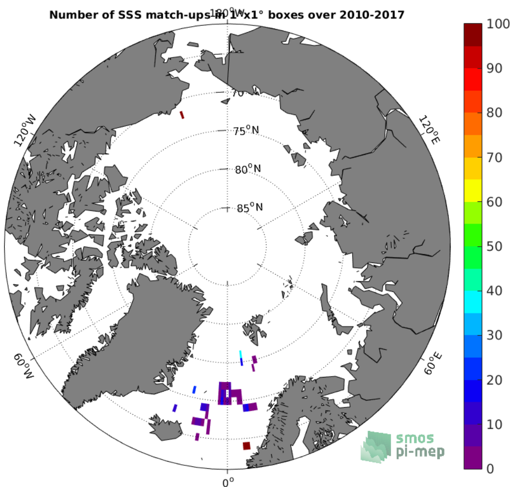
Figure 3: Number of SSS match-ups between Surface drifters SSS and the SMOS-L3-CATDS-CECOS-IFREMER-V2-1DAY-0.5DEG SSS product for the Arctic Ocean Pi-MEP region over 1^\circ \times 1^\circ boxes and for the full satellite product period.
