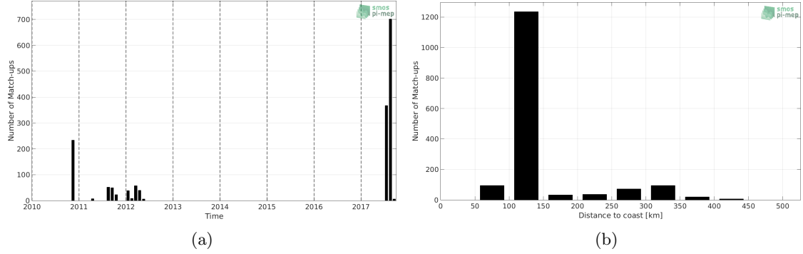
Figure 1: Number of match-ups between Surface drifters and SMOS-L3-CATDS-CECOS-IFREMER-V2-1DAY-0.5DEG SSS as a function of time (a) and as function of the distance to coast (b) over the Arctic Ocean Pi-MEP region and for the full satellite product period.
