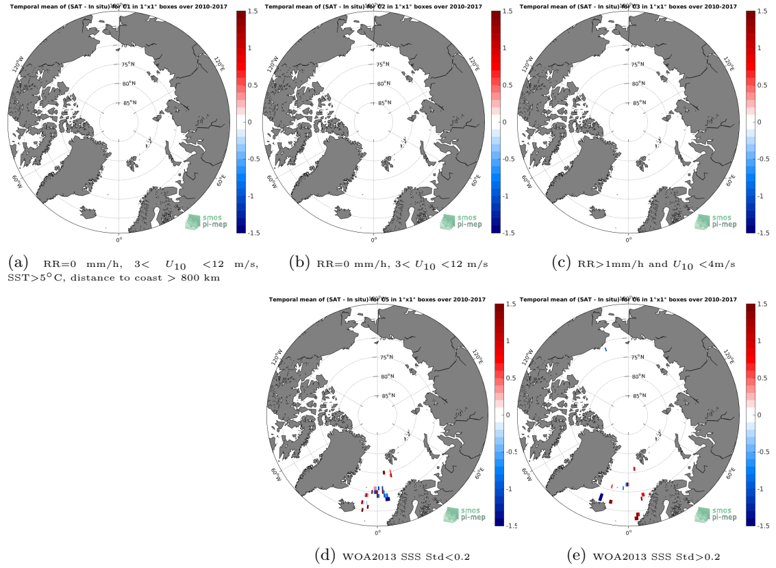
Figure 11: Temporal mean gridded over spatial boxes of size 1^\circ \times 1^\circ of \Delta SSS (SMOS-L3-CATDS-CECOS-IFREMER-V2-1DAY-0.5DEG - Surface drifters) for 5 different subdatasets corresponding to: RR=0 mm/h, 3 < U_{10} < 12 m/s, SST > 5^\circ C , distance to coast > 800 km (a), RR=0 mm/h, 3 < U_{10} < 12 m/s (b), RR > 1 mm/h and U_{10} < 4 m/s (c), WOA2013 SSS Std < 0.2 (d), WOA2013 SSS Std > 0.2 (e).
