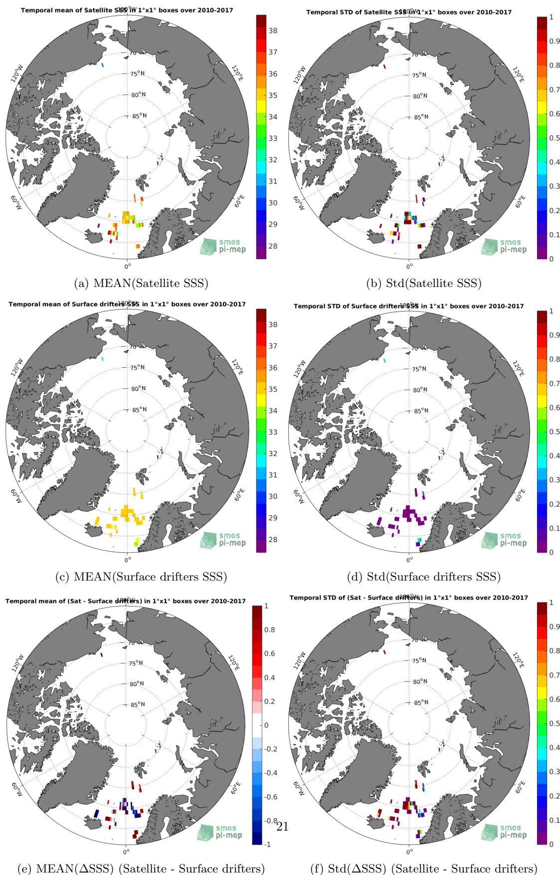
Figure 5: Temporal mean (left) and Std (right) of SSS from SMOS-L3-CATDS-CECOS-IFREMER-V2-1DAY-0.5DEG (top), Surface drifters (middle), and of \Delta SSS (Satellite - Surface drifters). Only match-up pairs are used to generate these maps.
