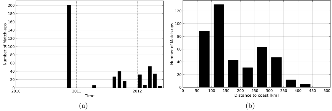
Figure 1: Number of match-ups between Surface drifters and SMOS-L3-CATDS-CECOS-IFREMER-V2-1DAY-0.5DEG SSS as a function of time (a) and as function of the distance to coast (b) over the Arctic Ocean Pi-MEP region and for the full satellite product period.
