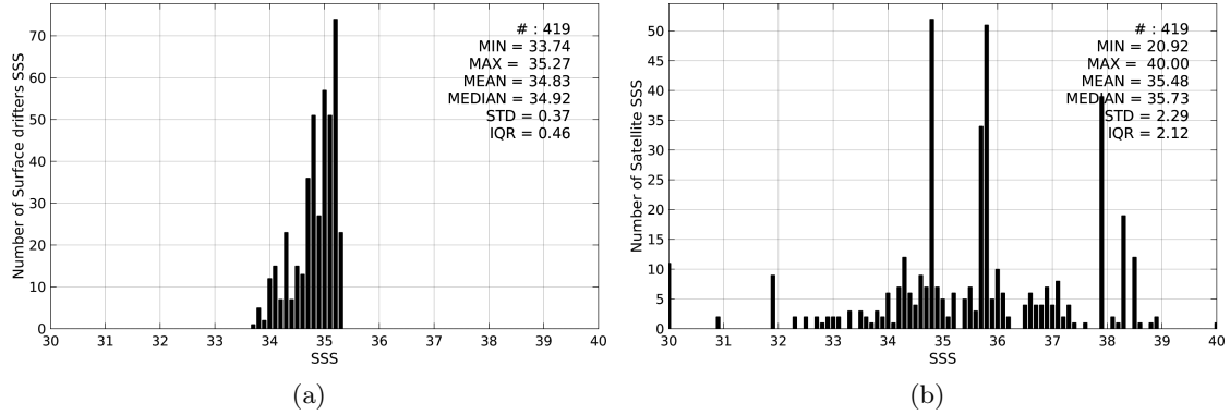
Figure 2: Histograms of SSS from Surface drifters (a) and SMOS-L3-CATDS-CECOS-IFREMER-V2-1DAY-0.5deg (b) considering all match-up pairs per bins of 0.1 over the Arctic Ocean Pi-MEP region and for the full satellite product period.
