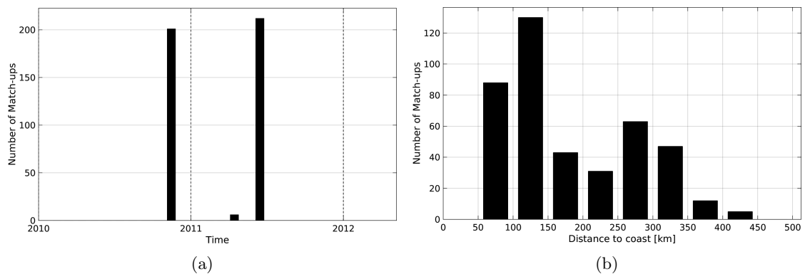
Figure 1: Number of match-ups between Surface drifters and SMOS-L3-CATDS-CECOS-IFREMER-V2-1DAY-0.5deg SSS as a function of time (a) and as function of the distance to coast (b) over the Arctic Ocean Pi-MEP region and for the full satellite product period.
