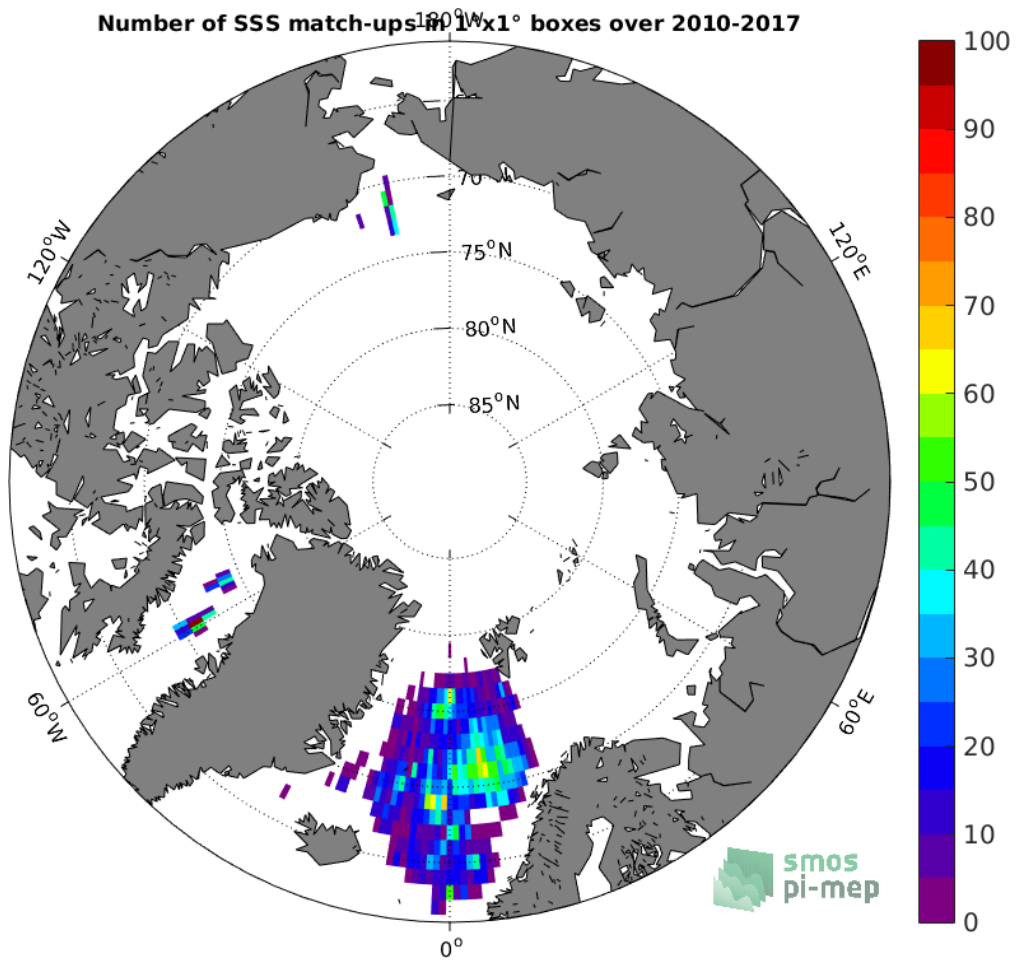
Figure 4: Number of SSS match-ups between Argo SSS and the SMOS-L3-CATDS-CECOS-IFREMER-V2-1DAY-0.5DEG SSS product for the Arctic Ocean Pi-MEP region over 1^\circ \times 1^\circ boxes and for the full satellite product period.
