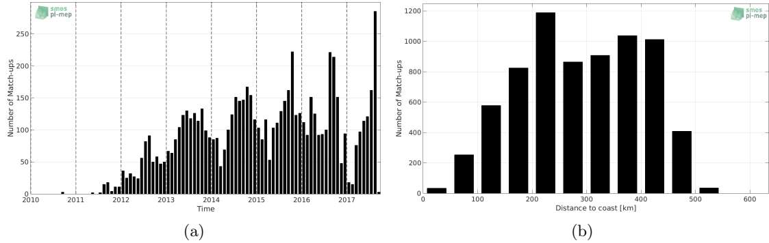
Figure 1: Number of match-ups between Argo and SMOS-L3-CATDS-CECOS-IFREMER-V2-1DAY-0.5DEG SSS as a function of time (a) and as function of the distance to coast (b) over the Arctic Ocean Pi-MEP region and for the full satellite product period.
