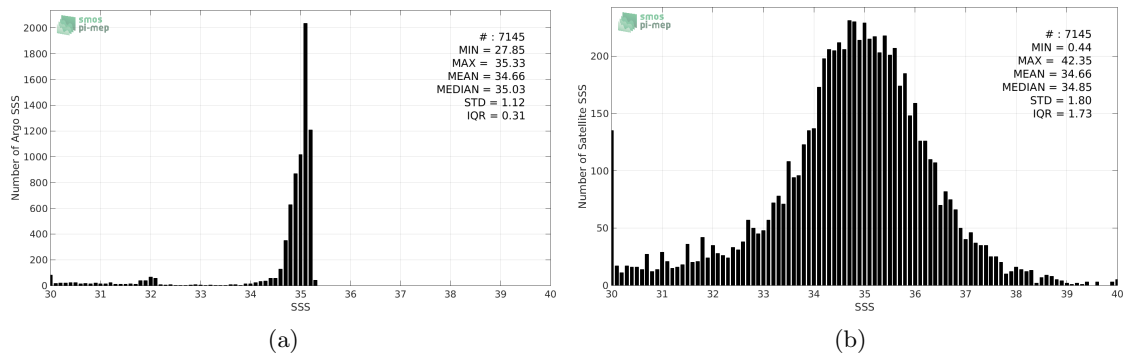
Figure 2: Histograms of SSS from Argo (a) and SMOS-L3-CATDS-CECOS-IFREMER-V2-1DAY-0.5DEG (b) considering all match-up pairs per bins of 0.1 over the Arctic Ocean Pi-MEP region and for the full satellite product period.
