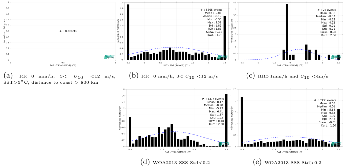
Figure 15: Normalized histogram of \Delta SSS (SMOS SSS L3 v335 - Monthly - 25 km (CATDS-CPDC) - TSG (SAMOS)) for 5 different subdatasets corresponding to: RR=0 mm/h, 3 < U_{10} < 12 m/s, SST > 5°C, distance to coast > 800 km (a), RR=0 mm/h, 3 < U_{10} < 12 m/s (b), RR > 1mm/h and U_{10} < 4 m/s (c), WOA2013 SSS Std < 0.2 (d), WOA2013 SSS Std > 0.2 (e).
