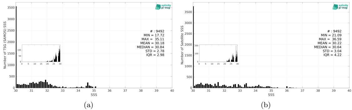
Figure 3: Histograms of SSS from TSG (SAMOS) (a) and SMOS SSS L3 v335 - Monthly - 25 km (CATDS-CPDC) (b) considering all match-up pairs per bins of 0.1 over the Arctic Ocean Pi-MEP region and for the full satellite product period.
