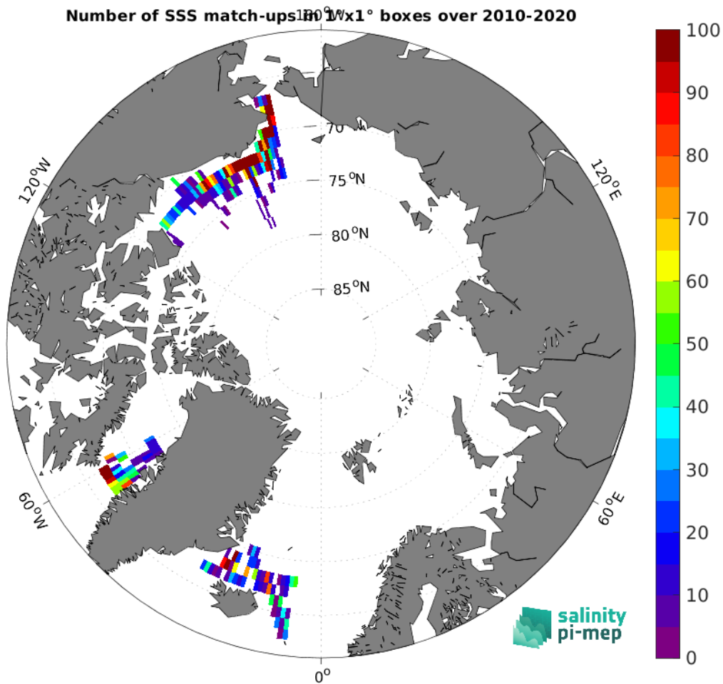
Figure 5: Number of SSS match-ups between TSG (SAMOS) SSS and the SMOS SSS L3 v335 - Monthly - 25 km (CATDS-CPDC) SSS product for the Arctic Ocean Pi-MEP region over 1^\circ \times 1^\circ boxes and for the full satellite product period.
