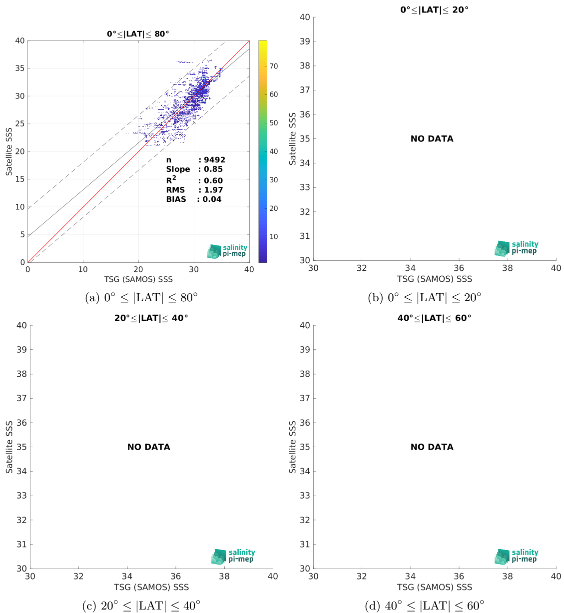
Figure 10: Contour maps of the concentration of SMOS SSS L3 v335 - Monthly - 25 km (CATDS-CPDC) SSS (y-axis) versus TSG (SAMOS) SSS (x-axis) at match-up pairs for different latitude bands. For each plot, the red line shows x=y . The black thin and dashed lines indicate a linear fit through the data cloud and the \pm 95\% confidence levels, respectively. The number match-up pairs n , the slope and R^2 coefficient of the linear fit, the root mean square (RMS) and the mean bias between satellite and in situ data are indicated for each latitude band in each plots.
