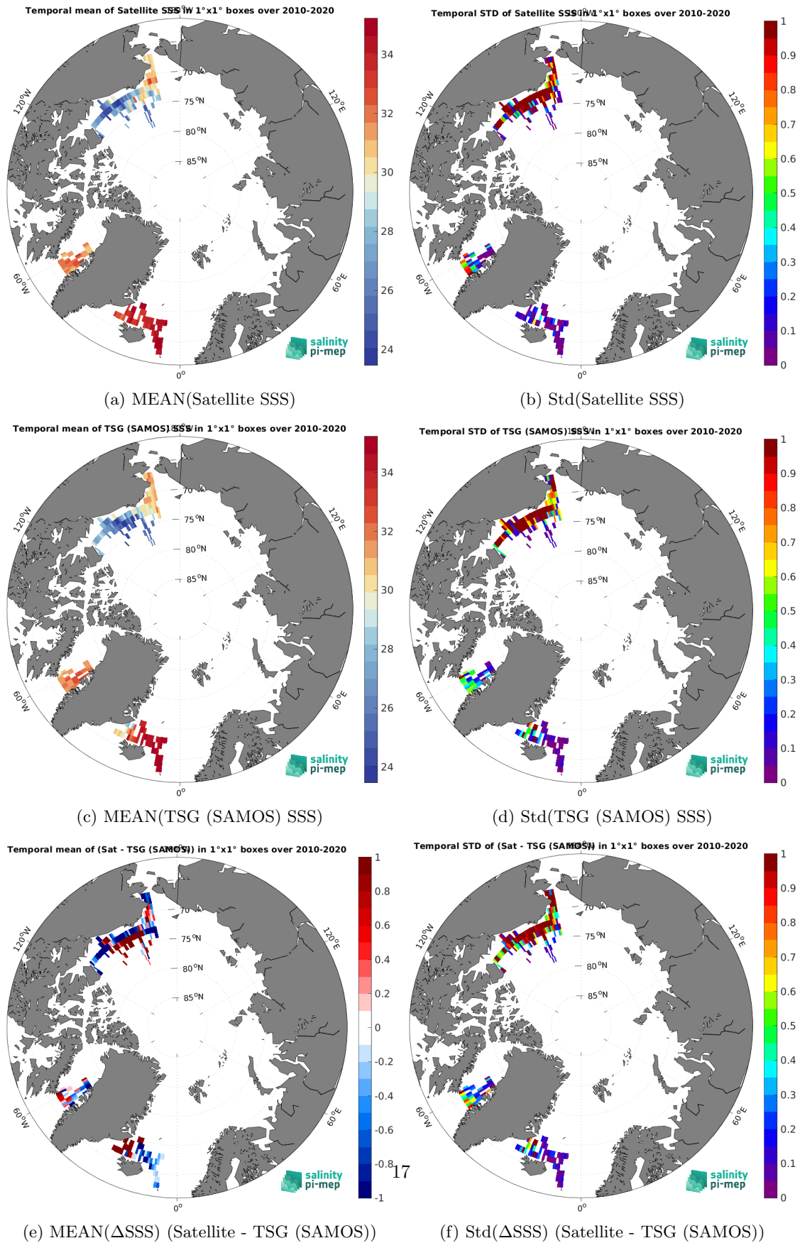
Figure 7: Temporal mean (left) and Std (right) of SSS from SMOS SSS L3 v335 - Monthly - 25 km (CATDS-CPDC) (top), TSG (SAMOS) (middle), and of \Delta SSS (Satellite - TSG (SAMOS)). Only match-up pairs are used to generate these maps.
