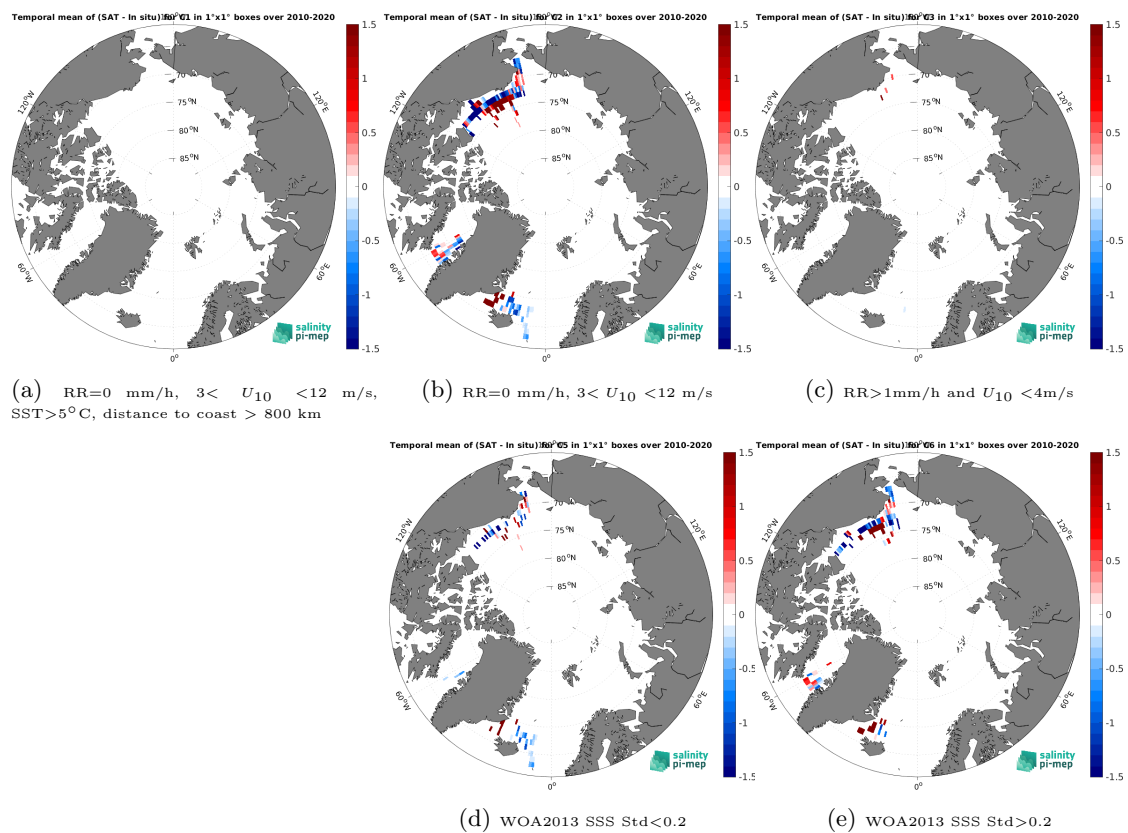
Figure 14: Temporal mean gridded over spatial boxes of size 1^\circ \times 1^\circ of \Delta SSS (SMOS SSS L3 v335 - Monthly - 25 km (CATDS-CPDC) - TSG (SAMOS)) for 5 different subdatasets corresponding to: RR=0 mm/h, 3 < U_{10} < 12 m/s, SST > 5°C, distance to coast > 800 km (a), RR=0 mm/h, 3 < U_{10} < 12 m/s (b), RR > 1mm/h and U_{10} < 4 m/s (c), WOA2013 SSS Std < 0.2 (d), WOA2013 SSS Std > 0.2 (e).
