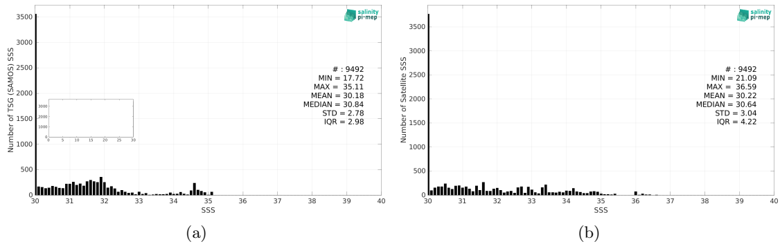
Figure 2: Histograms of SSS from TSG (SAMOS) (a) and SMOS SSS L3 v335 - Monthly - 25 km (CATDS-CPDC) (b) considering all match-up pairs per bins of 0.1 over the Arctic Ocean Pi-MEP region and for the full satellite product period.
