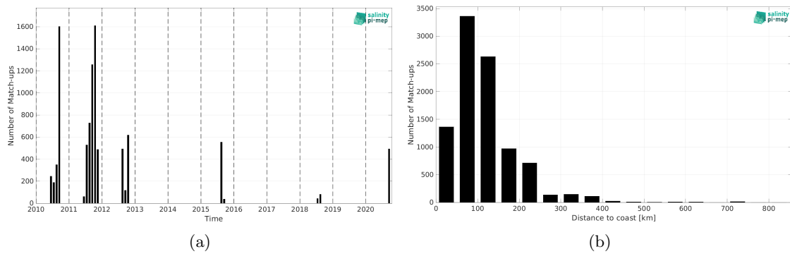
Figure 1: Number of match-ups between TSG (SAMOS) and SMOS SSS L3 v335 - Monthly - 25 km (CATDS-CPDC) SSS as a function of time (a) and as function of the distance to coast (b) over the Arctic Ocean Pi-MEP region and for the full satellite product period.
