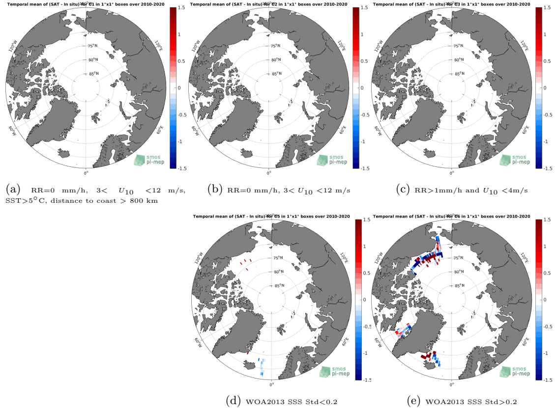
Figure 12: Temporal mean gridded over spatial boxes of size 1^{\circ} \times 1^{\circ} of \Delta\text{SSS} (SMOS SSS L3 v335 - Monthly - 25 km (CATDS-CPDC) - TSG (SAMOS)) for 5 different subdatasets corresponding to: RR=0 mm/h, 3 < U_{10} < 12 m/s, SST >5^{\circ}\text{C} , distance to coast > 800 km (a), RR=0 mm/h, 3 < U_{10} < 12 m/s (b), RR >1 mm/h and U_{10} < 4 m/s (c), WOA2013 SSS Std <0.2 (d), WOA2013 SSS Std >0.2 (e).
