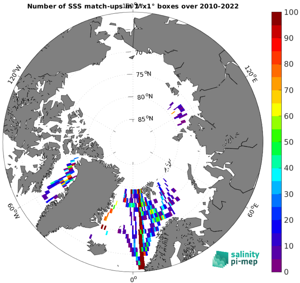
Figure 5: Number of SSS match-ups between TSG (Polarstern) SSS and the SMOS SSS L3 v335 - Monthly - 25 km (CATDS-CPDC) SSS product for the Arctic Ocean Pi-MEP region over 1^\circ \times 1^\circ boxes and for the full satellite product period.
