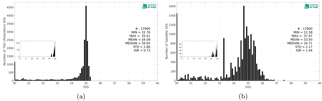
Figure 3: Histograms of SSS from TSG (Polarstern) (a) and SMOS SSS L3 v335 - Monthly - 25 km (CATDS-CPDC) (b) considering all match-up pairs per bins of 0.1 over the Arctic Ocean Pi-MEP region and for the full satellite product period.
