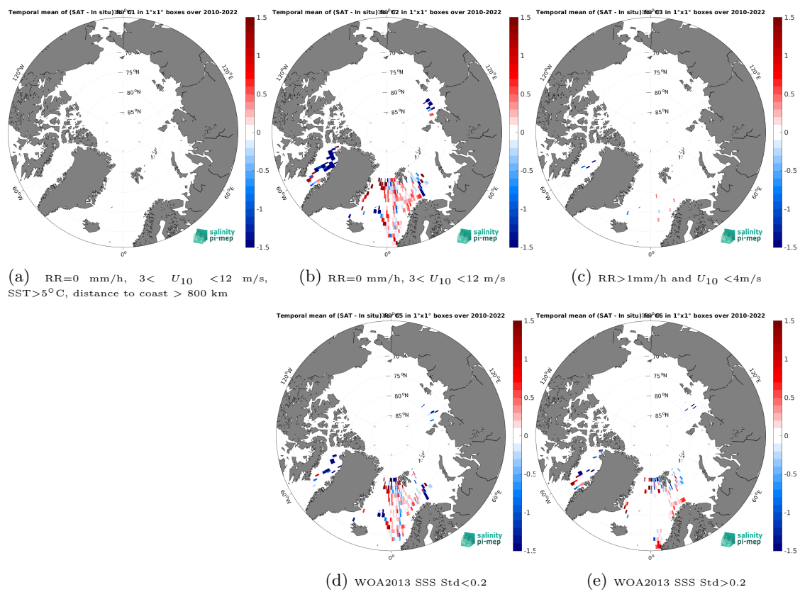
Figure 14: Temporal mean gridded over spatial boxes of size 1^\circ \times 1^\circ of \Delta SSS (SMOS SSS L3 v335 - Monthly - 25 km (CATDS-CPDC) - TSG (Polarstern)) for 5 different subdatasets corresponding to: RR=0 mm/h, 3 < U_{10} < 12 m/s, SST > 5°C, distance to coast > 800 km (a), RR=0 mm/h, 3 < U_{10} < 12 m/s (b), RR > 1mm/h and U_{10} < 4 m/s (c), WOA2013 SSS Std < 0.2 (d), WOA2013 SSS Std > 0.2 (e).
