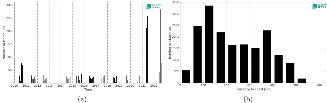
Figure 2: Number of match-ups between TSG (Polarstern) and SMOS SSS L3 v335 - Monthly - 25 km (CATDS-CPDC) SSS as a function of time (a) and as function of the distance to coast (b) over the Arctic Ocean Pi-MEP region and for the full satellite product period.
