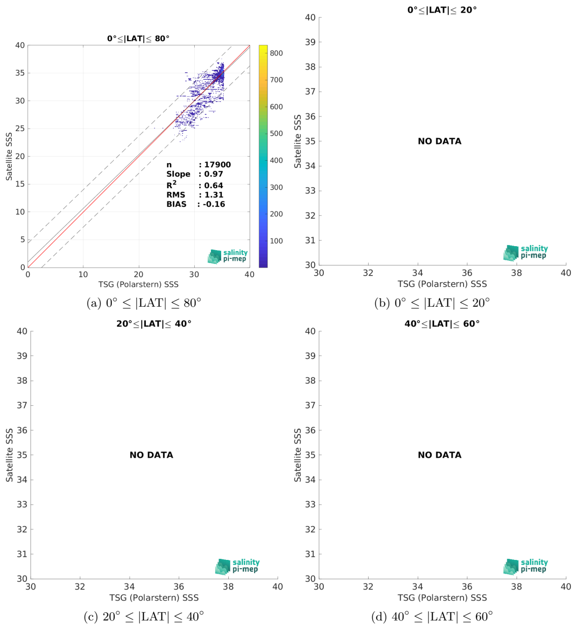
Figure 10: Contour maps of the concentration of SMOS SSS L3 v335 - Monthly - 25 km (CATDS-CPDC) SSS (y-axis) versus TSG (Polarstern) SSS (x-axis) at match-up pairs for different latitude bands. For each plot, the red line shows x=y . The black thin and dashed lines indicate a linear fit through the data cloud and the \pm 95\% confidence levels, respectively. The number match-up pairs n , the slope and R^2 coefficient of the linear fit, the root mean square (RMS) and the mean bias between satellite and in situ data are indicated for each latitude band in each plots.
