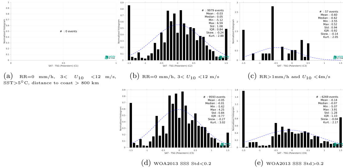
Figure 15: Normalized histogram of \Delta SSS (SMOS SSS L3 v335 - Monthly - 25 km (CATDS-CPDC) - TSG (Polarstern)) for 5 different subdatasets corresponding to: RR=0 mm/h, 3 < U_{10} < 12 m/s, SST > 5°C, distance to coast > 800 km (a), RR=0 mm/h, 3 < U_{10} < 12 m/s (b), RR > 1mm/h and U_{10} < 4 m/s (c), WOA2013 SSS Std < 0.2 (d), WOA2013 SSS Std > 0.2 (e).
