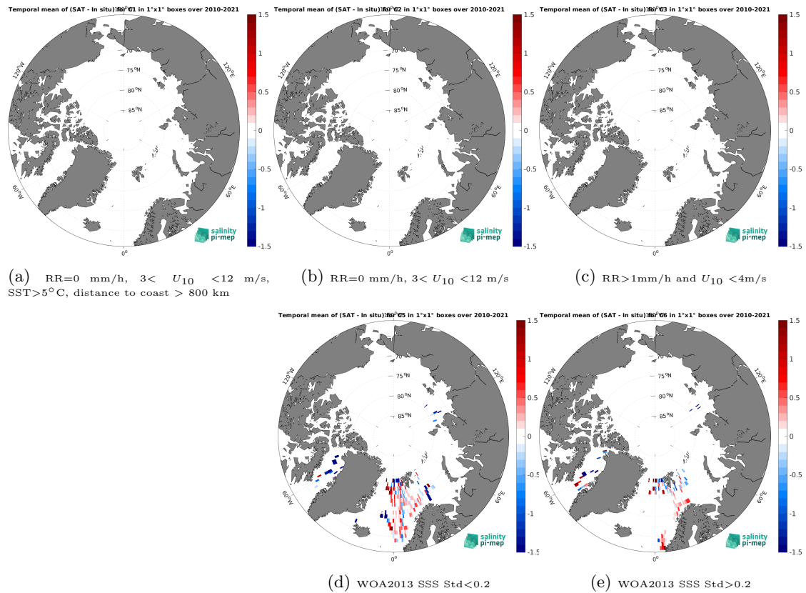
Figure 12: Temporal mean gridded over spatial boxes of size 1^{\circ}\times 1^{\circ} of \Delta\text{SSS} (SMOS SSS L3 v335 - Monthly - 25 km (CATDS-CPDC) - TSG (Polarstern)) for 5 different subdatasets corresponding to: RR=0 mm/h, 3 < U_{10} < 12 m/s, SST > 5^{\circ}\text{C} , distance to coast > 800 km (a), RR=0 mm/h, 3 < U_{10} < 12 m/s (b), RR > 1 mm/h and U_{10} < 4 m/s (c), WOA2013 SSS Std < 0.2 (d), WOA2013 SSS Std > 0.2 (e).
