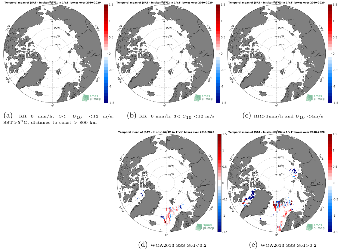
Figure 12: Temporal mean gridded over spatial boxes of size 1^{\circ} \times 1^{\circ} of \Delta\text{SSS} (SMOS SSS L3 v335 - Monthly - 25 km (CATDS-CPDC) - TSG (Polarstern)) for 5 different subdatasets corresponding to: RR=0 mm/h, 3 < U_{10} < 12 m/s, SST >5^{\circ}\text{C} , distance to coast > 800 km (a), RR=0 mm/h, 3 < U_{10} < 12 m/s (b), RR >1 mm/h and U_{10} < 4 m/s (c), WOA2013 SSS Std <0.2 (d), WOA2013 SSS Std >0.2 (e).
