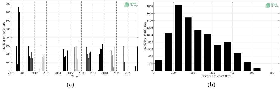
Figure 1: Number of match-ups between TSG (Polarstern) and SMOS SSS L3 v335 - Monthly - 25 km (CATDS-CPDC) SSS as a function of time (a) and as function of the distance to coast (b) over the Arctic Ocean Pi-MEP region and for the full satellite product period.
