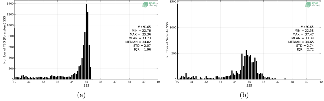
Figure 2: Histograms of SSS from TSG (Polarstern) (a) and SMOS SSS L3 v335 - Monthly - 25 km (CATDS-CPDC) (b) considering all match-up pairs per bins of 0.1 over the Arctic Ocean Pi-MEP region and for the full satellite product period.
