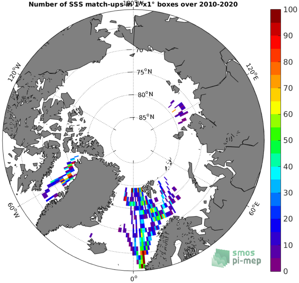
Figure 4: Number of SSS match-ups between TSG (Polarstern) SSS and the SMOS SSS L3 v335 - Monthly - 25 km (CATDS-CPDC) SSS product for the Arctic Ocean Pi-MEP region over 1^\circ \times 1^\circ boxes and for the full satellite product period.
