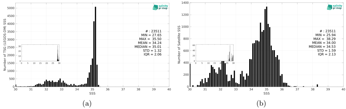
Figure 3: Histograms of SSS from TSG (LEGOS-DM) (a) and SMOS SSS L3 v335 - Monthly - 25 km (CATDS-CPDC) (b) considering all match-up pairs per bins of 0.1 over the Arctic Ocean Pi-MEP region and for the full satellite product period.
