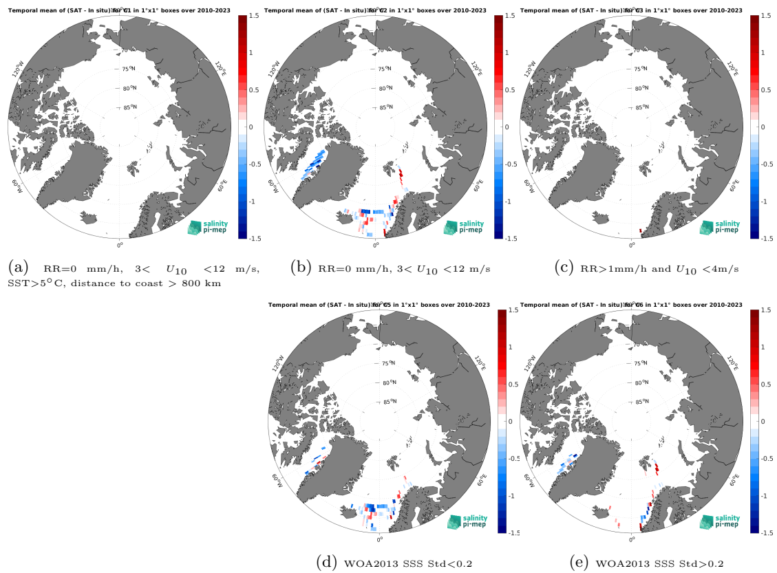
Figure 14: Temporal mean gridded over spatial boxes of size 1^\circ \times 1^\circ of \Delta SSS (SMOS SSS L3 v335 - Monthly - 25 km (CATDS-CPDC) - TSG (LEGOS-DM)) for 5 different subdatasets corresponding to: RR=0 mm/h, 3 < U_{10} < 12 m/s, SST > 5°C, distance to coast > 800 km (a), RR=0 mm/h, 3 < U_{10} < 12 m/s (b), RR > 1mm/h and U_{10} < 4 m/s (c), WOA2013 SSS Std < 0.2 (d), WOA2013 SSS Std > 0.2 (e).
