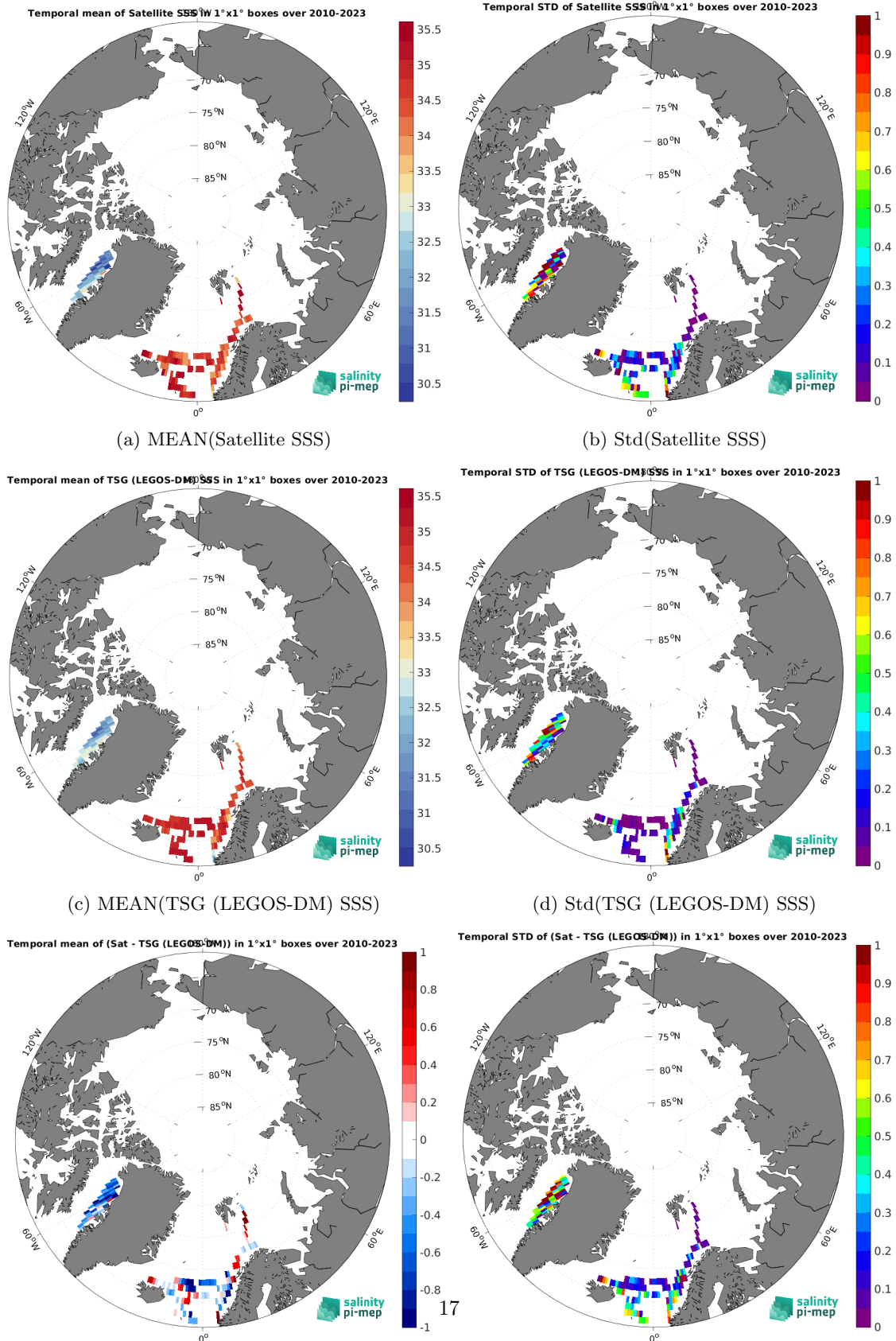
(e) MEAN( \Delta SSS) (Satellite - TSG (LEGOS-DM)) (f) Std( \Delta SSS) (Satellite - TSG (LEGOS-DM)) Figure 7: Temporal mean (left) and Std (right) of SSS from SMOS SSS L3 v335 - Monthly - 25 km (CATDS-CPDC) (top), TSG (LEGOS-DM) (middle), and of \Delta SSS (Satellite - TSG (LEGOS-DM)). Only match-up pairs are used to generate these maps.
