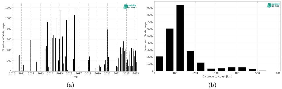
Figure 2: Number of match-ups between TSG (LEGOS-DM) and SMOS SSS L3 v335 - Monthly - 25 km (CATDS-CPDC) SSS as a function of time (a) and as function of the distance to coast (b) over the Arctic Ocean Pi-MEP region and for the full satellite product period.
