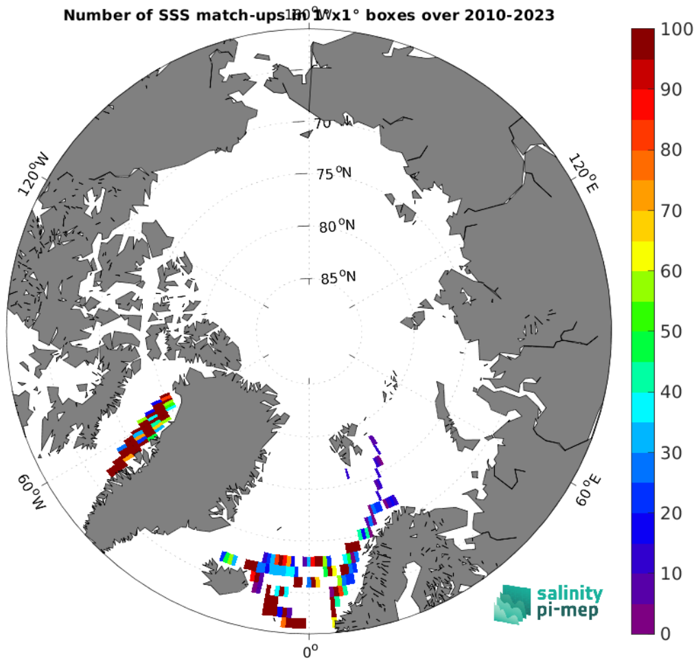
Figure 5: Number of SSS match-ups between TSG (LEGOS-DM) SSS and the SMOS SSS L3 v335 - Monthly - 25 km (CATDS-CPDC) SSS product for the Arctic Ocean Pi-MEP region over 1^\circ \times 1^\circ boxes and for the full satellite product period.
