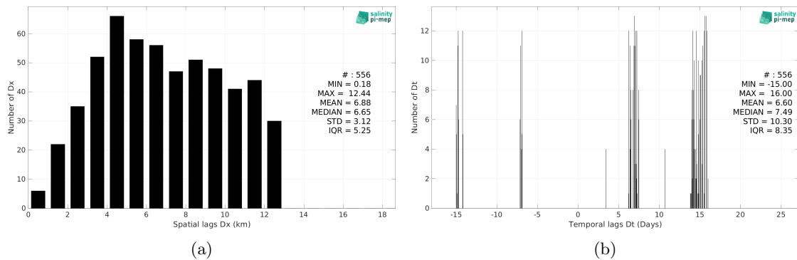
Figure 6: Histograms of the spatial (a) and temporal (b) lags between the location/time of the TSG (Lauge-Koch) measurement and the date of the corresponding SMOS SSS L3 v335 - Monthly - 25 km (CATDS-CPDC) SSS pixel.
