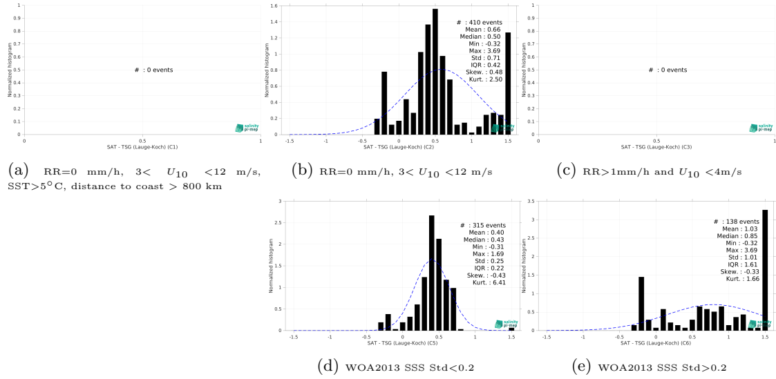
Figure 15: Normalized histogram of \Delta SSS (SMOS SSS L3 v335 - Monthly - 25 km (CATDS-CPDC) - TSG (Lauge-Koch)) for 5 different subdatasets corresponding to: RR=0 mm/h, 3 < U_{10} < 12 m/s, SST > 5°C, distance to coast > 800 km (a), RR=0 mm/h, 3 < U_{10} < 12 m/s (b), RR > 1mm/h and U_{10} < 4 m/s (c), WOA2013 SSS Std < 0.2 (d), WOA2013 SSS Std > 0.2 (e).
