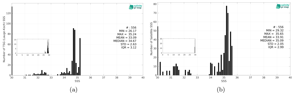
Figure 3: Histograms of SSS from TSG (Lauge-Koch) (a) and SMOS SSS L3 v335 - Monthly - 25 km (CATDS-CPDC) (b) considering all match-up pairs per bins of 0.1 over the Arctic Ocean Pi-MEP region and for the full satellite product period.
