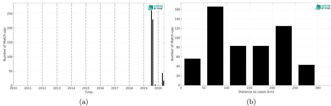
Figure 2: Number of match-ups between TSG (Lauge-Koch) and SMOS SSS L3 v335 - Monthly - 25 km (CATDS-CPDC) SSS as a function of time (a) and as function of the distance to coast (b) over the Arctic Ocean Pi-MEP region and for the full satellite product period.
