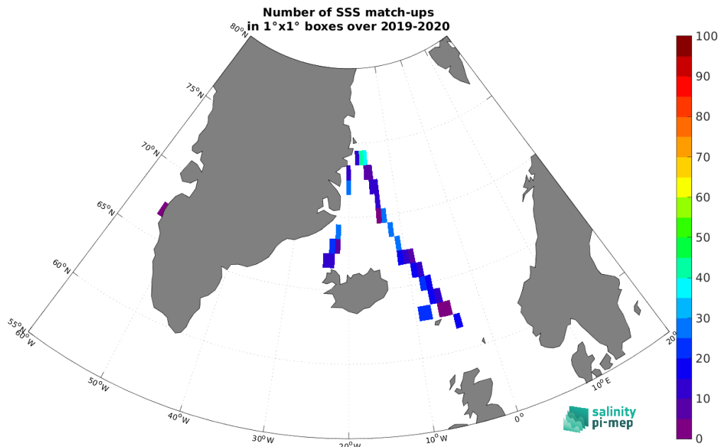
Figure 4: Number of SSS match-ups between TSG (Lauge-Koch) SSS and the SMOS SSS L3 v335 - Monthly - 25 km (CATDS-CPDC) SSS product for the Arctic Ocean Pi-MEP region over 1^\circ \times 1^\circ boxes and for the full satellite product period.
