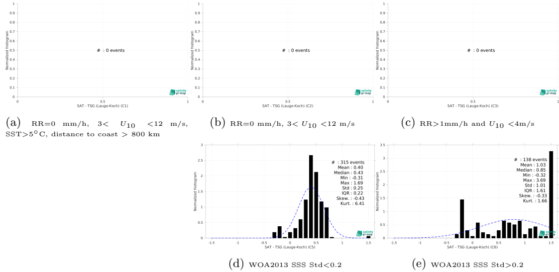
Figure 13: Normalized histogram of \Delta SSS (SMOS SSS L3 v335 - Monthly - 25 km (CATDS-CPDC) - TSG (Laue-Koch)) for 5 different subdatasets corresponding to: RR=0 mm/h, 3 < U_{10} < 12 m/s, SST>5°C, distance to coast > 800 km (a), RR=0 mm/h, 3 < U_{10} < 12 m/s (b), RR>1mm/h and U_{10} < 4 m/s (c), WOA2013 SSS Std<0.2 (d), WOA2013 SSS Std>0.2 (e).
