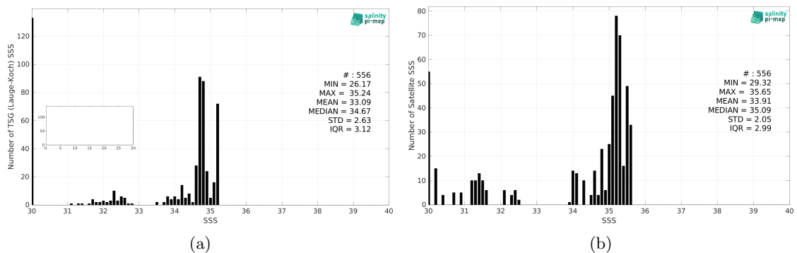
Figure 2: Histograms of SSS from TSG (Lauge-Koch) (a) and SMOS SSS L3 v335 - Monthly - 25 km (CATDS-CPDC) (b) considering all match-up pairs per bins of 0.1 over the Arctic Ocean Pi-MEP region and for the full satellite product period.
