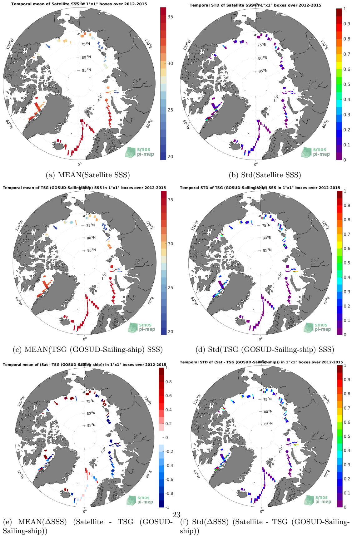
Figure 6: Temporal mean (left) and Std (right) of SSS from SMOS SSS L3 v335 - Monthly - 25 km (CATDS-CPDC) (top), TSG (GOSUD-Sailing-ship) (middle), and of \Delta SSS (Satellite - TSG (GOSUD-Sailing-ship)). Only match-up pairs are used to generate these maps.
