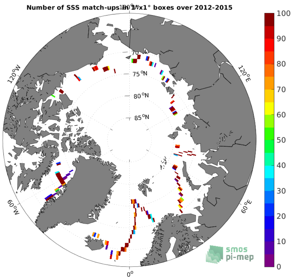
Figure 4: Number of SSS match-ups between TSG (GOSUD-Sailing-ship) SSS and the SMOS SSS L3 v335 - Monthly - 25 km (CATDS-CPDC) SSS product for the Arctic Ocean Pi-MEP region over 1^{\circ} \times 1^{\circ} boxes and for the full satellite product period.
