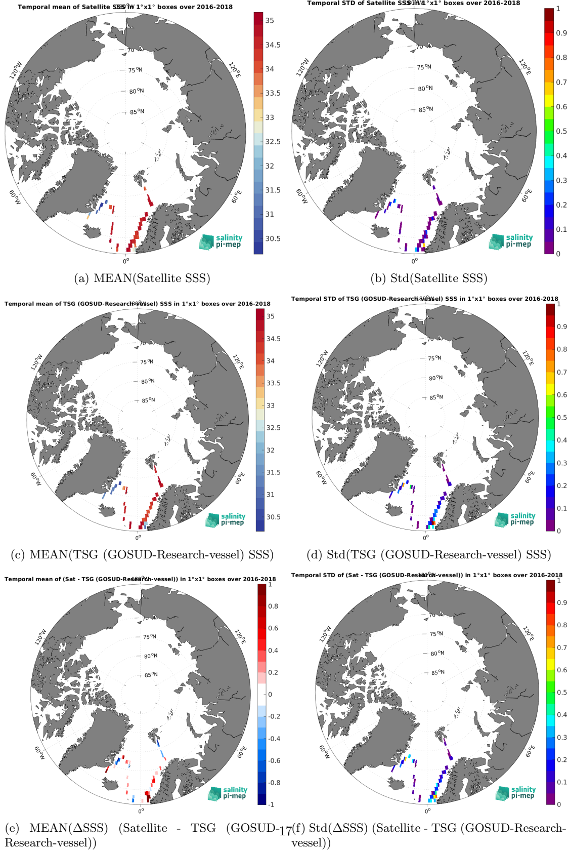
Figure 7: Temporal mean (left) and Std (right) of SSS from SMOS SSS L3 v335 - Monthly - 25 km (CATDS-CPDC) (top), TSG (GOSUD-Research-vessel) (middle), and of \Delta SSS (Satellite - TSG (GOSUD-Research-vessel)). Only match-up pairs are used to generate these maps.
