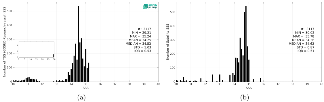
Figure 3: Histograms of SSS from TSG (GOSUD-Research-vessel) (a) and SMOS SSS L3 v335 - Monthly - 25 km (CATDS-CPDC) (b) considering all match-up pairs per bins of 0.1 over the Arctic Ocean Pi-MEP region and for the full satellite product period.
