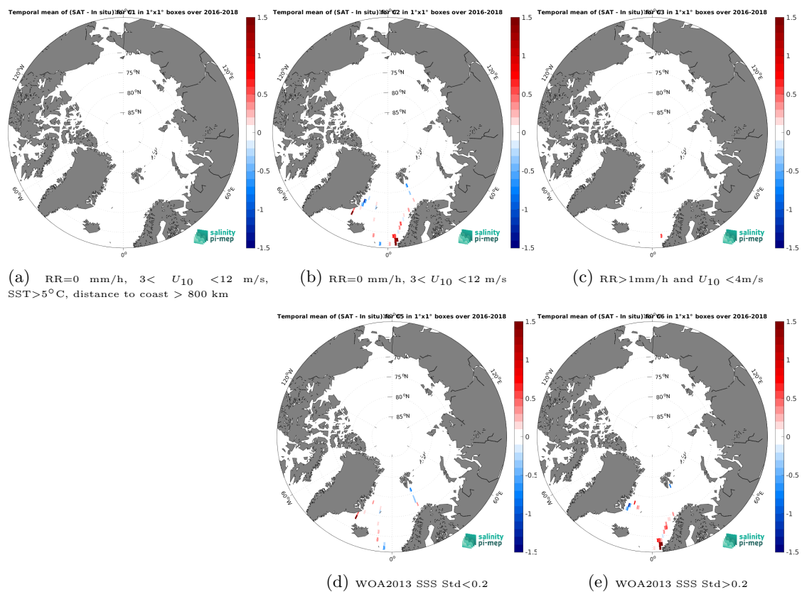
Figure 14: Temporal mean gridded over spatial boxes of size 1^\circ \times 1^\circ of \Delta SSS (SMOS SSS L3 v335 - Monthly - 25 km (CATDS-CPDC) - TSG (GOSUD-Research-vessel)) for 5 different subdatasets corresponding to: RR=0 mm/h, 3 < U_{10} < 12 m/s, SST > 5°C, distance to coast > 800 km (a), RR=0 mm/h, 3 < U_{10} < 12 m/s (b), RR > 1mm/h and U_{10} < 4 m/s (c), WOA2013 SSS Std < 0.2 (d), WOA2013 SSS Std > 0.2 (e).
