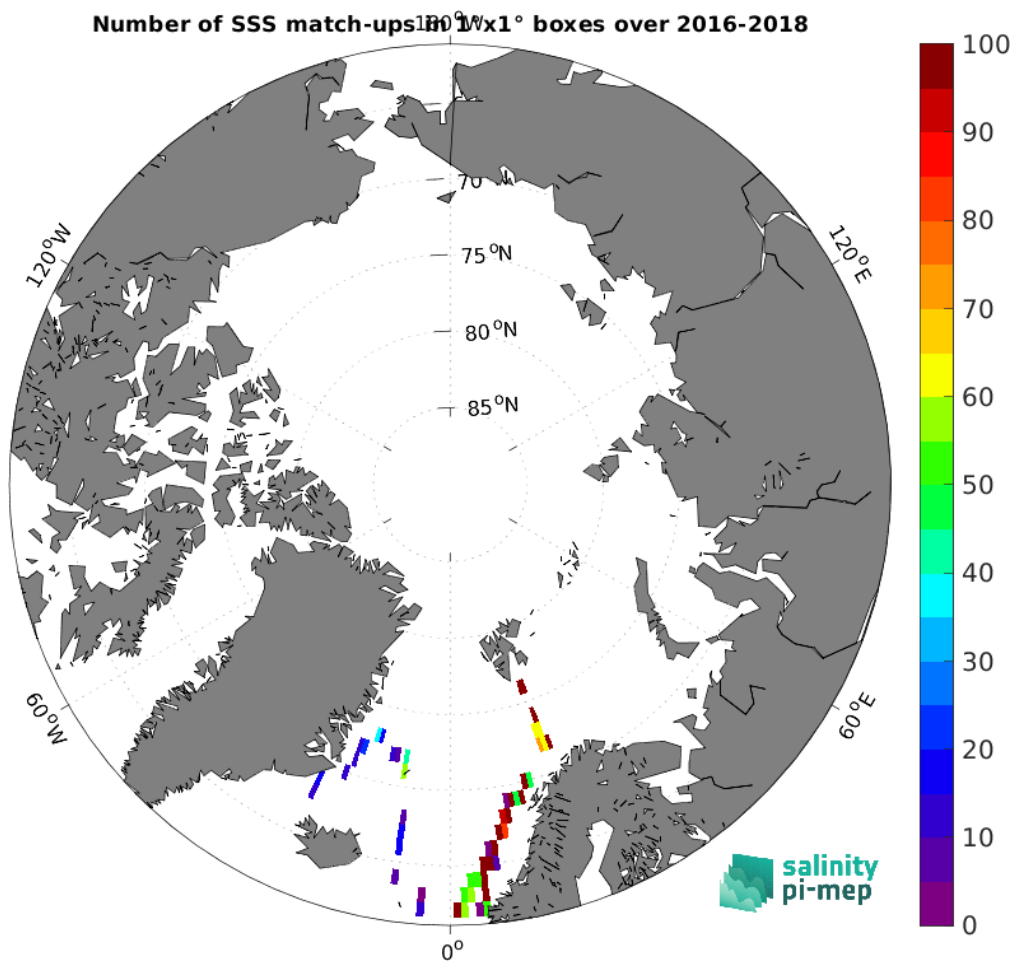
Figure 5: Number of SSS match-ups between TSG (GOSUD-Research-vessel) SSS and the SMOS SSS L3 v335 - Monthly - 25 km (CATDS-CPDC) SSS product for the Arctic Ocean Pi-MEP region over 1^{\circ} \times 1^{\circ} boxes and for the full satellite product period.
