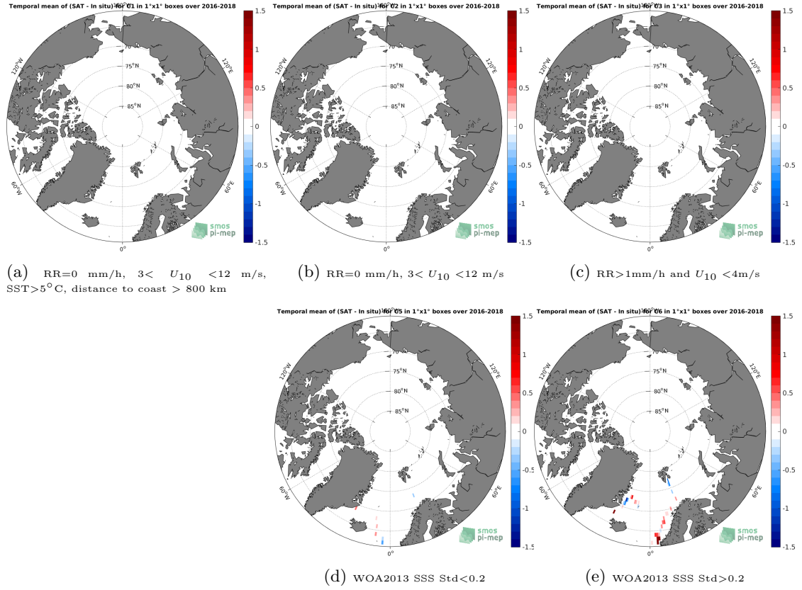
Figure 12: Temporal mean gridded over spatial boxes of size 1^\circ \times 1^\circ of \Delta\text{SSS} (SMOS SSS L3 v335 - Monthly - 25 km (CATDS-CPDC) - TSG (GOSUD-Research-vessel)) for 5 different subdatasets corresponding to: RR=0 mm/h, 3 < U_{10} < 12 m/s, SST > 5^\circ\text{C} , distance to coast > 800 km (a), RR=0 mm/h, 3 < U_{10} < 12 m/s (b), RR > 1\text{mm/h} and U_{10} < 4\text{m/s} (c), WOA2013 SSS Std < 0.2 (d), WOA2013 SSS Std > 0.2 (e).
