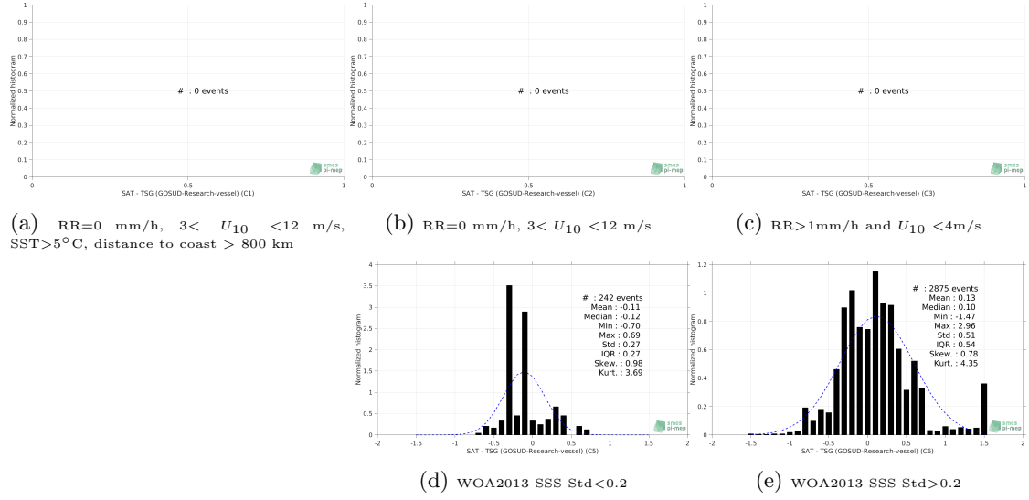
Figure 13: Normalized histogram of \Delta\text{SSS} (SMOS SSS L3 v335 - Monthly - 25 km (CATDS-CPDC) - TSG (GOSUD-Research-vessel)) for 5 different subdatasets corresponding to: RR=0 mm/h, 3 < U_{10} < 12 m/s, SST > 5^\circ\text{C} , distance to coast > 800 km (a), RR=0 mm/h, 3 < U_{10} < 12 m/s (b), RR > 1 mm/h and U_{10} < 4 m/s (c), WOA2013 SSS Std < 0.2 (d), WOA2013 SSS Std > 0.2 (e).
