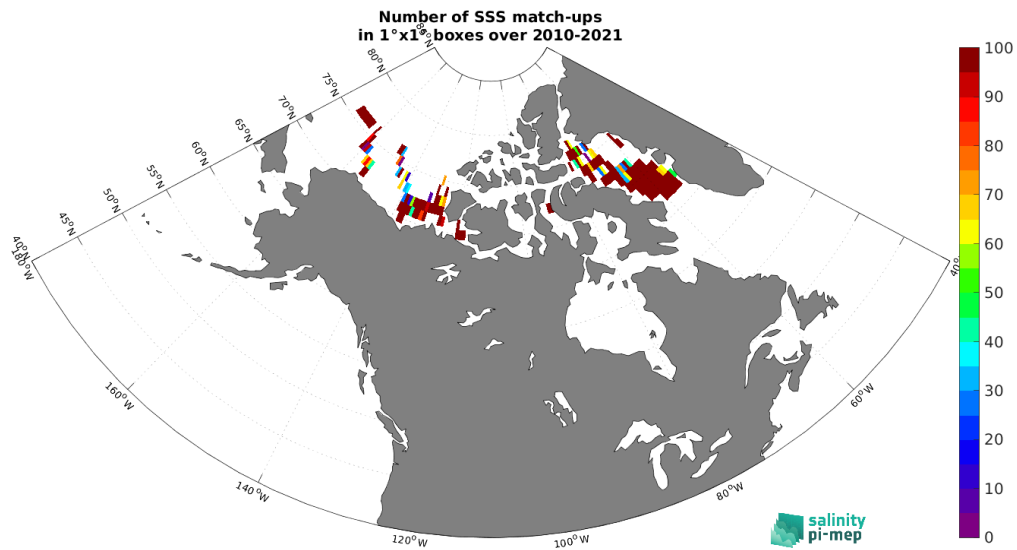
Figure 5: Number of SSS match-ups between TSG (Amundsen) SSS and the SMOS SSS L3 v335 - Monthly - 25 km (CATDS-CPDC) SSS product for the Arctic Ocean Pi-MEP region over 1^\circ \times 1^\circ boxes and for the full satellite product period.
