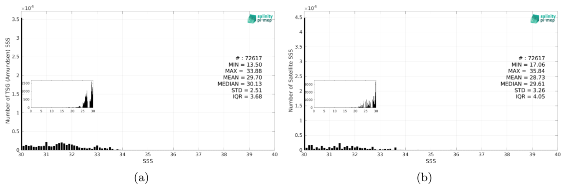
Figure 3: Histograms of SSS from TSG (Amundsen) (a) and SMOS SSS L3 v335 - Monthly - 25 km (CATDS-CPDC) (b) considering all match-up pairs per bins of 0.1 over the Arctic Ocean Pi-MEP region and for the full satellite product period.
