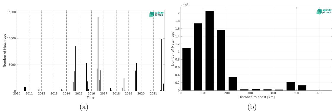
Figure 2: Number of match-ups between TSG (Amundsen) and SMOS SSS L3 v335 - Monthly - 25 km (CATDS-CPDC) SSS as a function of time (a) and as function of the distance to coast (b) over the Arctic Ocean Pi-MEP region and for the full satellite product period.
