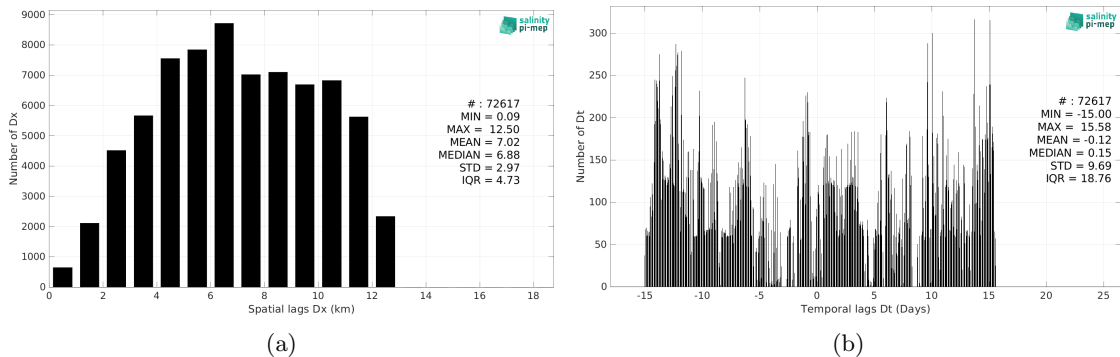
Figure 6: Histograms of the spatial (a) and temporal (b) lags between the location/time of the TSG (Amundsen) measurement and the date of the corresponding SMOS SSS L3 v335 - Monthly - 25 km (CATDS-CPDC) SSS pixel.
