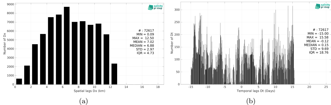
Figure 5: Histograms of the spatial (a) and temporal (b) lags between the location/time of the TSG (Amundsen) measurement and the date of the corresponding SMOS SSS L3 v335 - Monthly - 25 km (CATDS-CPDC) SSS pixel.
