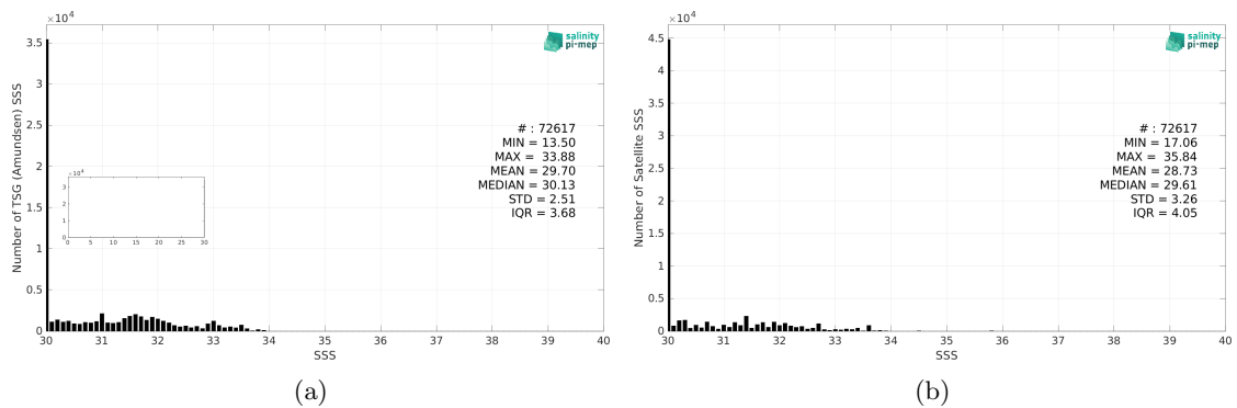
Figure 2: Histograms of SSS from TSG (Amundsen) (a) and SMOS SSS L3 v335 - Monthly - 25 km (CATDS-CPDC) (b) considering all match-up pairs per bins of 0.1 over the Arctic Ocean Pi-MEP region and for the full satellite product period.
