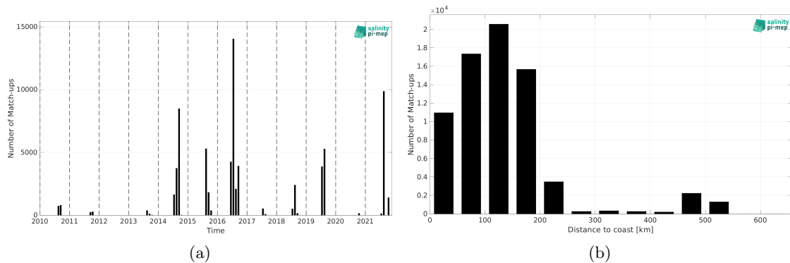
Figure 1: Number of match-ups between TSG (Amundsen) and SMOS SSS L3 v335 - Monthly - 25 km (CATDS-CPDC) SSS as a function of time (a) and as function of the distance to coast (b) over the Arctic Ocean Pi-MEP region and for the full satellite product period.
