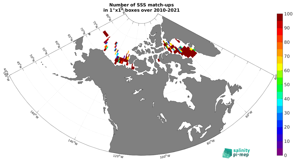
Figure 4: Number of SSS match-ups between TSG (Amundsen) SSS and the SMOS SSS L3 v335 - Monthly - 25 km (CATDS-CPDC) SSS product for the Arctic Ocean Pi-MEP region over 1^\circ \times 1^\circ boxes and for the full satellite product period.
