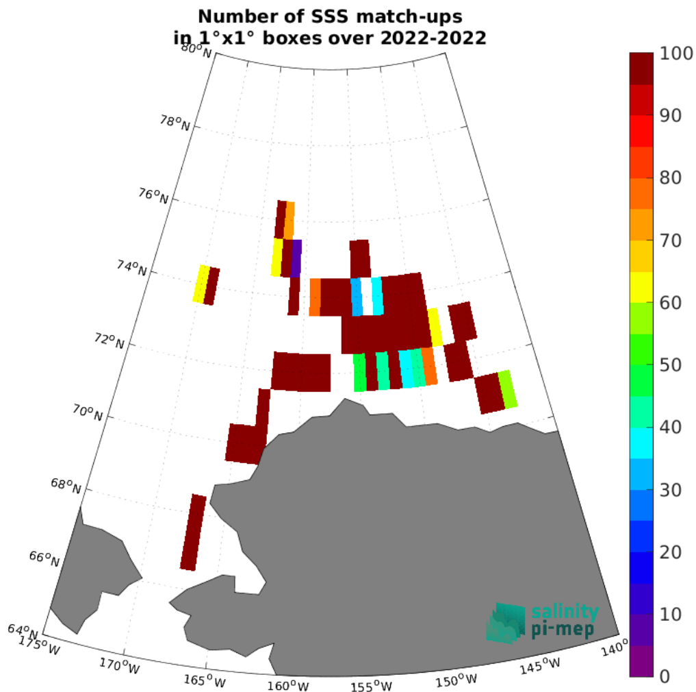
Figure 5: Number of SSS match-ups between SASSIE SSS and the SMOS SSS L3 v335 - Monthly - 25 km (CATDS-CPDC) SSS product for the Arctic Ocean Pi-MEP region over 1^\circ \times 1^\circ boxes and for the full satellite product period.
