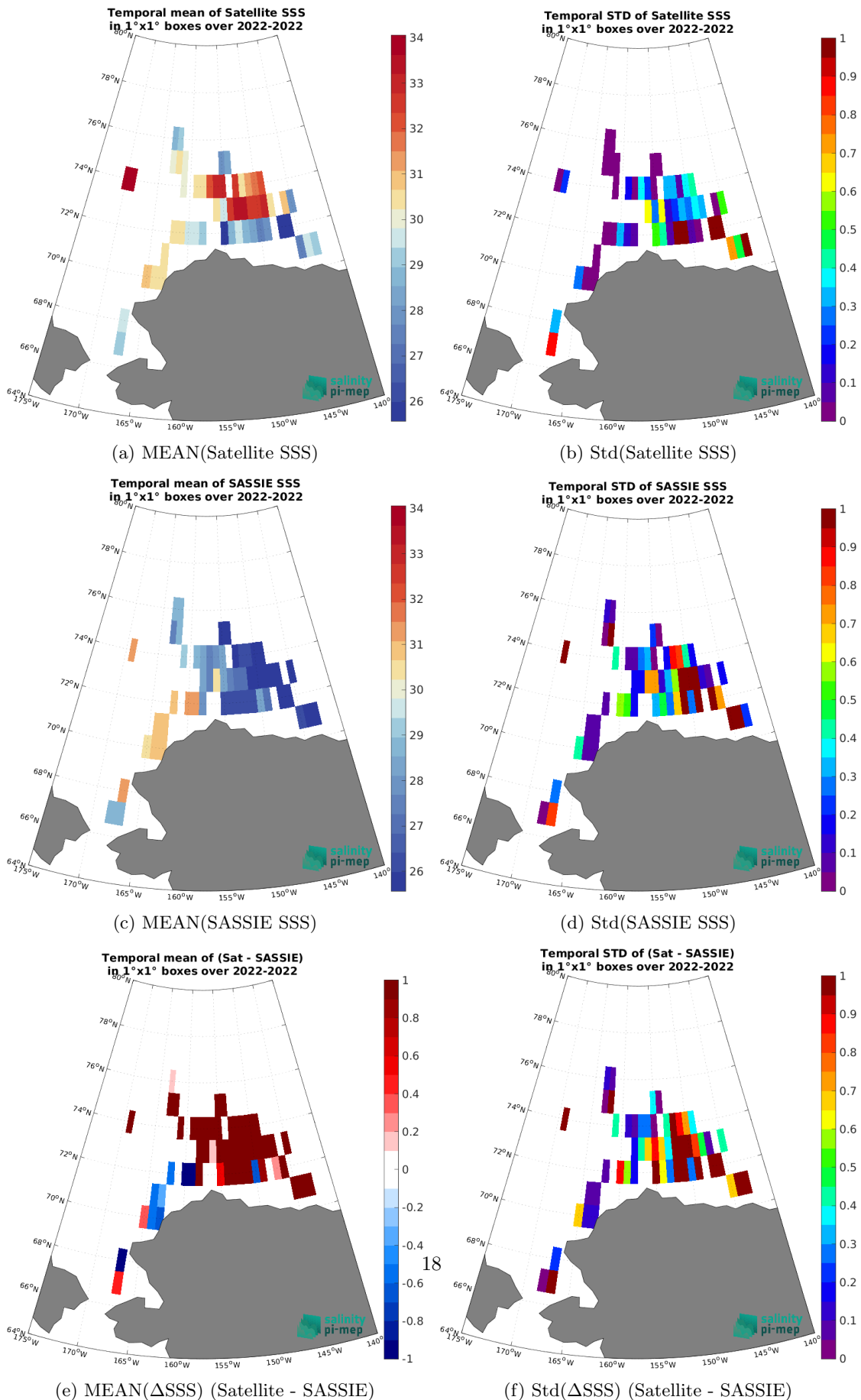
Figure 7: Temporal mean (left) and Std (right) of SSS from SMOS SSS L3 v335 - Monthly - 25 km (CATDS-CPDC) (top), SASSIE (middle), and of \Delta SSS (Satellite - SASSIE). Only match-up pairs are used to generate these maps.
