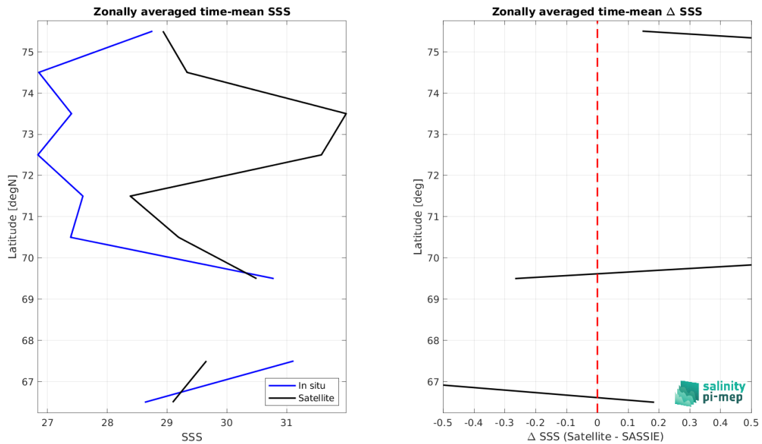
Figure 9: Left panel: Zonal mean SSS from SMOS SSS L3 v335 - Monthly - 25 km (CATDS-CPDC) satellite product (black) and from SASSIE (blue). Right panel: Zonal mean of \Delta SSS (Satellite - SASSIE) for all the collected Pi-MEP match-up pairs estimated over the full satellite product period.
