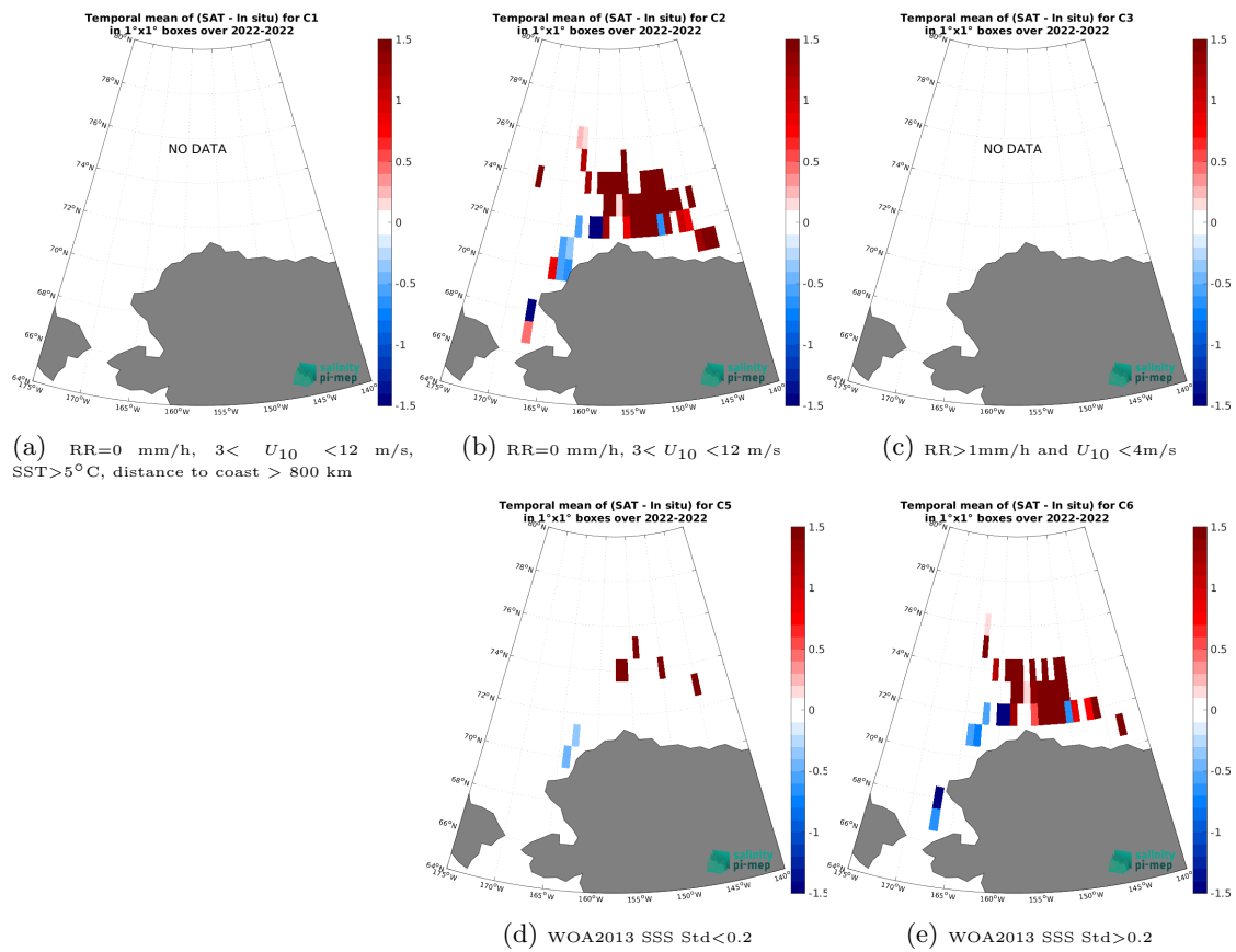
Figure 14: Temporal mean gridded over spatial boxes of size 1^\circ \times 1^\circ of \Delta SSS (SMOS SSS L3 v335 - Monthly - 25 km (CATDS-CPDC) - SASSIE) for 5 different subdatasets corresponding to:RR=0 mm/h, 3 < U_{10} < 12 m/s, SST >5^\circ\text{C} , distance to coast > 800 km (a), RR=0 mm/h, 3 < U_{10} < 12 m/s (b), RR >1 mm/h and U_{10} < 4 m/s (c), WOA2013 SSS Std <0.2 (d), WOA2013 SSS Std >0.2 (e).
