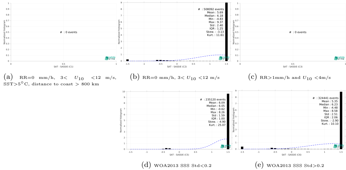
Figure 15: Normalized histogram of \Delta SSS (SMOS SSS L3 v335 - Monthly - 25 km (CATDS-CPDC) - SASSIE) for 5 different subdatasets corresponding to: RR=0 mm/h, 3 < U_{10} < 12 m/s, SST>5°C, distance to coast > 800 km (a), RR=0 mm/h, 3 < U_{10} < 12 m/s (b), RR>1mm/h and U_{10} < 4 m/s (c), WOA2013 SSS Std<0.2 (d), WOA2013 SSS Std>0.2 (e).
