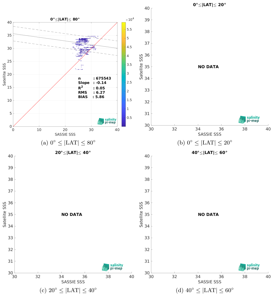
Figure 10: Contour maps of the concentration of SMOS SSS L3 v335 - Monthly - 25 km (CATDS-CPDC) SSS (y-axis) versus SASSIE SSS (x-axis) at match-up pairs for different latitude bands. For each plot, the red line shows x=y . The black thin and dashed lines indicate a linear fit through the data cloud and the \pm 95\% confidence levels, respectively. The number match-up pairs n , the slope and R^2 coefficient of the linear fit, the root mean square (RMS) and the mean bias between satellite and in situ data are indicated for each latitude band in each plots.
