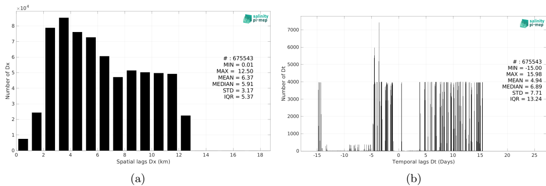
Figure 6: Histograms of the spatial (a) and temporal (b) lags between the location/time of the SASSIE measurement and the date of the corresponding SMOS SSS L3 v335 - Monthly - 25 km (CATDS-CPDC) SSS pixel.
