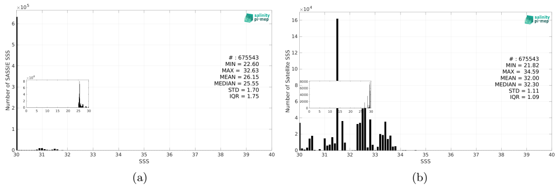
Figure 3: Histograms of SSS from SASSIE (a) and SMOS SSS L3 v335 - Monthly - 25 km (CATDS-CPDC) (b) considering all match-up pairs per bins of 0.1 over the Arctic Ocean Pi-MEP region and for the full satellite product period.
