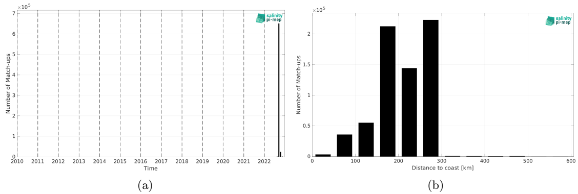
Figure 2: Number of match-ups between SASSIE and SMOS SSS L3 v335 - Monthly - 25 km (CATDS-CPDC) SSS as a function of time (a) and as function of the distance to coast (b) over the Arctic Ocean Pi-MEP region and for the full satellite product period.
