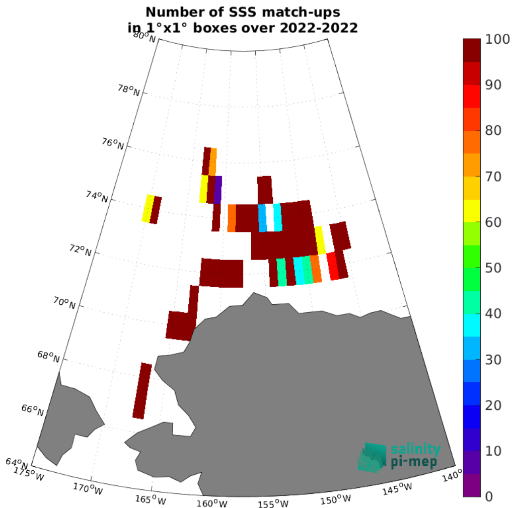
Figure 5: Number of SSS match-ups between SASSIE SSS and the SMOS SSS L3 v335 - Monthly - 25 km (CATDS-CPDC) SSS product for the Arctic Ocean Pi-MEP region over 1°x1° boxes and for the full satellite product period.
