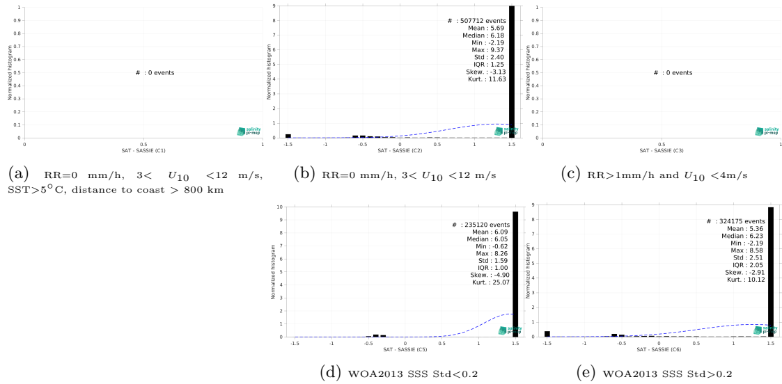
Figure 15: Normalized histogram of \Delta SSS (SMOS SSS L3 v335 - Monthly - 25 km (CATDS-CPDC) - SASSIE) for 5 different subdatasets corresponding to: RR=0 mm/h, 3 < U_{10} < 12 m/s, SST > 5°C, distance to coast > 800 km (a), RR=0 mm/h, 3 < U_{10} < 12 m/s (b), RR > 1mm/h and U_{10} < 4 m/s (c), WOA2013 SSS Std < 0.2 (d), WOA2013 SSS Std > 0.2 (e).
