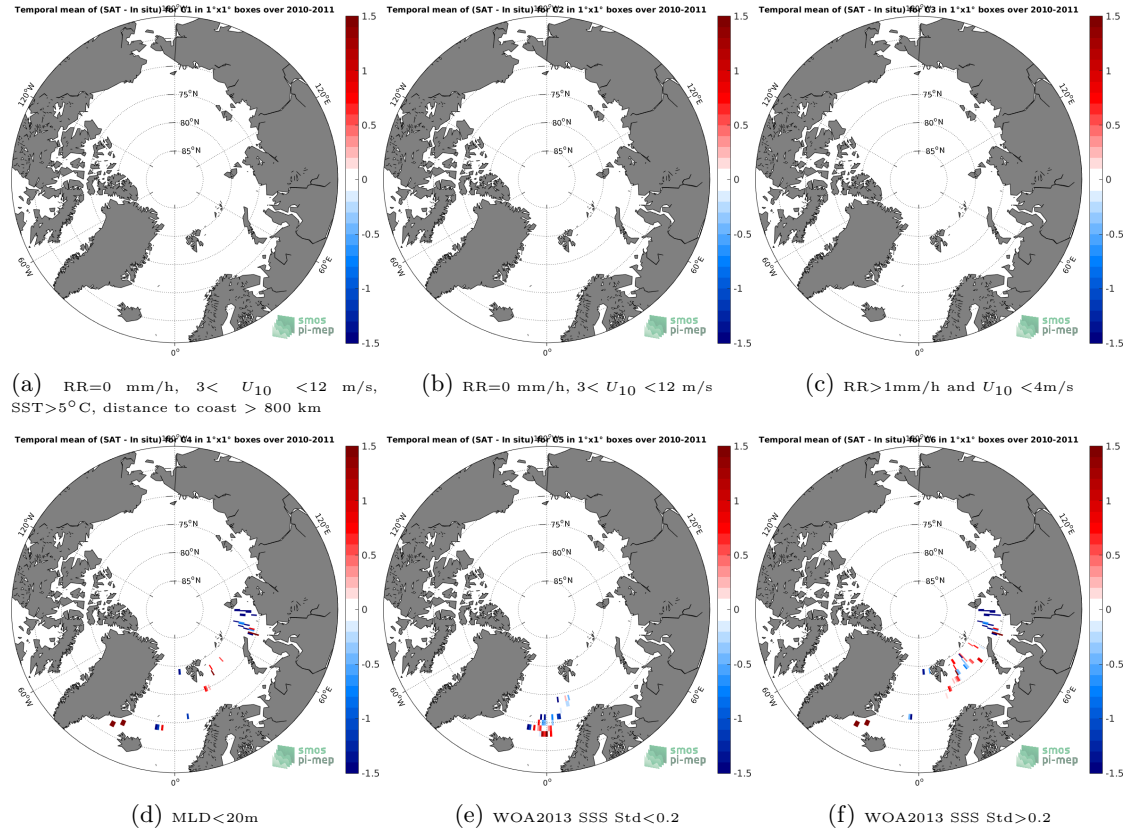
Figure 12: Temporal mean gridded over spatial boxes of size 1^{\circ} \times 1^{\circ} of \Delta\text{SSS} (SMOS SSS L3 v335 - Monthly - 25 km (CATDS-CPDC) - Marine mammals) for 6 different subdatasets corresponding to: RR=0 mm/h, 3 < U_{10} < 12 m/s, SST >5^{\circ}\text{C} , distance to coast > 800 km (a), RR=0 mm/h, 3 < U_{10} < 12 m/s (b), RR >1 mm/h and U_{10} < 4 m/s (c),MLD <20 m (d),WOA2013 SSS Std <0.2 (e),WOA2013 SSS Std >0.2 (f).
