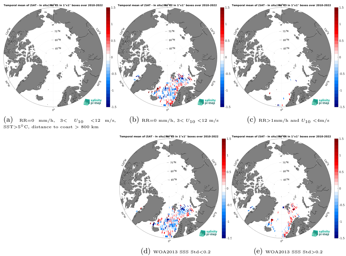
Figure 14: Temporal mean gridded over spatial boxes of size 1^\circ \times 1^\circ of \Delta SSS (SMOS SSS L3 v335 - Monthly - 25 km (CATDS-CPDC) - ICES) for 5 different subdatasets corresponding to: RR=0 mm/h, 3 < U_{10} < 12 m/s, SST > 5°C, distance to coast > 800 km (a), RR=0 mm/h, 3 < U_{10} < 12 m/s (b), RR > 1mm/h and U_{10} < 4 m/s (c), WOA2013 SSS Std < 0.2 (d), WOA2013 SSS Std > 0.2 (e).
