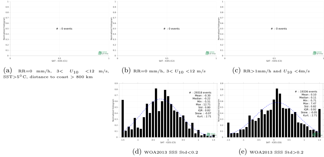
Figure 13: Normalized histogram of \Delta SSS (SMOS SSS L3 v335 - Monthly - 25 km (CATDS-CPDC) - ICES) for 5 different subdatasets corresponding to: RR=0 mm/h, 3 < U_{10} < 12 m/s, SST >5^{\circ}\text{C} , distance to coast > 800 km (a), RR=0 mm/h, 3 < U_{10} < 12 m/s (b), RR >1 mm/h and U_{10} < 4 m/s (c), WOA2013 SSS Std <0.2 (d), WOA2013 SSS Std >0.2 (e).
