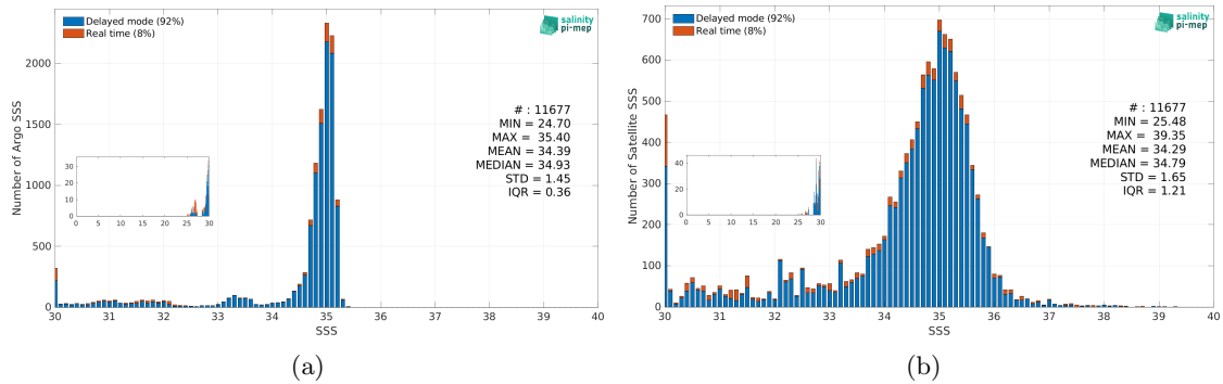
Figure 3: Histograms of SSS from Argo (a) and SMOS SSS L3 v335 - Monthly - 25 km (CATDS-CPDC) (b) considering all match-up pairs per bins of 0.1 over the Arctic Ocean Pi-MEP region and for the full satellite product period.
