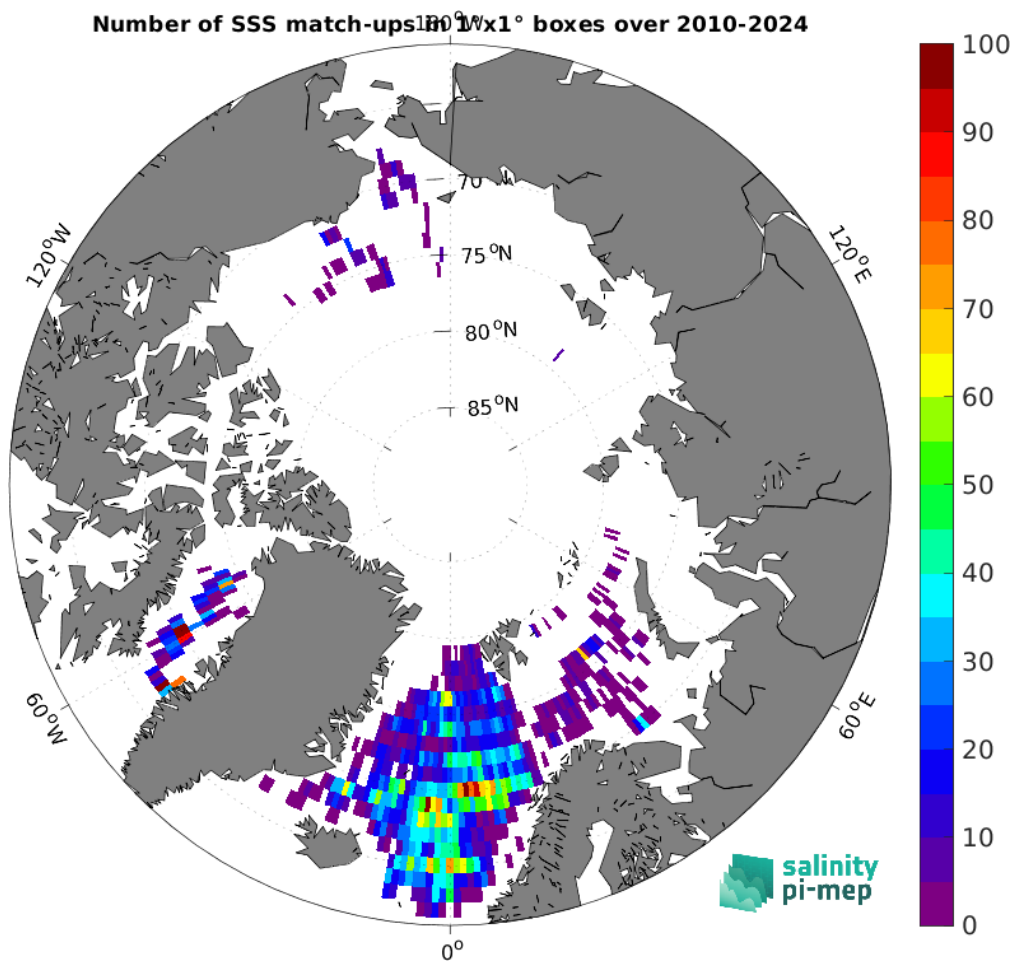
Figure 5: Number of SSS match-ups between Argo SSS and the SMOS SSS L3 v335 - Monthly - 25 km (CATDS-CPDC) SSS product for the Arctic Ocean Pi-MEP region over 1^\circ \times 1^\circ boxes and for the full satellite product period.
