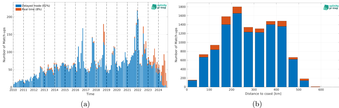
Figure 2: Number of match-ups between Argo and SMOS SSS L3 v335 - Monthly - 25 km (CATDS-CPDC) SSS as a function of time (a) and as function of the distance to coast (b) over the Arctic Ocean Pi-MEP region and for the full satellite product period.
