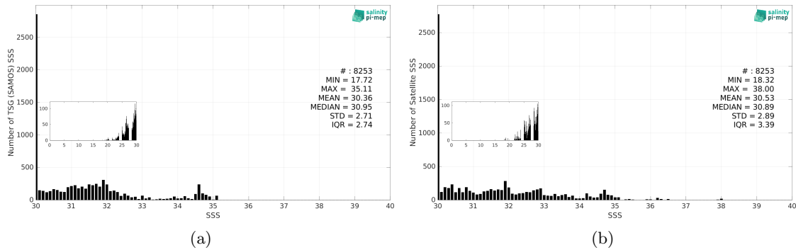
Figure 3: Histograms of SSS from TSG (SAMOS) (a) and SMOS SSS L3 v335 - 10 Days - 25 km (CATDS-CPDC) (b) considering all match-up pairs per bins of 0.1 over the Arctic Ocean Pi-MEP region and for the full satellite product period.
