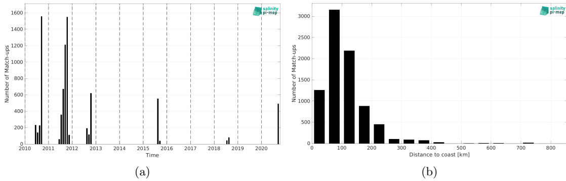
Figure 2: Number of match-ups between TSG (SAMOS) and SMOS SSS L3 v335 - 10 Days - 25 km (CATDS-CPDC) SSS as a function of time (a) and as function of the distance to coast (b) over the Arctic Ocean Pi-MEP region and for the full satellite product period.
