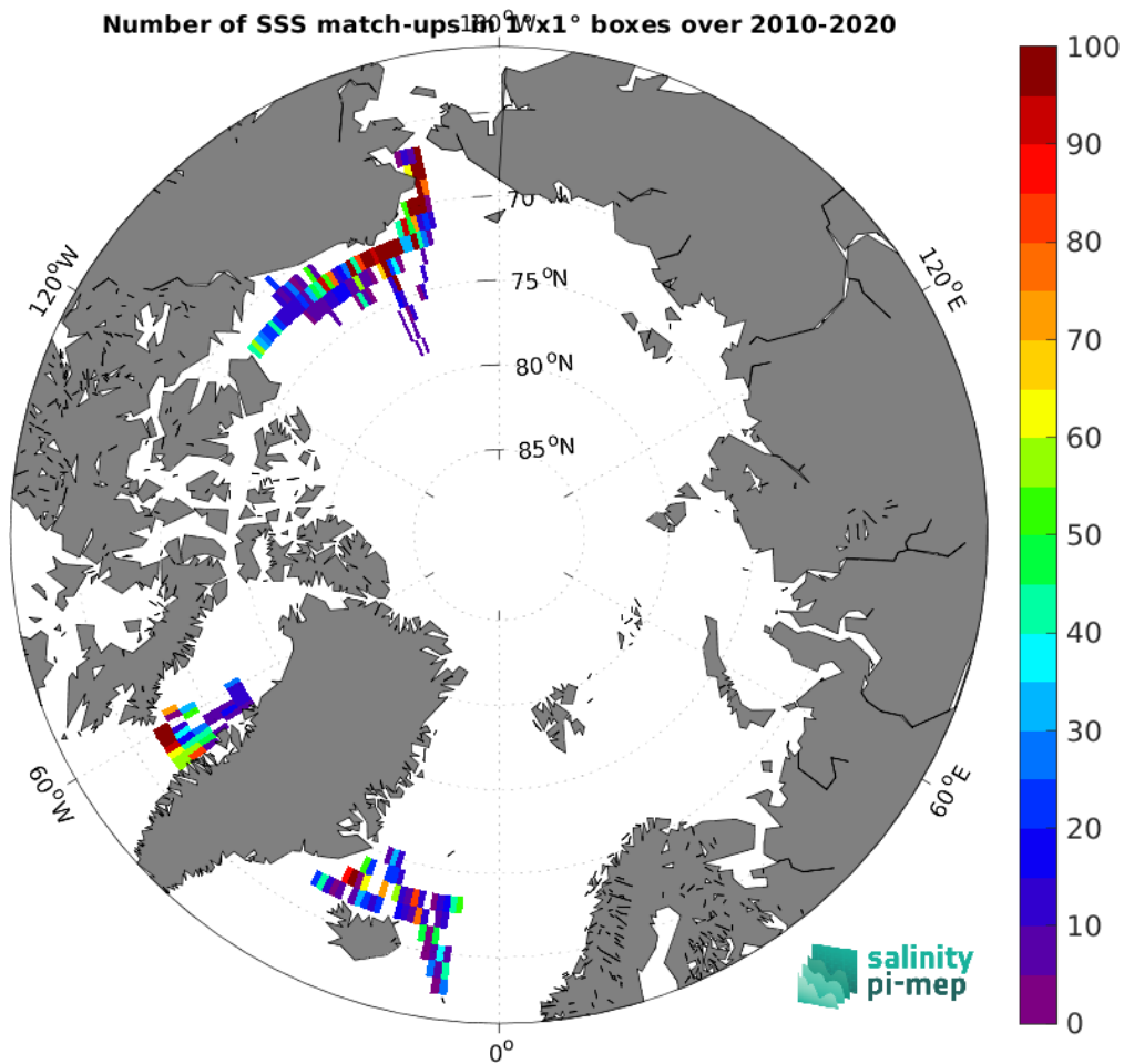
Figure 5: Number of SSS match-ups between TSG (SAMOS) SSS and the SMOS SSS L3 v335 - 10 Days - 25 km (CATDS-CPDC) SSS product for the Arctic Ocean Pi-MEP region over 1^\circ \times 1^\circ boxes and for the full satellite product period.
