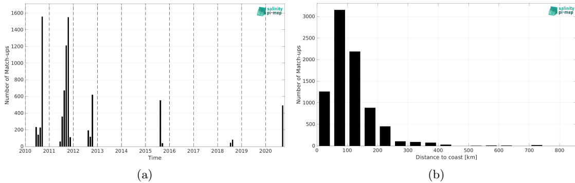
Figure 1: Number of match-ups between TSG (SAMOS) and SMOS SSS L3 v335 - 10 Days - 25 km (CATDS-CPDC) SSS as a function of time (a) and as function of the distance to coast (b) over the Arctic Ocean Pi-MEP region and for the full satellite product period.
