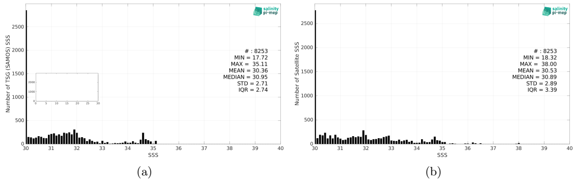
Figure 2: Histograms of SSS from TSG (SAMOS) (a) and SMOS SSS L3 v335 - 10 Days - 25 km (CATDS-CPDC) (b) considering all match-up pairs per bins of 0.1 over the Arctic Ocean Pi-MEP region and for the full satellite product period.
