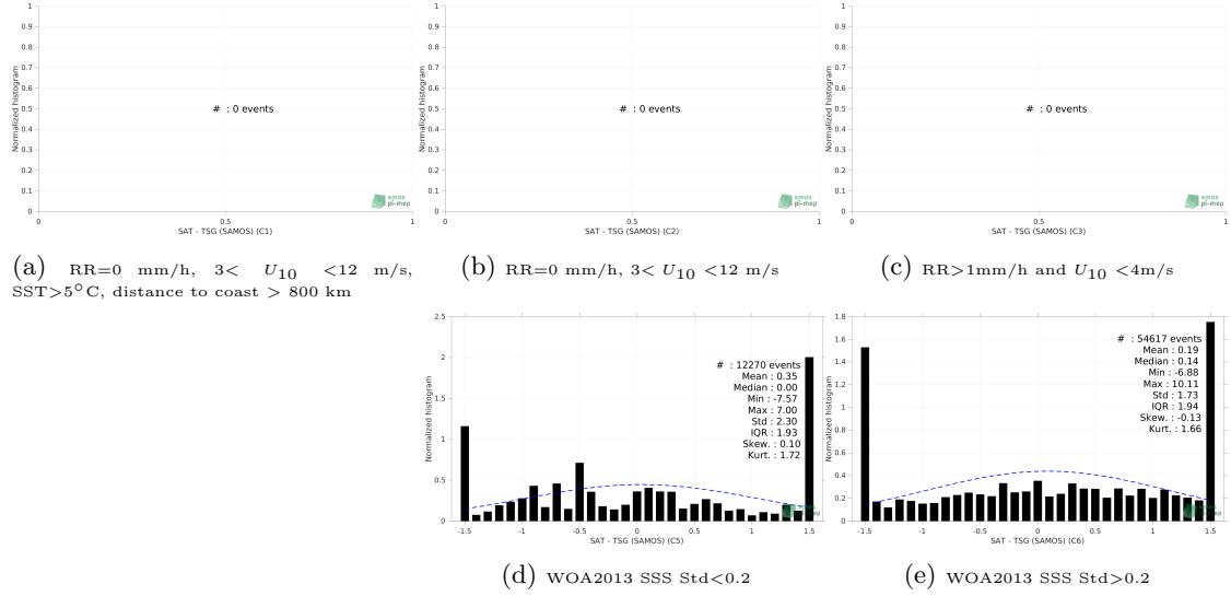
Figure 13: Normalized histogram of \Delta SSS (SMOS SSS L3 v335 - 10 Days - 25 km (CATDS-CPDC) - TSG (SAMOS)) for 5 different subdatasets corresponding to: RR=0 mm/h, 3 < U_{10} < 12 m/s, SST > 5°C, distance to coast > 800 km (a), RR=0 mm/h, 3 < U_{10} < 12 m/s (b), RR > 1mm/h and U_{10} < 4 m/s (c), WOA2013 SSS Std < 0.2 (d), WOA2013 SSS Std > 0.2 (e).
