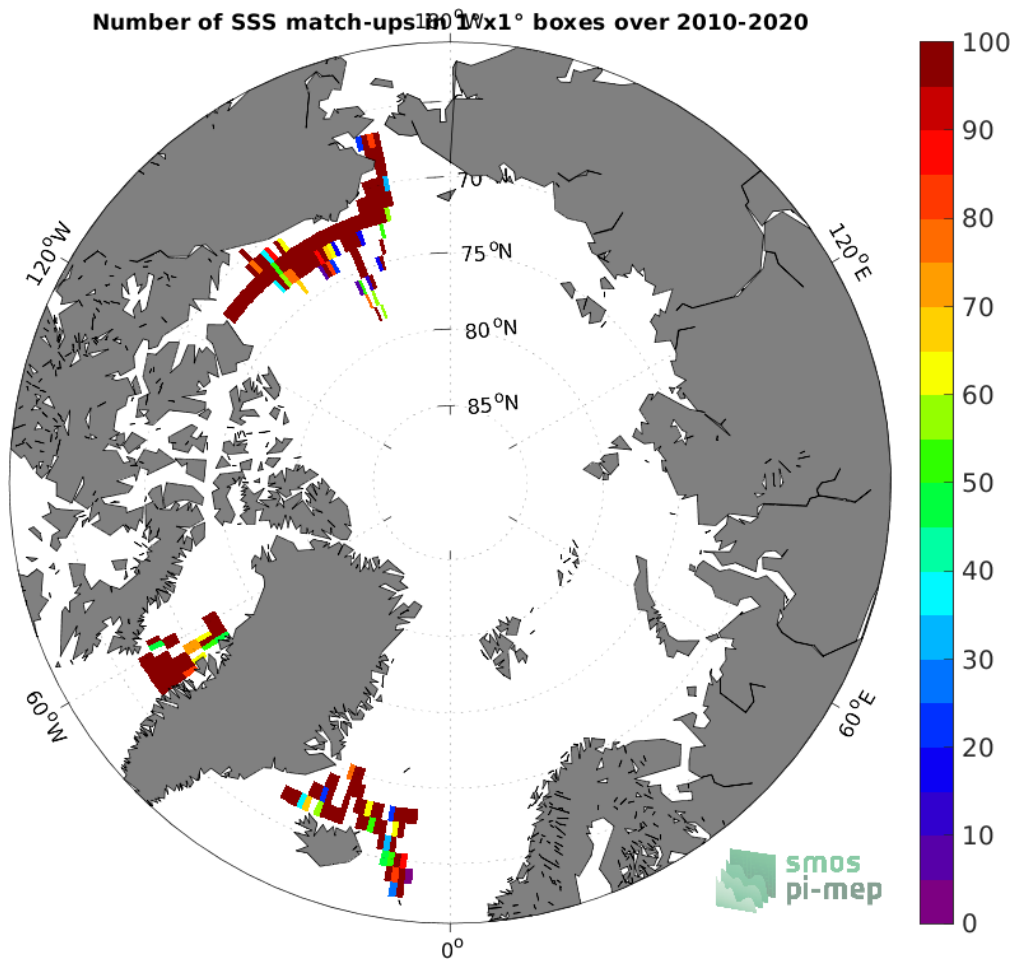
Figure 4: Number of SSS match-ups between TSG (SAMOS) SSS and the SMOS SSS L3 v335 - 10 Days - 25 km (CATDS-CPDC) SSS product for the Arctic Ocean Pi-MEP region over 1^{\circ} \times 1^{\circ} boxes and for the full satellite product period.
