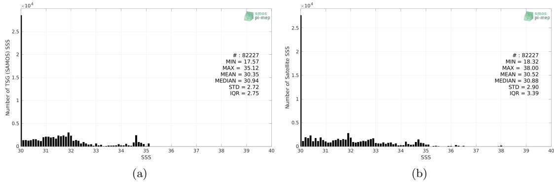
Figure 2: Histograms of SSS from TSG (SAMOS) (a) and SMOS SSS L3 v335 - 10 Days - 25 km (CATDS-CPDC) (b) considering all match-up pairs per bins of 0.1 over the Arctic Ocean Pi-MEP region and for the full satellite product period.
