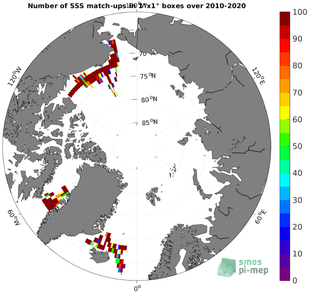
Figure 4: Number of SSS match-ups between TSG (SAMOS) SSS and the SMOS SSS L3 v335 - 10 Days - 25 km (CATDS-CPDC) SSS product for the Arctic Ocean Pi-MEP region over 1^\circ \times 1^\circ boxes and for the full satellite product period.
