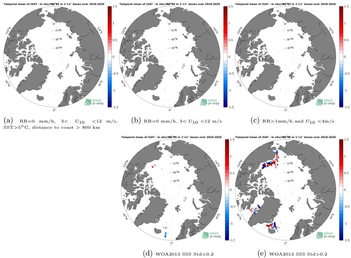
Figure 12: Temporal mean gridded over spatial boxes of size 1^{\circ}\times 1^{\circ} of \Delta\text{SSS} (SMOS SSS L3 v335 - 10 Days - 25 km (CATDS-CPDC) - TSG (SAMOS)) for 5 different subdatasets corresponding to:RR=0 mm/h, 3 < U_{10} < 12 m/s, SST >5^{\circ}\text{C} , distance to coast > 800 km (a), RR=0 mm/h, 3 < U_{10} < 12 m/s (b), RR >1 mm/h and U_{10} < 4 m/s (c), WOA2013 SSS Std <0.2 (d), WOA2013 SSS Std >0.2 (e).
