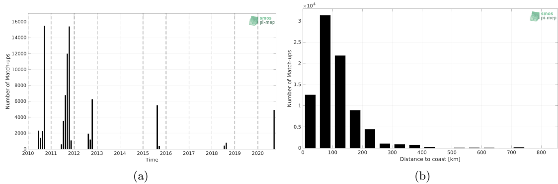
Figure 1: Number of match-ups between TSG (SAMOS) and SMOS SSS L3 v335 - 10 Days - 25 km (CATDS-CPDC) SSS as a function of time (a) and as function of the distance to coast (b) over the Arctic Ocean Pi-MEP region and for the full satellite product period.
