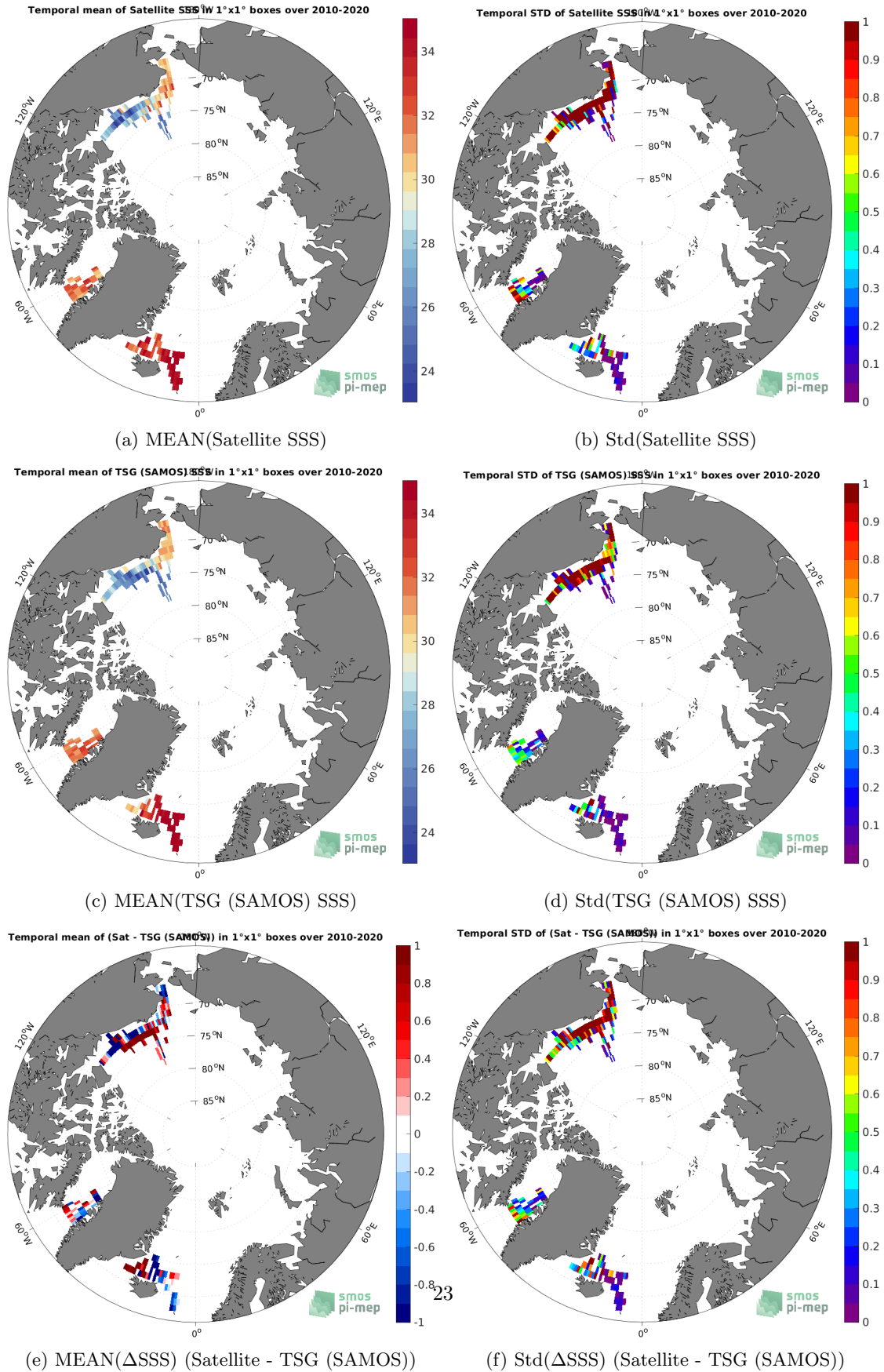
Figure 6: Temporal mean (left) and Std (right) of SSS from SMOS SSS L3 v335 - 10 Days - 25 km (CATDS-CPDC) (top), TSG (SAMOS) (middle), and of \Delta SSS (Satellite - TSG (SAMOS)). Only match-up pairs are used to generate these maps.
