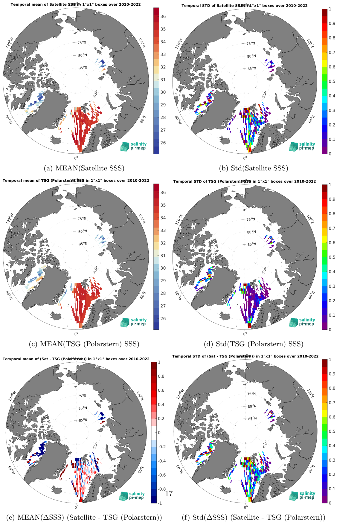
Figure 7: Temporal mean (left) and Std (right) of SSS from SMOS SSS L3 v335 - 10 Days - 25 km (CATDS-CPDC) (top), TSG (Polarstern) (middle), and of \Delta SSS (Satellite - TSG (Polarstern)). Only match-up pairs are used to generate these maps.
