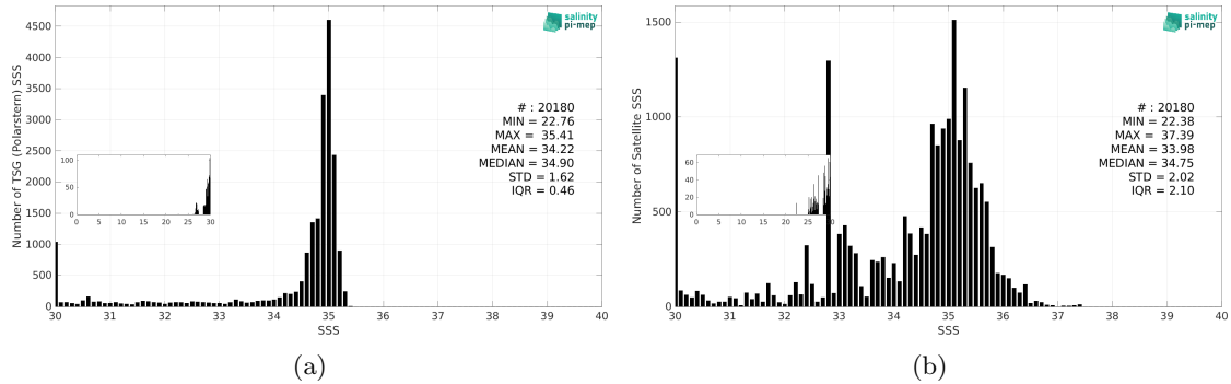
Figure 3: Histograms of SSS from TSG (Polarstern) (a) and SMOS SSS L3 v335 - 10 Days - 25 km (CATDS-CPDC) (b) considering all match-up pairs per bins of 0.1 over the Arctic Ocean Pi-MEP region and for the full satellite product period.
