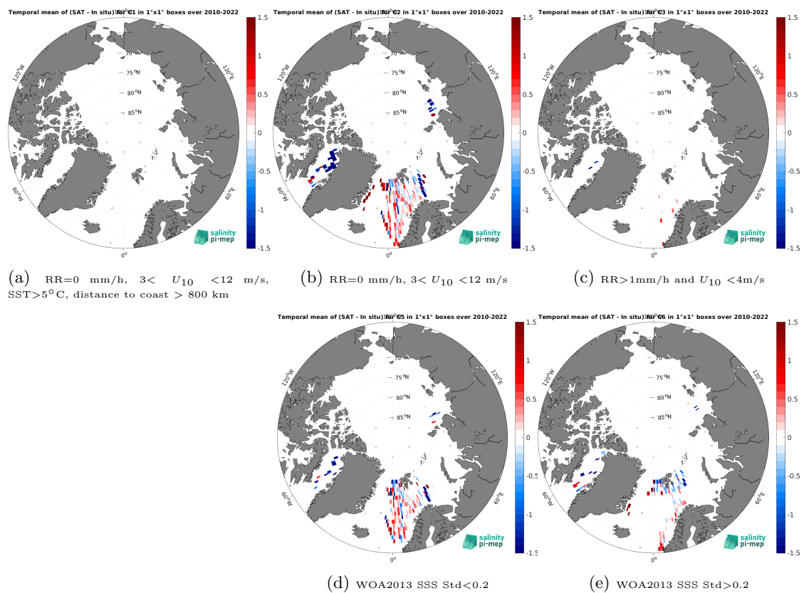
Figure 14: Temporal mean gridded over spatial boxes of size 1^\circ \times 1^\circ of \Delta SSS (SMOS SSS L3 v335 - 10 Days - 25 km (CATDS-CPDC) - TSG (Polarstern)) for 5 different subdatasets corresponding to: RR=0 mm/h, 3 < U_{10} < 12 m/s, SST > 5^\circ\text{C} , distance to coast > 800 km (a), RR=0 mm/h, 3 < U_{10} < 12 m/s (b), RR > 1 mm/h and U_{10} < 4 m/s (c), WOA2013 SSS Std < 0.2 (d), WOA2013 SSS Std > 0.2 (e).
