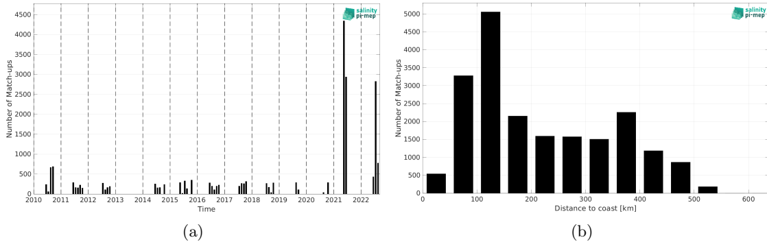
Figure 2: Number of match-ups between TSG (Polarstern) and SMOS SSS L3 v335 - 10 Days - 25 km (CATDS-CPDC) SSS as a function of time (a) and as function of the distance to coast (b) over the Arctic Ocean Pi-MEP region and for the full satellite product period.
