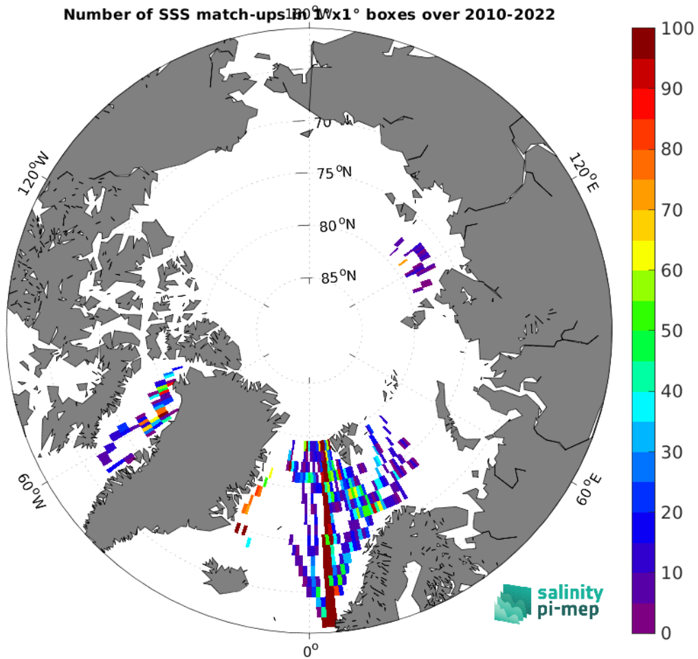
Figure 5: Number of SSS match-ups between TSG (Polarstern) SSS and the SMOS SSS L3 v335 - 10 Days - 25 km (CATDS-CPDC) SSS product for the Arctic Ocean Pi-MEP region over 1^\circ \times 1^\circ boxes and for the full satellite product period.
