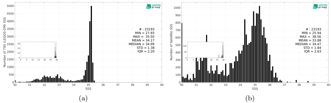
Figure 3: Histograms of SSS from TSG (LEGOS-DM) (a) and SMOS SSS L3 v335 - 10 Days - 25 km (CATDS-CPDC) (b) considering all match-up pairs per bins of 0.1 over the Arctic Ocean Pi-MEP region and for the full satellite product period.
