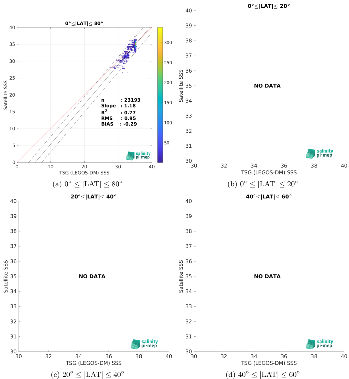
Figure 10: Contour maps of the concentration of SMOS SSS L3 v335 - 10 Days - 25 km (CATDS-CPDC) SSS (y-axis) versus TSG (LEGOS-DM) SSS (x-axis) at match-up pairs for different latitude bands. For each plot, the red line shows x=y . The black thin and dashed lines indicate a linear fit through the data cloud and the \pm 95\% confidence levels, respectively. The number match-up pairs n , the slope and R^2 coefficient of the linear fit, the root mean square (RMS) and the mean bias between satellite and in situ data are indicated for each latitude band in each plots.
