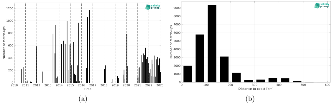
Figure 2: Number of match-ups between TSG (LEGOS-DM) and SMOS SSS L3 v335 - 10 Days - 25 km (CATDS-CPDC) SSS as a function of time (a) and as function of the distance to coast (b) over the Arctic Ocean Pi-MEP region and for the full satellite product period.
