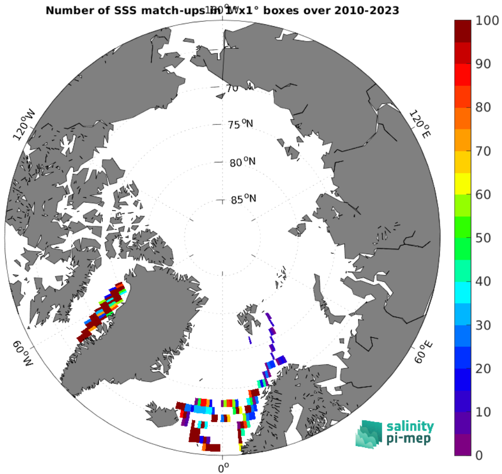
Figure 5: Number of SSS match-ups between TSG (LEGOS-DM) SSS and the SMOS SSS L3 v335 - 10 Days - 25 km (CATDS-CPDC) SSS product for the Arctic Ocean Pi-MEP region over 1^\circ \times 1^\circ boxes and for the full satellite product period.
