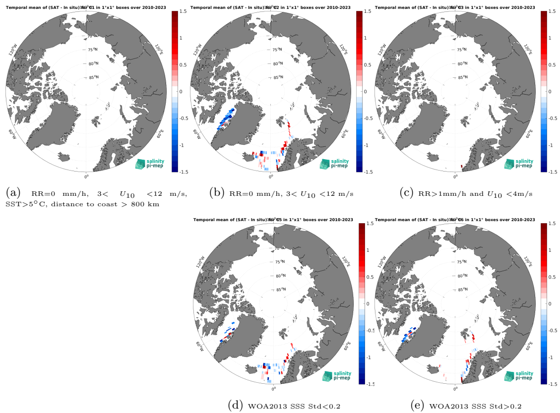
Figure 14: Temporal mean gridded over spatial boxes of size 1^\circ \times 1^\circ of \Delta SSS (SMOS SSS L3 v335 - 10 Days - 25 km (CATDS-CPDC) - TSG (LEGOS-DM)) for 5 different subdatasets corresponding to:RR=0 mm/h, 3 < U_{10} < 12 m/s, SST>5°C, distance to coast > 800 km (a), RR=0 mm/h, 3 < U_{10} < 12 m/s (b), RR>1mm/h and U_{10} < 4 m/s (c), WOA2013 SSS Std<0.2 (d), WOA2013 SSS Std>0.2 (e).
