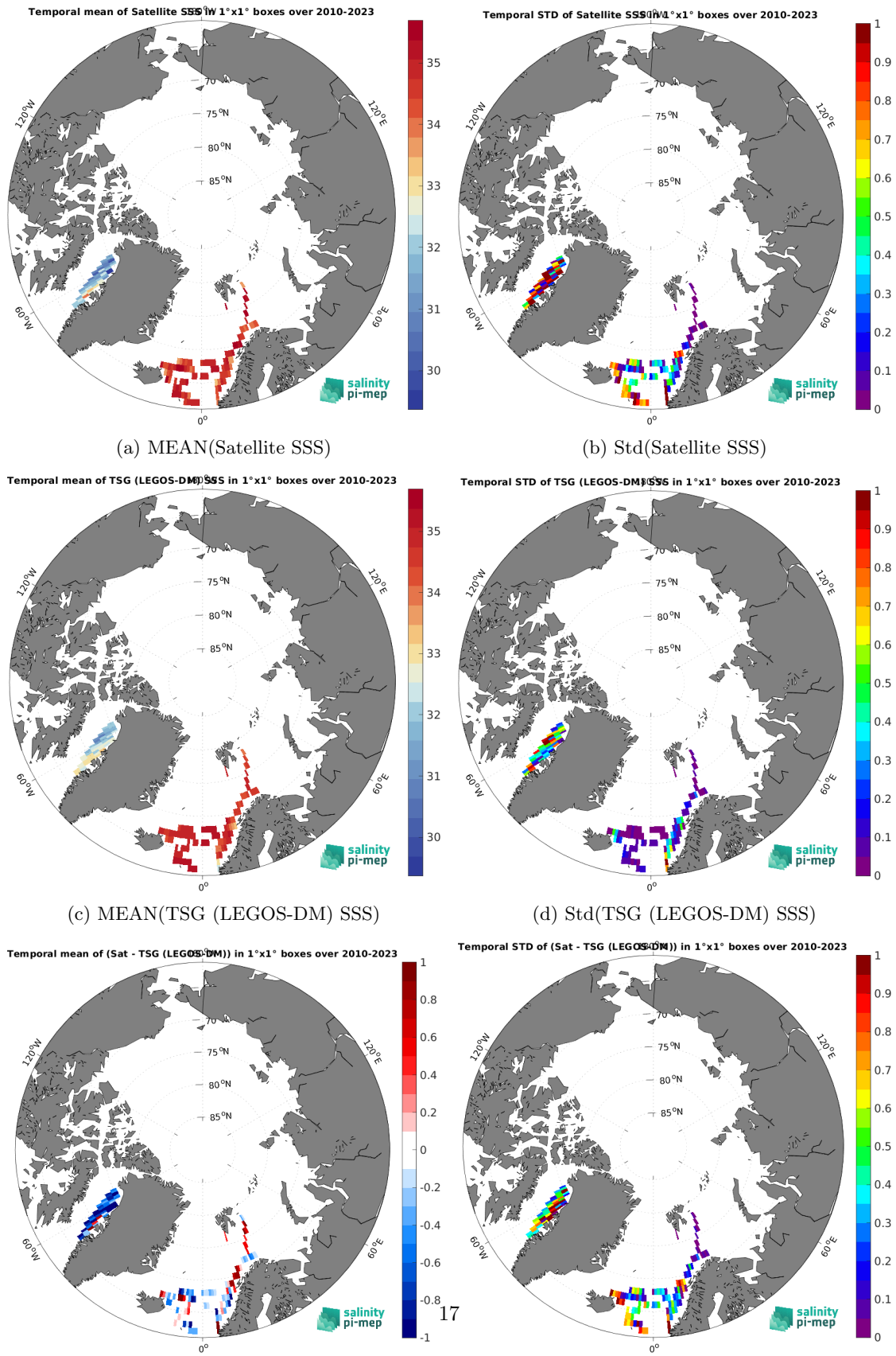
Figure 7: Temporal mean (left) and Std (right) of SSS from SMOS SSS L3 v335 - 10 Days - 25 km (CATDS-CPDC) (top), TSG (LEGOS-DM) (middle), and of \Delta SSS (Satellite - TSG (LEGOS-DM)). Only match-up pairs are used to generate these maps.
