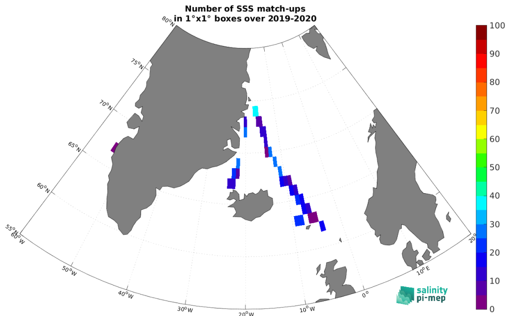
Figure 5: Number of SSS match-ups between TSG (Lauge-Koch) SSS and the SMOS SSS L3 v335 - 10 Days - 25 km (CATDS-CPDC) SSS product for the Arctic Ocean Pi-MEP region over 1^\circ \times 1^\circ boxes and for the full satellite product period.
