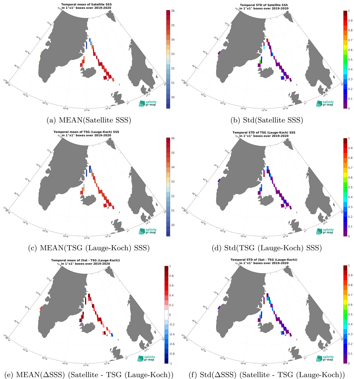
Figure 7: Temporal mean (left) and Std (right) of SSS from SMOS SSS L3 v335 - 10 Days - 25 km (CATDS-CPDC) (top), TSG (Lauge-Koch) (middle), and of \Delta SSS (Satellite - TSG (Lauge-Koch)). Only match-up pairs are used to generate these maps.
