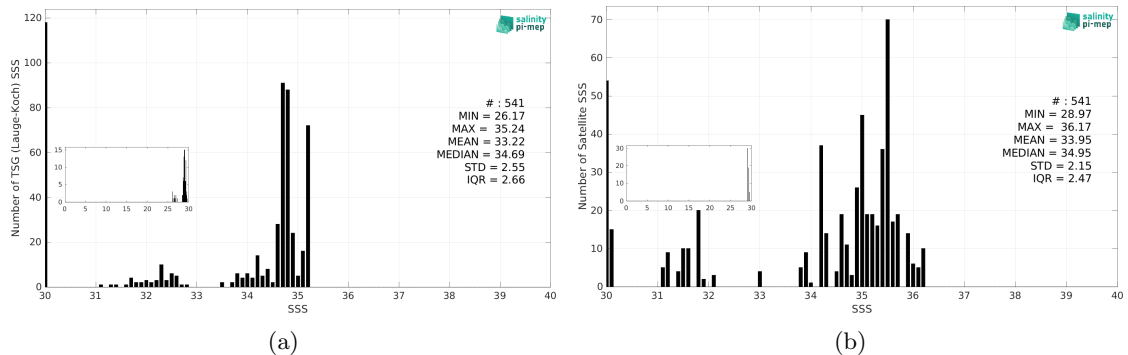
Figure 3: Histograms of SSS from TSG (Lauge-Koch) (a) and SMOS SSS L3 v335 - 10 Days - 25 km (CATDS-CPDC) (b) considering all match-up pairs per bins of 0.1 over the Arctic Ocean Pi-MEP region and for the full satellite product period.
