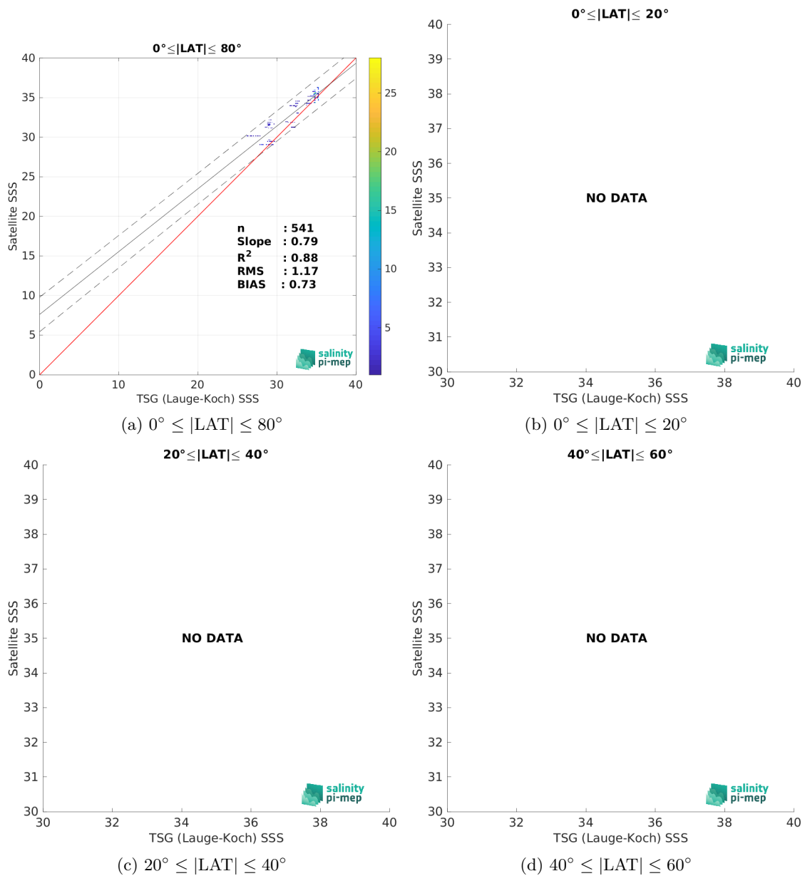
Figure 10: Contour maps of the concentration of SMOS SSS L3 v335 - 10 Days - 25 km (CATDS-CPDC) SSS (y-axis) versus TSG (Lauge-Koch) SSS (x-axis) at match-up pairs for different latitude bands. For each plot, the red line shows x=y . The black thin and dashed lines indicate a linear fit through the data cloud and the \pm 95\% confidence levels, respectively. The number match-up pairs n , the slope and R^2 coefficient of the linear fit, the root mean square (RMS) and the mean bias between satellite and in situ data are indicated for each latitude band in each plots.
