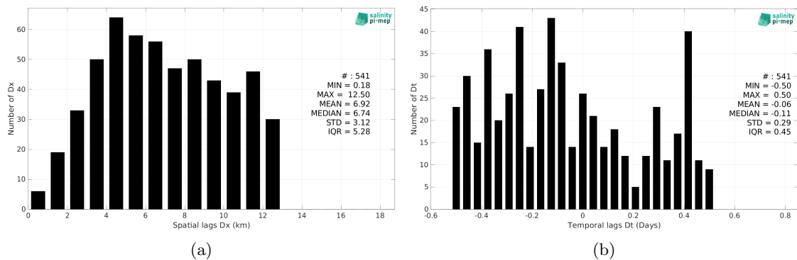
Figure 6: Histograms of the spatial (a) and temporal (b) lags between the location/time of the TSG (Lauge-Koch) measurement and the date of the corresponding SMOS SSS L3 v335 - 10 Days - 25 km (CATDS-CPDC) SSS pixel.
