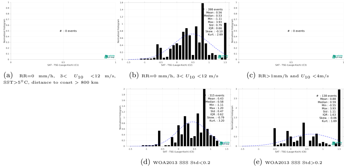
Figure 15: Normalized histogram of \Delta SSS (SMOS SSS L3 v335 - 10 Days - 25 km (CATDS-CPDC) - TSG (Lauge-Koch)) for 5 different subdatasets corresponding to: RR=0 mm/h, 3 < U_{10} < 12 m/s, SST>5°C, distance to coast > 800 km (a), RR=0 mm/h, 3 < U_{10} < 12 m/s (b), RR>1mm/h and U_{10} < 4 m/s (c), WOA2013 SSS Std<0.2 (d), WOA2013 SSS Std>0.2 (e).
