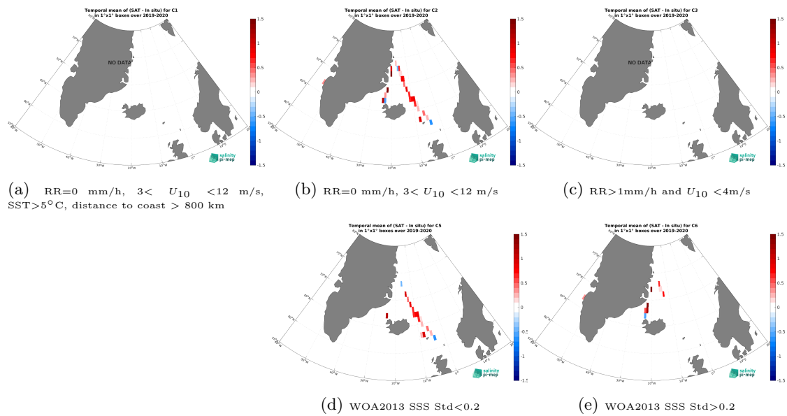
Figure 14: Temporal mean gridded over spatial boxes of size 1^\circ \times 1^\circ of \Delta SSS (SMOS SSS L3 v335 - 10 Days - 25 km (CATDS-CPDC) - TSG (Lauge-Koch)) for 5 different subdatasets corresponding to: RR=0 mm/h, 3 < U_{10} < 12 m/s, SST > 5^\circ C, distance to coast > 800 km (a), RR=0 mm/h, 3 < U_{10} < 12 m/s (b), RR > 1 mm/h and U_{10} < 4 m/s (c), WOA2013 SSS Std < 0.2 (d), WOA2013 SSS Std > 0.2 (e).
