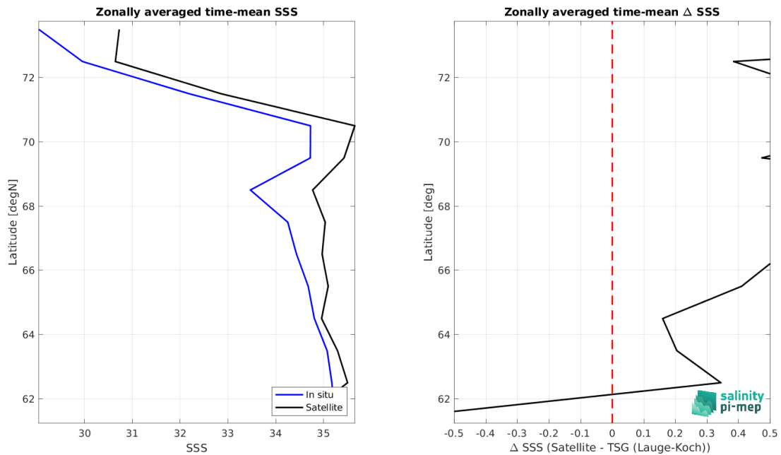
Figure 9: Left panel: Zonal mean SSS from SMOS SSS L3 v335 - 10 Days - 25 km (CATDS-CPDC) satellite product (black) and from TSG (Lauge-Koch) (blue). Right panel: Zonal mean of \Delta SSS (Satellite - TSG (Lauge-Koch)) for all the collected Pi-MEP match-up pairs estimated over the full satellite product period.
