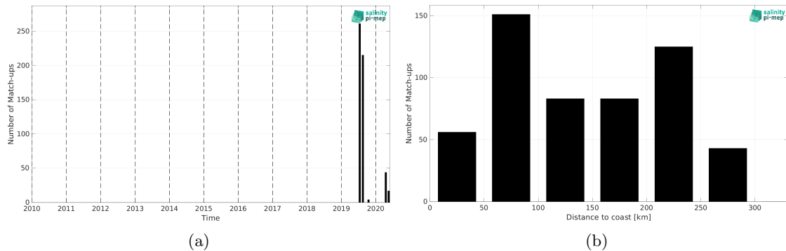
Figure 2: Number of match-ups between TSG (Lauge-Koch) and SMOS SSS L3 v335 - 10 Days - 25 km (CATDS-CPDC) SSS as a function of time (a) and as function of the distance to coast (b) over the Arctic Ocean Pi-MEP region and for the full satellite product period.
