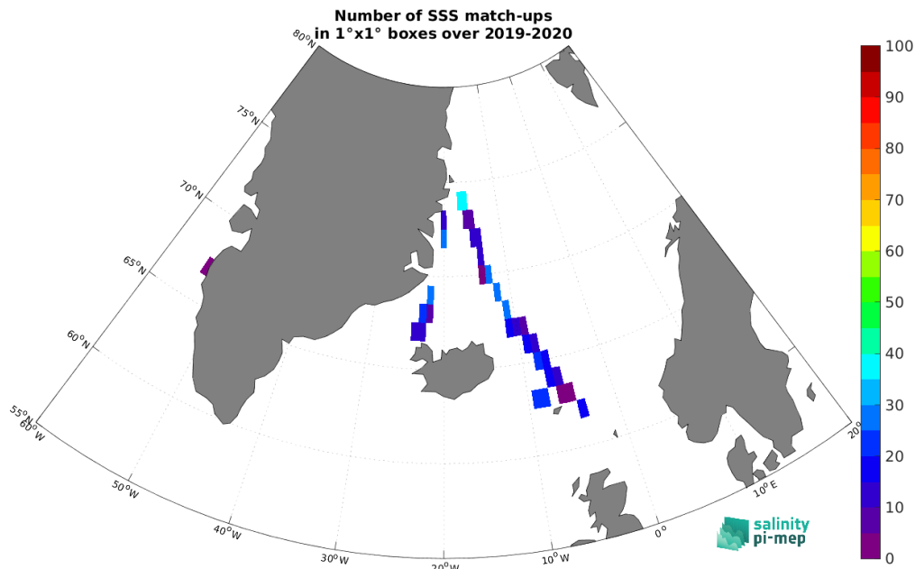
Figure 5: Number of SSS match-ups between TSG (Lauge-Koch) SSS and the SMOS SSS L3 v335 - 10 Days - 25 km (CATDS-CPDC) SSS product for the Arctic Ocean Pi-MEP region over 1^\circ \times 1^\circ boxes and for the full satellite product period.
