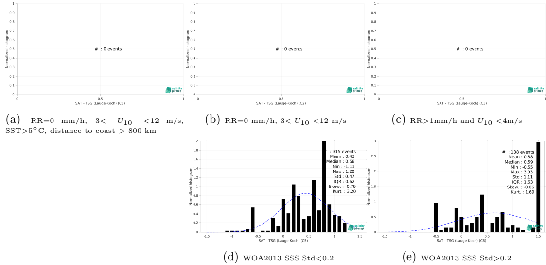
Figure 13: Normalized histogram of \Delta SSS (SMOS SSS L3 v335 - 10 Days - 25 km (CATDS-CPDC) - TSG (Laue-Koch)) for 5 different subdatasets corresponding to: RR=0 mm/h, 3 < U_{10} < 12 m/s, SST>5°C, distance to coast > 800 km (a), RR=0 mm/h, 3 < U_{10} < 12 m/s (b), RR>1mm/h and U_{10} < 4 m/s (c), WOA2013 SSS Std<0.2 (d), WOA2013 SSS Std>0.2 (e).
