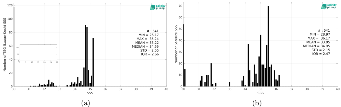
Figure 2: Histograms of SSS from TSG (Lauge-Koch) (a) and SMOS SSS L3 v335 - 10 Days - 25 km (CATDS-CPDC) (b) considering all match-up pairs per bins of 0.1 over the Arctic Ocean Pi-MEP region and for the full satellite product period.
