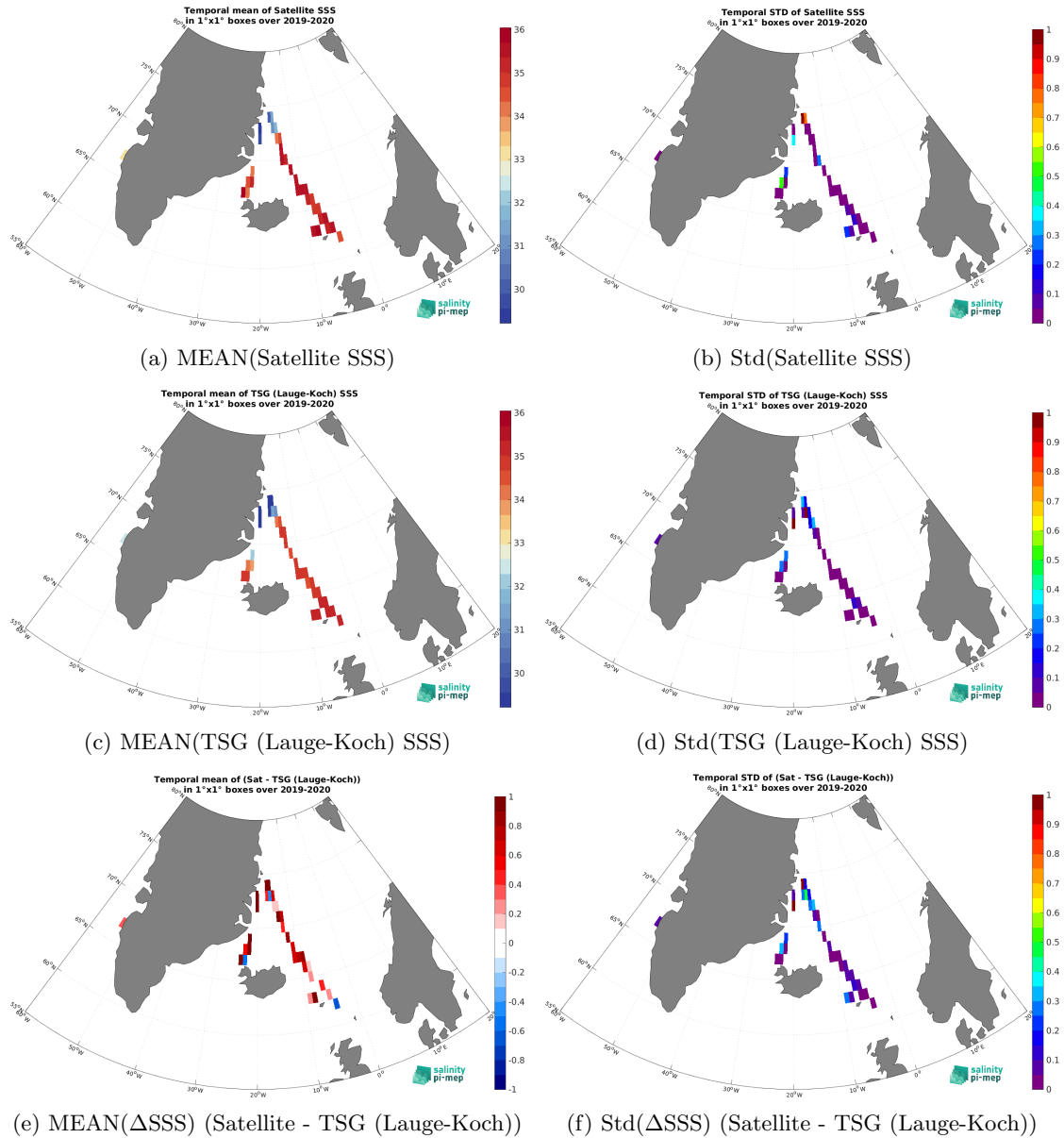
Figure 6: Temporal mean (left) and Std (right) of SSS from SMOS SSS L3 v335 - 10 Days - 25 km (CATDS-CPDC) (top), TSG (Lauge-Koch) (middle), and of \Delta SSS (Satellite - TSG (Lauge-Koch)). Only match-up pairs are used to generate these maps.
