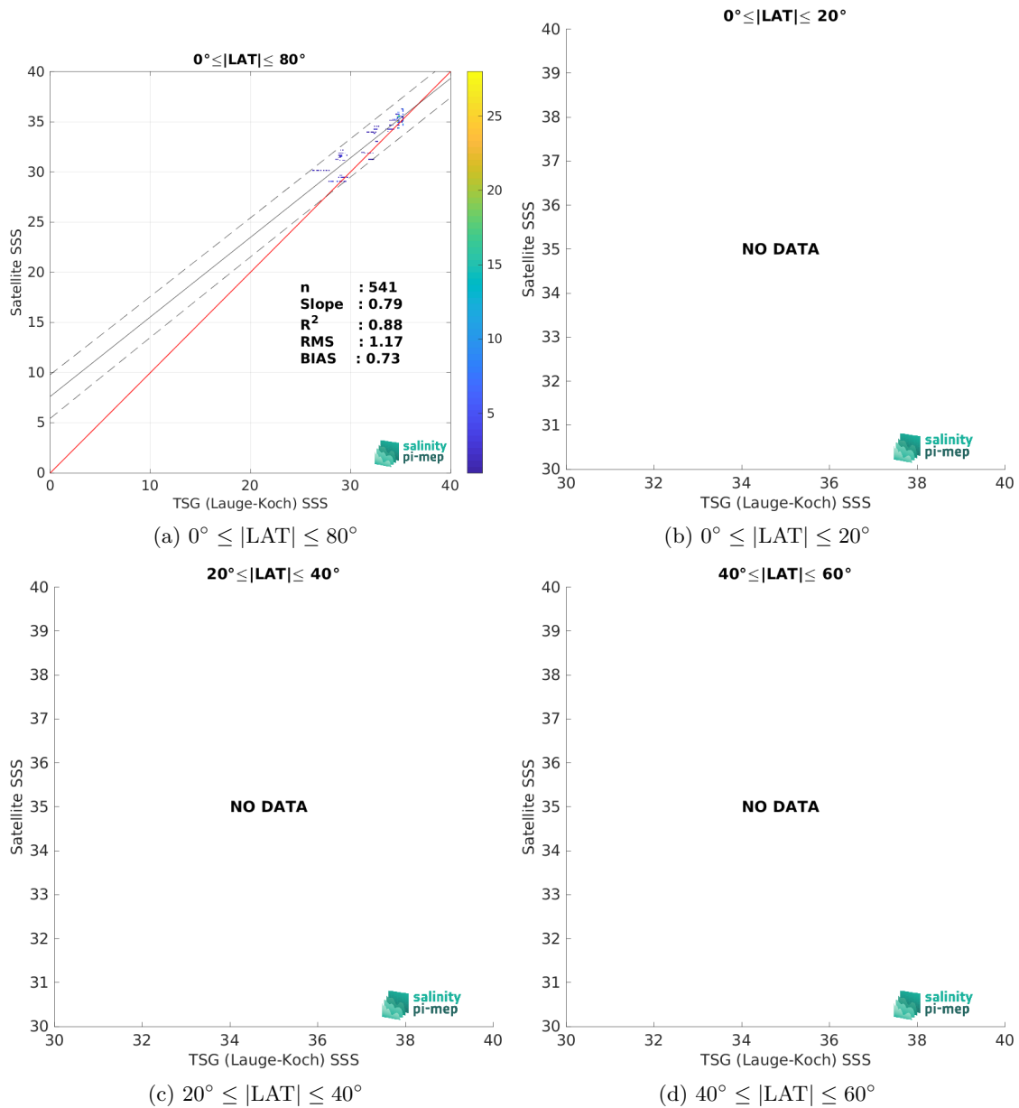
Figure 9: Contour maps of the concentration of SMOS SSS L3 v335 - 10 Days - 25 km (CATDS-CPDC) SSS (y-axis) versus TSG (Lauge-Koch) SSS (x-axis) at match-up pairs for different latitude bands. For each plot, the red line shows x=y . The black thin and dashed lines indicate a linear fit through the data cloud and the \pm 95\% confidence levels, respectively. The number match-up pairs n , the slope and R^2 coefficient of the linear fit, the root mean square (RMS) and the mean bias between satellite and in situ data are indicated for each latitude band in each plots.
