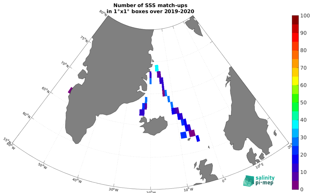
Figure 4: Number of SSS match-ups between TSG (Lauge-Koch) SSS and the SMOS SSS L3 v335 - 10 Days - 25 km (CATDS-CPDC) SSS product for the Arctic Ocean Pi-MEP region over 1^\circ \times 1^\circ boxes and for the full satellite product period.
