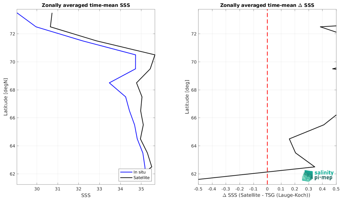
Figure 8: Left panel: Zonal mean SSS from SMOS SSS L3 v335 - 10 Days - 25 km (CATDS-CPDC) satellite product (black) and from TSG (Lauge-Koch) (blue). Right panel: Zonal mean of \Delta SSS (Satellite - TSG (Lauge-Koch)) for all the collected Pi-MEP match-up pairs estimated over the full satellite product period.
