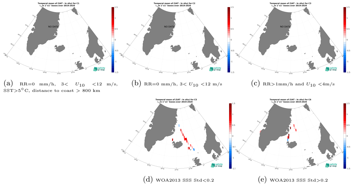
Figure 12: Temporal mean gridded over spatial boxes of size 1^{\circ}\times 1^{\circ} of \Delta\text{SSS} (SMOS SSS L3 v335 - 10 Days - 25 km (CATDS-CPDC) - TSG (Lauge-Koch)) for 5 different subdatasets corresponding to:RR=0 mm/h, 3 < U_{10} < 12 m/s, SST >5^{\circ}\text{C} , distance to coast > 800 km (a), RR=0 mm/h, 3 < U_{10} < 12 m/s (b), RR >1 mm/h and U_{10} < 4 m/s (c), WOA2013 SSS Std <0.2 (d), WOA2013 SSS Std >0.2 (e).
