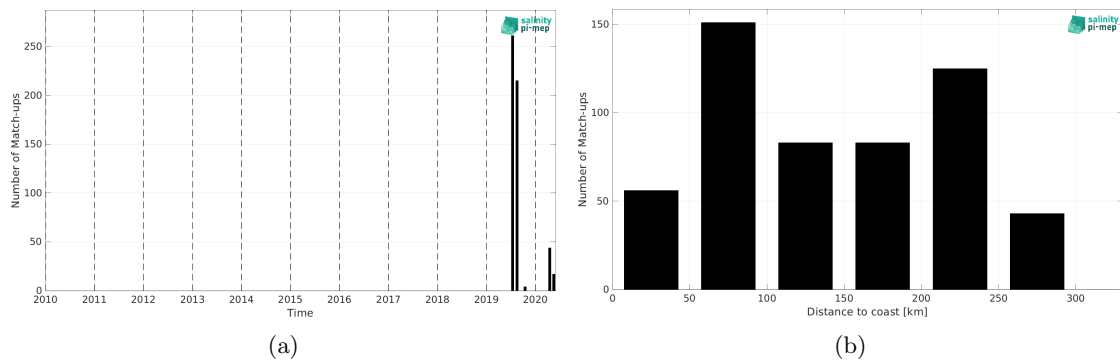
Figure 1: Number of match-ups between TSG (Lauge-Koch) and SMOS SSS L3 v335 - 10 Days - 25 km (CATDS-CPDC) SSS as a function of time (a) and as function of the distance to coast (b) over the Arctic Ocean Pi-MEP region and for the full satellite product period.
