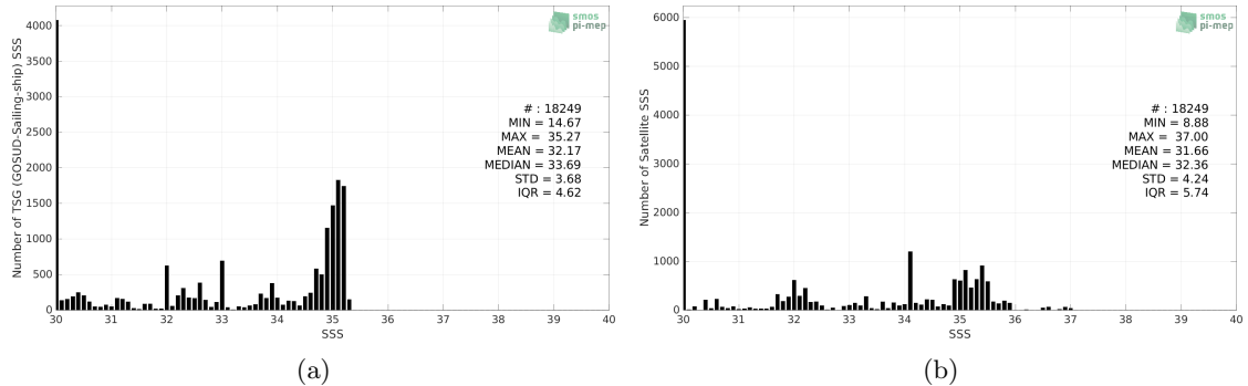
Figure 2: Histograms of SSS from TSG (GOSUD-Sailing-ship) (a) and SMOS SSS L3 v335 - 10 Days - 25 km (CATDS-CPDC) (b) considering all match-up pairs per bins of 0.1 over the Arctic Ocean Pi-MEP region and for the full satellite product period.
