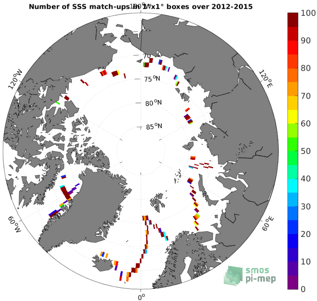
Figure 4: Number of SSS match-ups between TSG (GOSUD-Sailing-ship) SSS and the SMOS SSS L3 v335 - 10 Days - 25 km (CATDS-CPDC) SSS product for the Arctic Ocean Pi-MEP region over 1^\circ \times 1^\circ boxes and for the full satellite product period.
