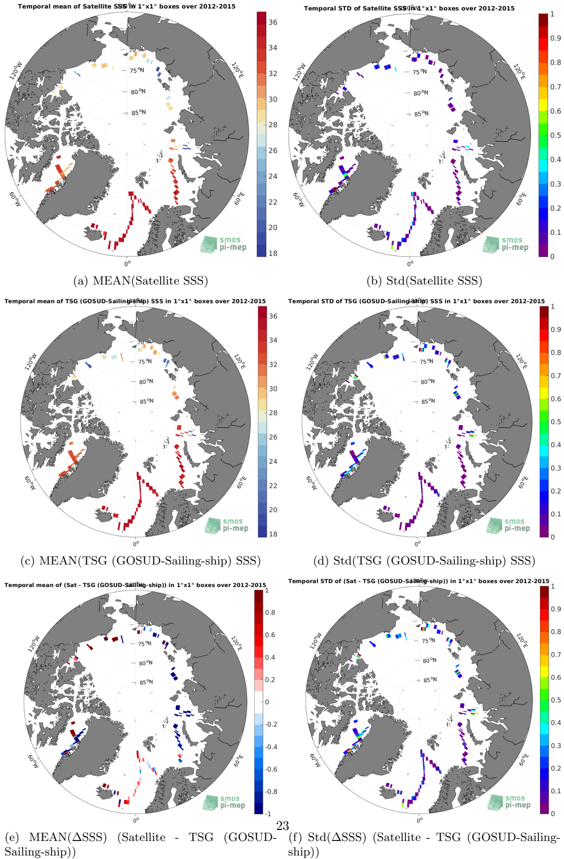
Figure 6: Temporal mean (left) and Std (right) of SSS from SMOS SSS L3 v335 - 10 Days - 25 km (CATDS-CPDC) (top), TSG (GOSUD-Sailing-ship) (middle), and of \Delta SSS (Satellite - TSG (GOSUD-Sailing-ship)). Only match-up pairs are used to generate these maps.
