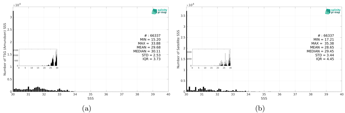
Figure 3: Histograms of SSS from TSG (Amundsen) (a) and SMOS SSS L3 v335 - 10 Days - 25 km (CATDS-CPDC) (b) considering all match-up pairs per bins of 0.1 over the Arctic Ocean Pi-MEP region and for the full satellite product period.
