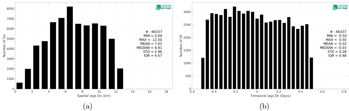
Figure 6: Histograms of the spatial (a) and temporal (b) lags between the location/time of the TSG (Amundsen) measurement and the date of the corresponding SMOS SSS L3 v335 - 10 Days - 25 km (CATDS-CPDC) SSS pixel.
