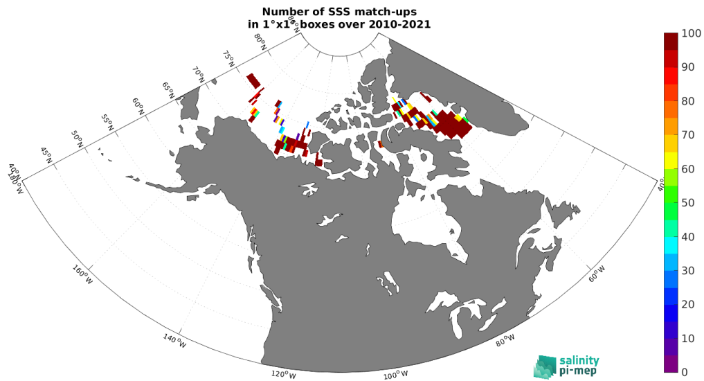
Figure 5: Number of SSS match-ups between TSG (Amundsen) SSS and the SMOS SSS L3 v335 - 10 Days - 25 km (CATDS-CPDC) SSS product for the Arctic Ocean Pi-MEP region over 1^\circ \times 1^\circ boxes and for the full satellite product period.
