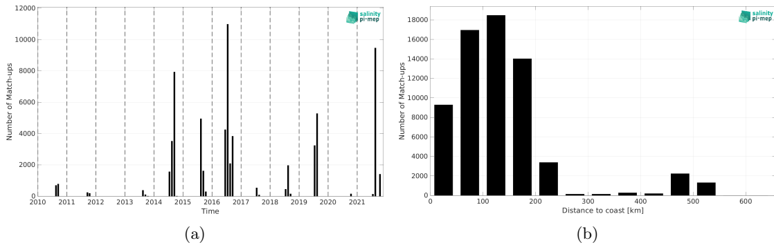
Figure 2: Number of match-ups between TSG (Amundsen) and SMOS SSS L3 v335 - 10 Days - 25 km (CATDS-CPDC) SSS as a function of time (a) and as function of the distance to coast (b) over the Arctic Ocean Pi-MEP region and for the full satellite product period.
