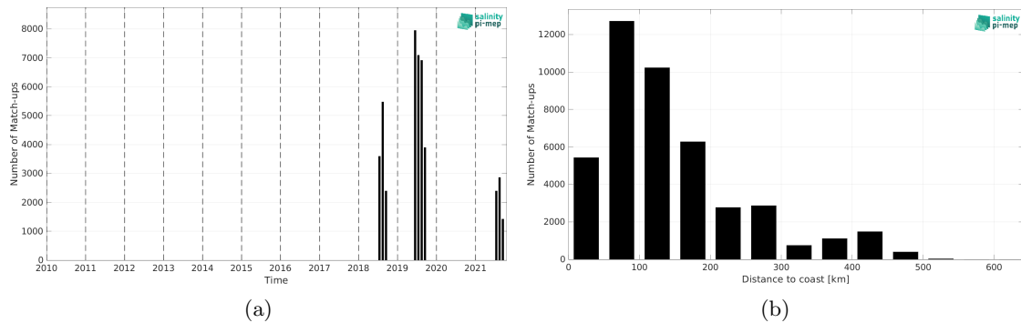
Figure 2: Number of match-ups between Saildrone and SMOS SSS L3 v335 - 10 Days - 25 km (CATDS-CPDC) SSS as a function of time (a) and as function of the distance to coast (b) over the Arctic Ocean Pi-MEP region and for the full satellite product period.
