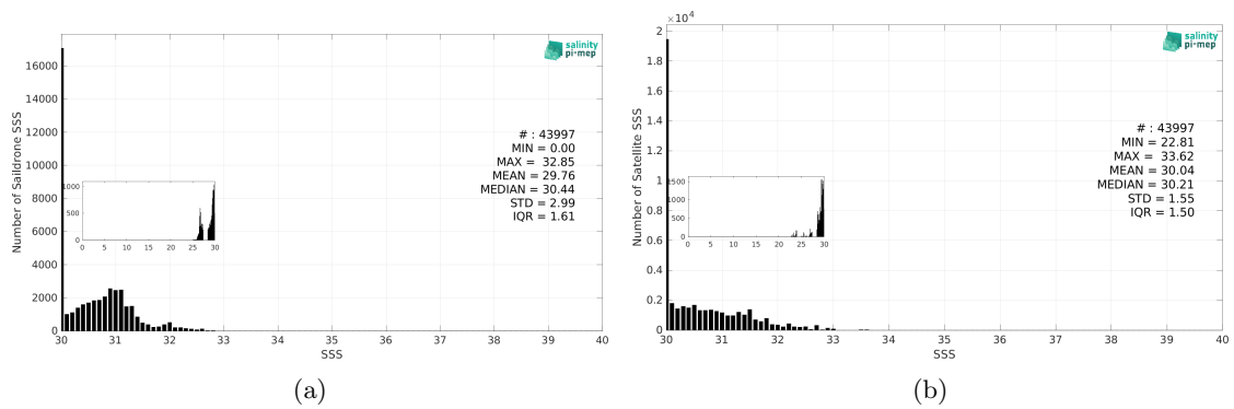
Figure 3: Histograms of SSS from Saildrone (a) and SMOS SSS L3 v335 - 10 Days - 25 km (CATDS-CPDC) (b) considering all match-up pairs per bins of 0.1 over the Arctic Ocean Pi-MEP region and for the full satellite product period.
