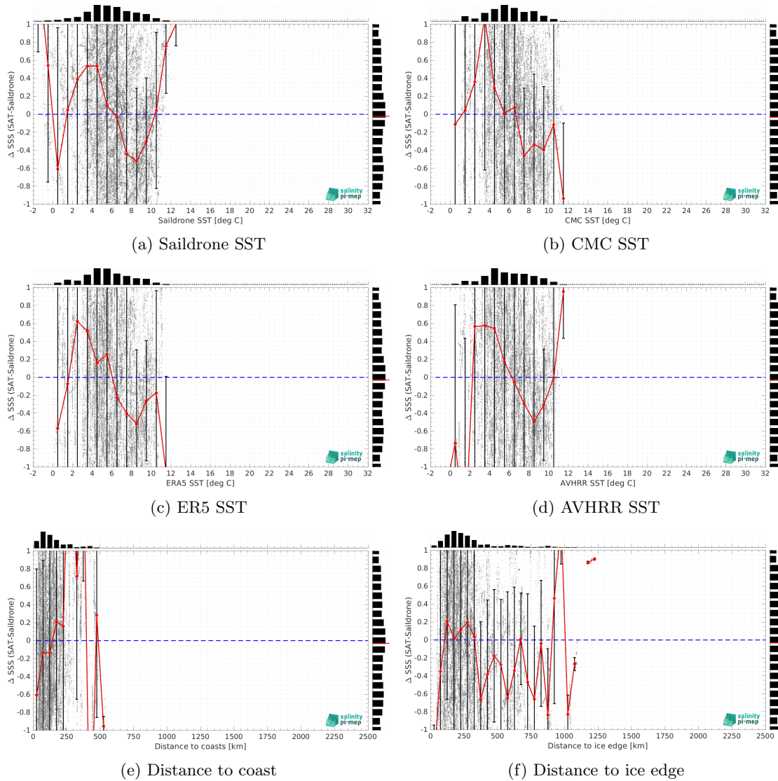
Figure 13: \Delta SSS (Satellite - Saiddrone) sorted as function of Saildrone SST values (a), CMC SST (b), ERA5 SST (c), AVHRR SST (d), distance to coast (e) and distance to ice edge (f). In all plots the median and Std of \Delta SSS for each bin is indicated by the red curves and black vertical thick bars ( \pm 1 Std). Links to similar figures sorted as function of Sea ice fraction and in situ measurement depth .
