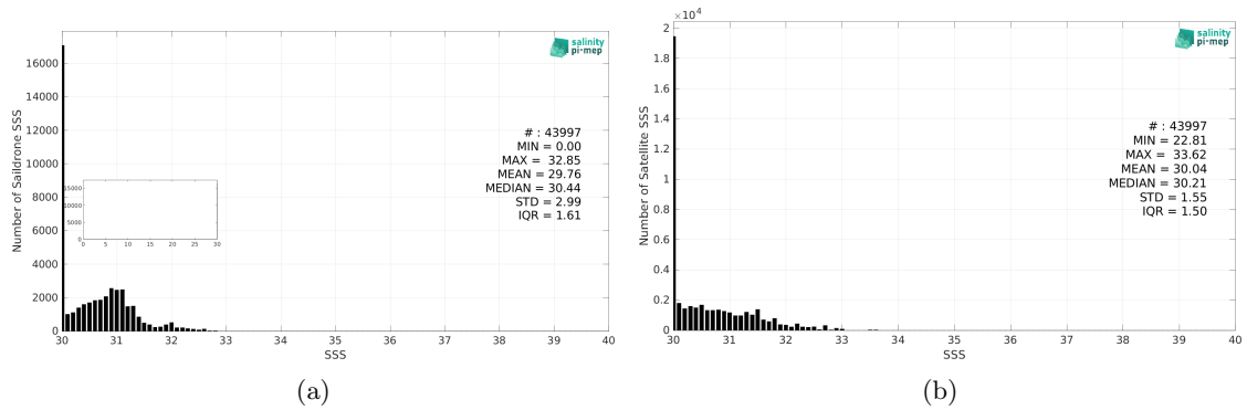
Figure 2: Histograms of SSS from Saildrone (a) and SMOS SSS L3 v335 - 10 Days - 25 km (CATDS-CPDC) (b) considering all match-up pairs per bins of 0.1 over the Arctic Ocean Pi-MEP region and for the full satellite product period.
