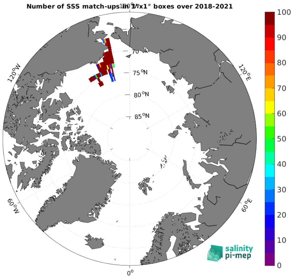
Figure 4: Number of SSS match-ups between Sailldrone SSS and the SMOS SSS L3 v335 - 10 Days - 25 km (CATDS-CPDC) SSS product for the Arctic Ocean Pi-MEP region over 1^\circ \times 1^\circ boxes and for the full satellite product period.
