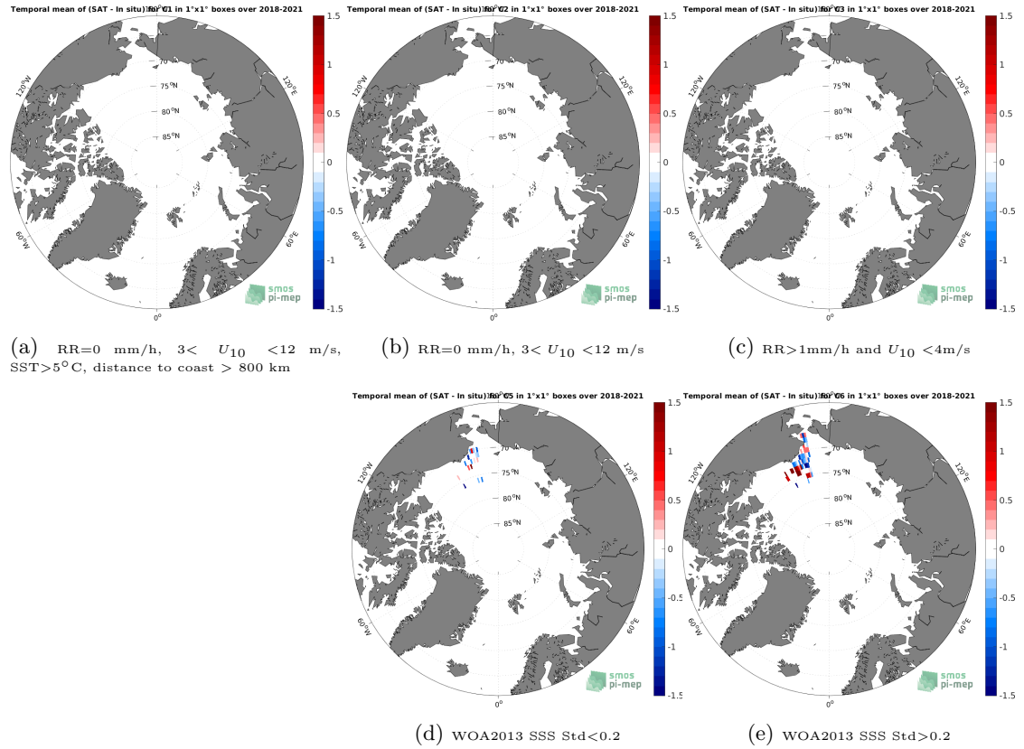
Figure 12: Temporal mean gridded over spatial boxes of size 1^{\circ}\times 1^{\circ} of \Delta\text{SSS} (SMOS SSS L3 v335 - 10 Days - 25 km (CATDS-CPDC) - Saildrone) for 5 different subdatasets corresponding to: RR=0 mm/h, 3 < U_{10} < 12 m/s, SST > 5^{\circ}\text{C} , distance to coast > 800 km (a), RR=0 mm/h, 3 < U_{10} < 12 m/s (b), RR > 1 mm/h and U_{10} < 4 m/s (c), WOA2013 SSS Std < 0.2 (d), WOA2013 SSS Std > 0.2 (e).
