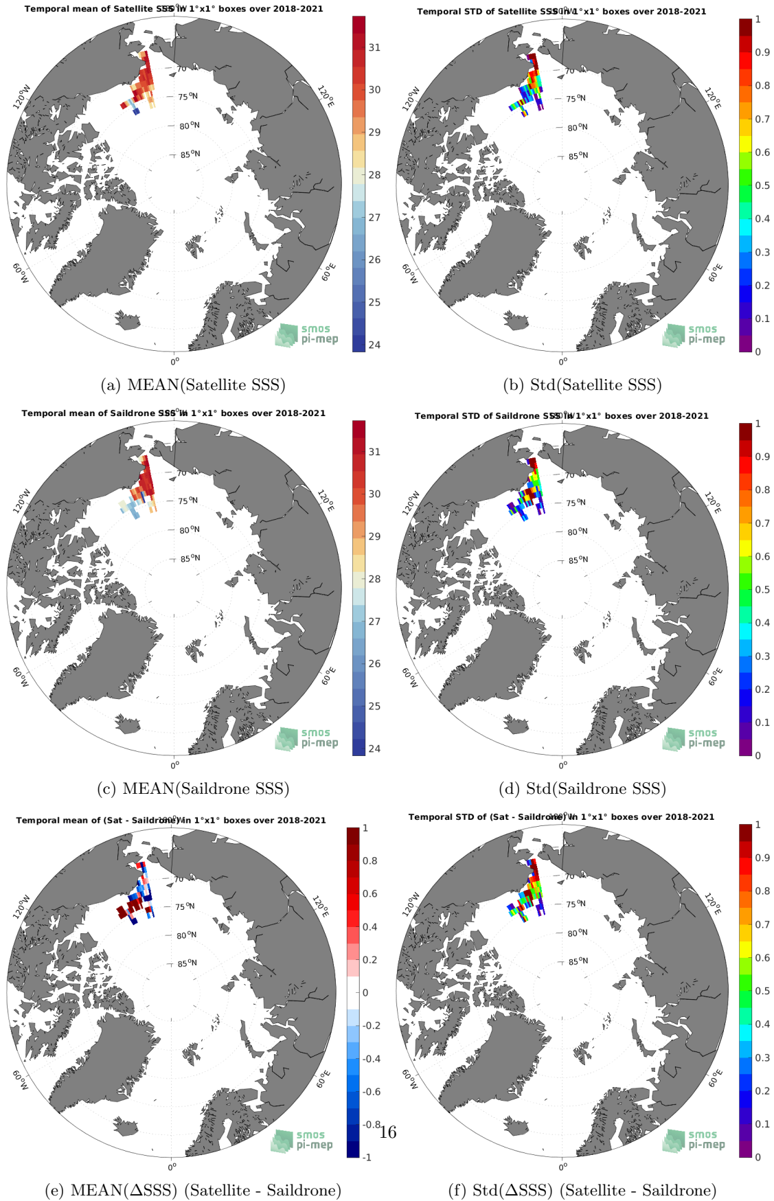
Figure 6: Temporal mean (left) and Std (right) of SSS from SMOS SSS L3 v335 - 10 Days - 25 km (CATDS-CPDC) (top), Saildrone (middle), and of \Delta SSS (Satellite - Saildrone). Only match-up pairs are used to generate these maps.
