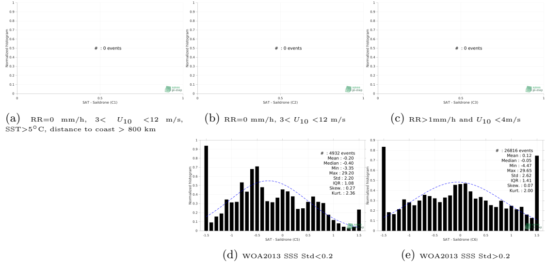
Figure 13: Normalized histogram of \Delta SSS (SMOS SSS L3 v335 - 10 Days - 25 km (CATDS-CPDC) - Salldrone) for 5 different subdatasets corresponding to: RR=0 mm/h, 3 < U_{10} < 12 m/s, SST>5°C, distance to coast > 800 km (a), RR=0 mm/h, 3 < U_{10} < 12 m/s (b), RR>1mm/h and U_{10} < 4 m/s (c), WOA2013 SSS Std<0.2 (d), WOA2013 SSS Std>0.2 (e).
