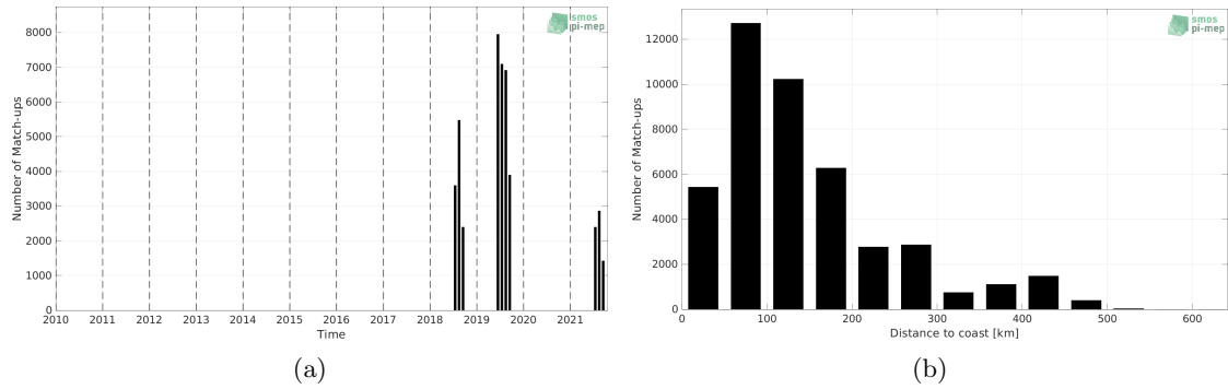
Figure 1: Number of match-ups between Saildrone and SMOS SSS L3 v335 - 10 Days - 25 km (CATDS-CPDC) SSS as a function of time (a) and as function of the distance to coast (b) over the Arctic Ocean Pi-MEP region and for the full satellite product period.
