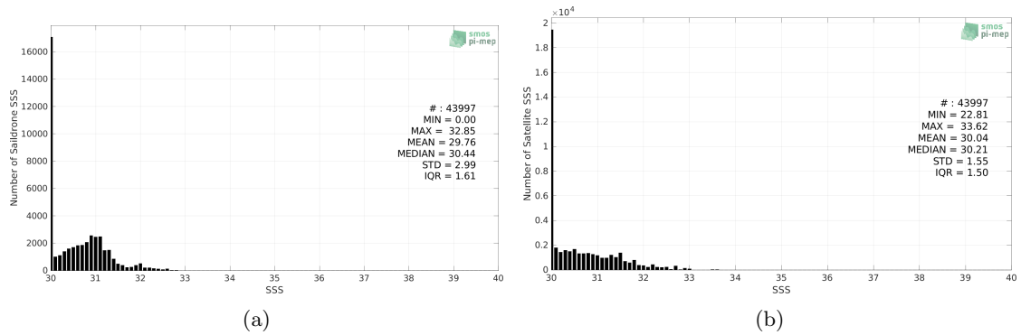
Figure 2: Histograms of SSS from Saikdrone (a) and SMOS SSS L3 v335 - 10 Days - 25 km (CATDS-CPDC) (b) considering all match-up pairs per bins of 0.1 over the Arctic Ocean Pi-MEP region and for the full satellite product period.
