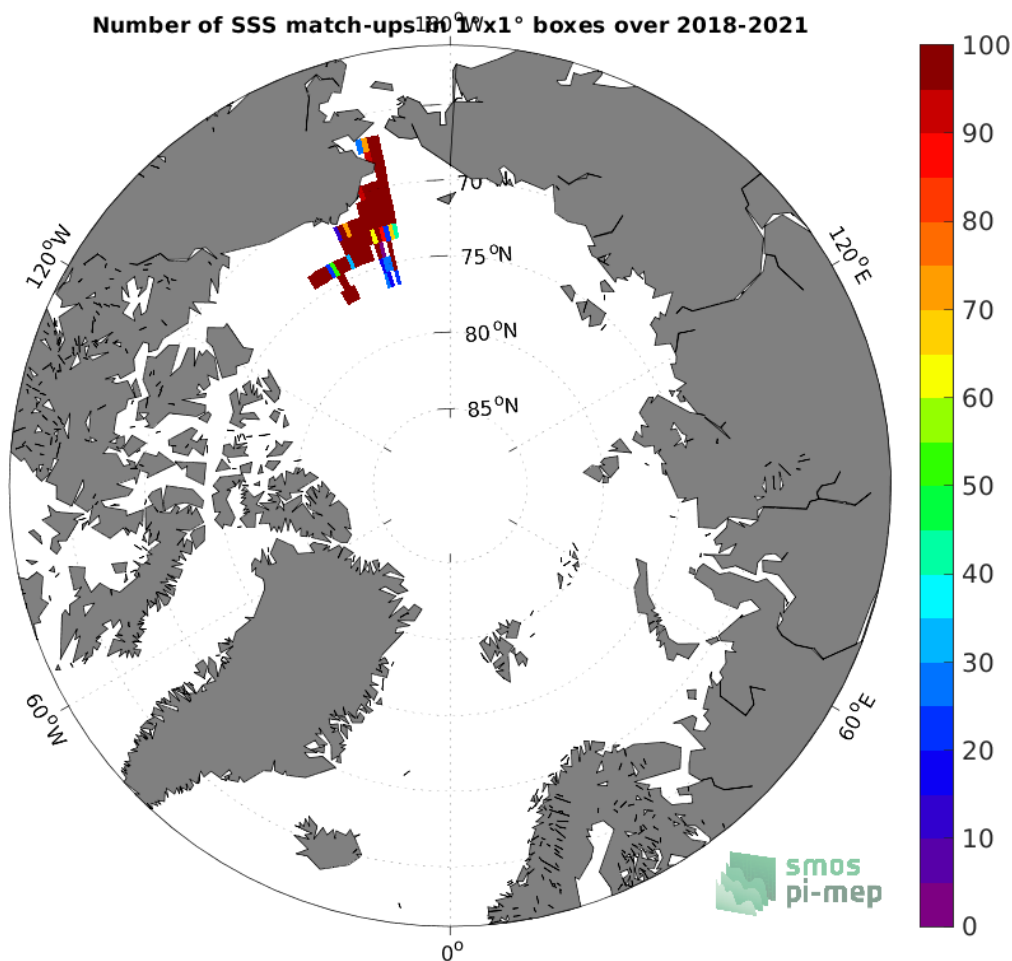
Figure 4: Number of SSS match-ups between Saildrone SSS and the SMOS SSS L3 v335 - 10 Days - 25 km (CATDS-CPDC) SSS product for the Arctic Ocean Pi-MEP region over 1^\circ \times 1^\circ boxes and for the full satellite product period.
