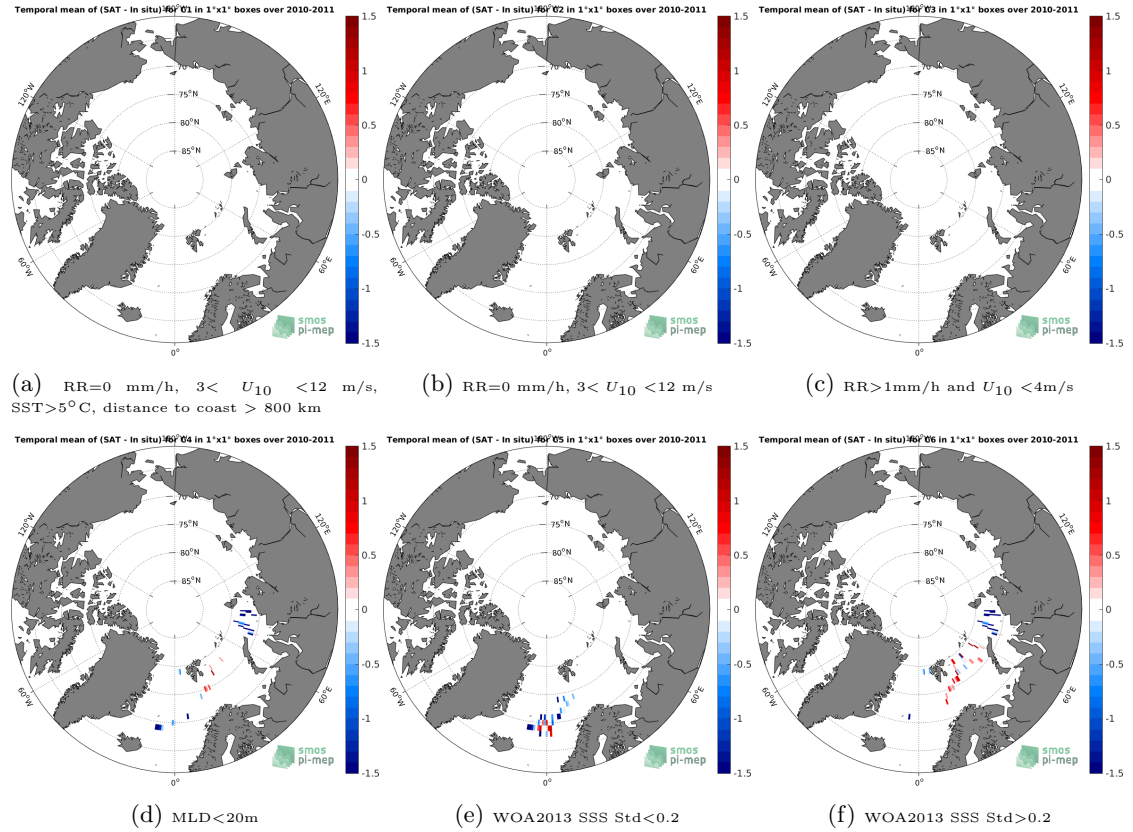
Figure 12: Temporal mean gridded over spatial boxes of size 1^{\circ} \times 1^{\circ} of \Delta\text{SSS} (SMOS SSS L3 v335 - 10 Days - 25 km (CATDS-CPDC) - Marine mammals) for 6 different subdatasets corresponding to: RR=0 mm/h, 3 < U_{10} < 12 m/s, SST > 5^{\circ}\text{C} , distance to coast > 800 km (a), RR=0 mm/h, 3 < U_{10} < 12 m/s (b), RR > 1 mm/h and U_{10} < 4 m/s (c), MLD < 20\text{m} (d), WOA2013 SSS Std < 0.2 (e), WOA2013 SSS Std > 0.2 (f).
