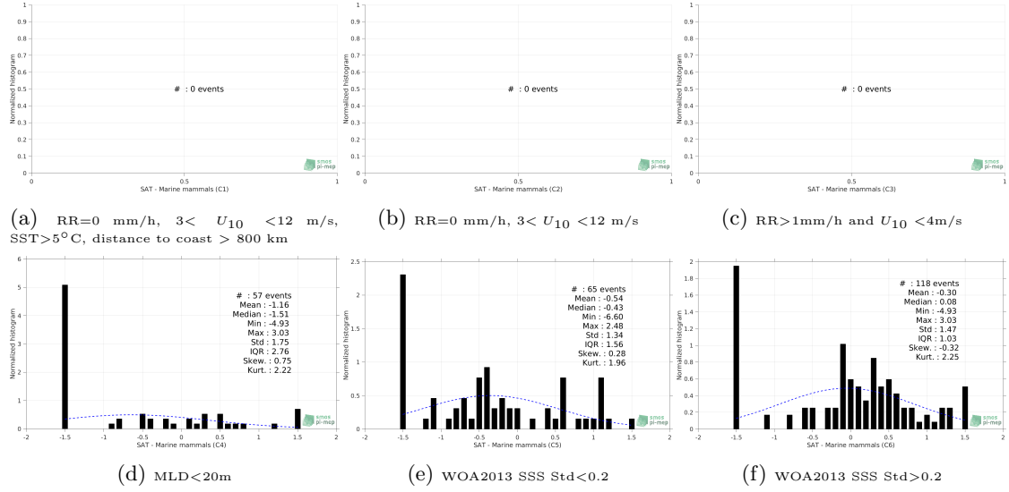
Figure 13: Normalized histogram of \Delta\text{SSS} (SMOS SSS L3 v335 - 10 Days - 25 km (CATDS-CPDC) - Marine mammals) for 6 different subdatasets corresponding to: RR=0 mm/h, 3 < U_{10} < 12 m/s, SST > 5^\circ\text{C} , distance to coast > 800 km (a), RR=0 mm/h, 3 < U_{10} < 12 m/s (b), RR > 1 mm/h and U_{10} < 4 m/s (c), MLD < 20 m (d), WOA2013 SSS Std < 0.2 (e), WOA2013 SSS Std > 0.2 (f).
