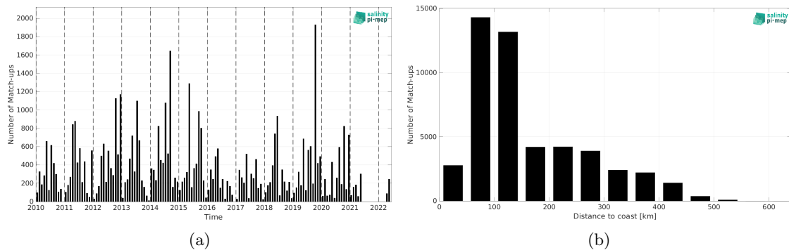
Figure 2: Number of match-ups between ICES and SMOS SSS L3 v335 - 10 Days - 25 km (CATDS-CPDC) SSS as a function of time (a) and as function of the distance to coast (b) over the Arctic Ocean Pi-MEP region and for the full satellite product period.
