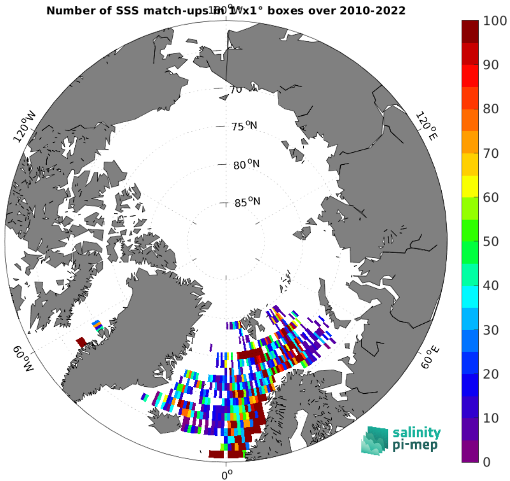
Figure 5: Number of SSS match-ups between ICES SSS and the SMOS SSS L3 v335 - 10 Days - 25 km (CATDS-CPDC) SSS product for the Arctic Ocean Pi-MEP region over 1^\circ \times 1^\circ boxes and for the full satellite product period.
