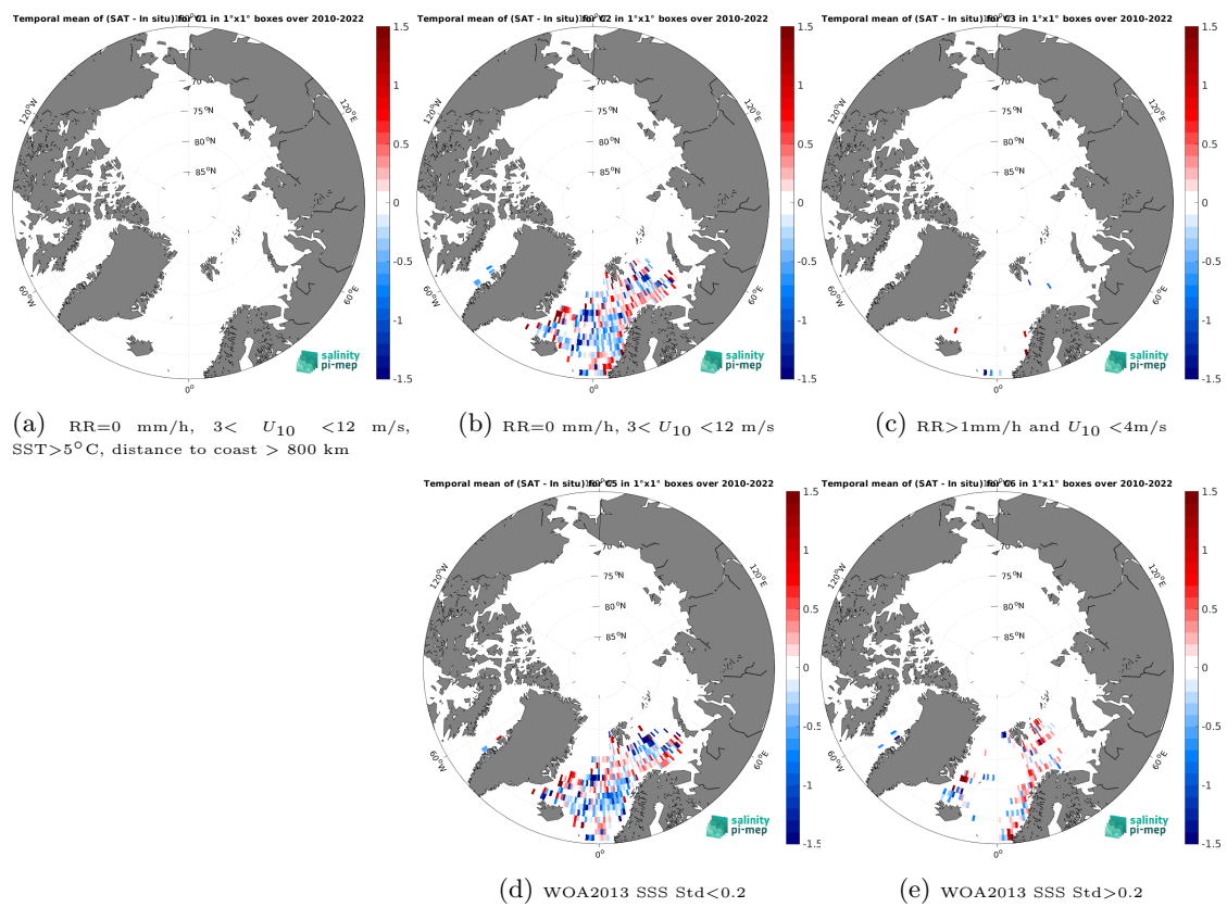
Figure 14: Temporal mean gridded over spatial boxes of size 1^\circ \times 1^\circ of \Delta\text{SSS} (SMOS SSS L3 v335 - 10 Days - 25 km (CATDS-CPDC) - ICES) for 5 different subdatasets corresponding to:RR=0 mm/h, 3 < U_{10} < 12 m/s, SST > 5°C, distance to coast > 800 km (a), RR=0 mm/h, 3 < U_{10} < 12 m/s (b), RR > 1mm/h and U_{10} < 4 m/s (c), WOA2013 SSS Std < 0.2 (d), WOA2013 SSS Std > 0.2 (e).
