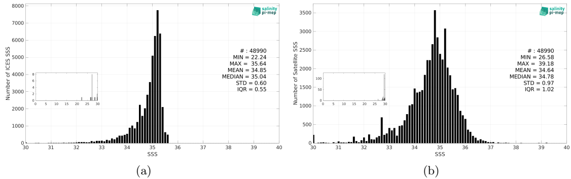
Figure 3: Histograms of SSS from ICES (a) and SMOS SSS L3 v335 - 10 Days - 25 km (CATDS-CPDC) (b) considering all match-up pairs per bins of 0.1 over the Arctic Ocean Pi-MEP region and for the full satellite product period.
