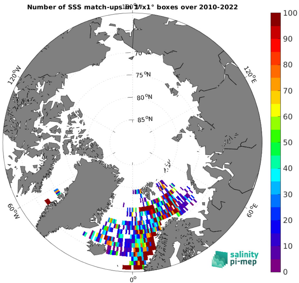
Figure 4: Number of SSS match-ups between ICES SSS and the SMOS SSS L3 v335 - 10 Days - 25 km (CATDS-CPDC) SSS product for the Arctic Ocean Pi-MEP region over 1^\circ \times 1^\circ boxes and for the full satellite product period.
