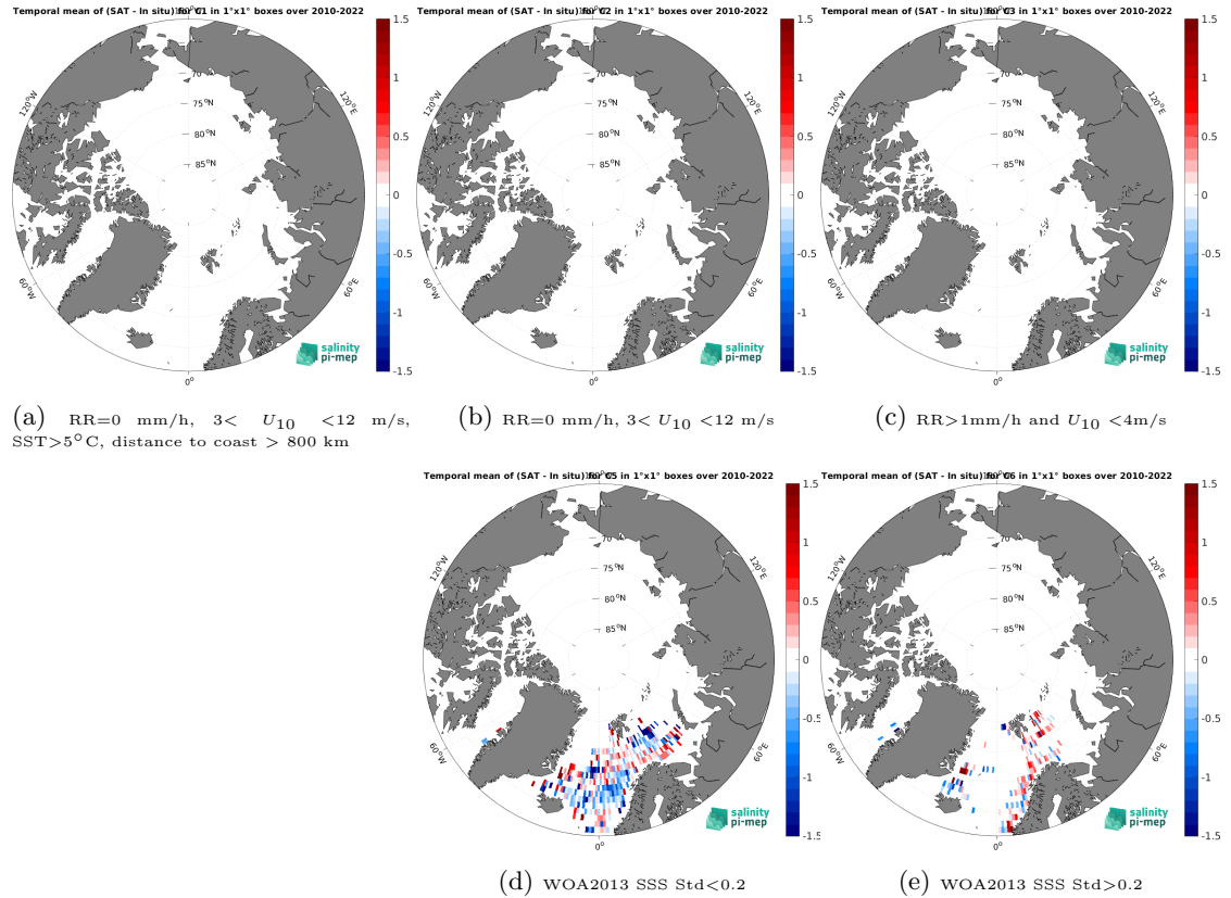
Figure 12: Temporal mean gridded over spatial boxes of size 1^{\circ}\times 1^{\circ} of \Delta\text{SSS} (SMOS SSS L3 v335 - 10 Days - 25 km (CATDS-CPDC) - ICES) for 5 different subdatasets corresponding to: RR=0 mm/h, 3 < U_{10} < 12 m/s, SST > 5^{\circ}\text{C} , distance to coast > 800 km (a), RR=0 mm/h, 3 < U_{10} < 12 m/s (b), RR > 1 mm/h and U_{10} < 4 m/s (c), WOA2013 SSS Std < 0.2 (d), WOA2013 SSS Std > 0.2 (e).
