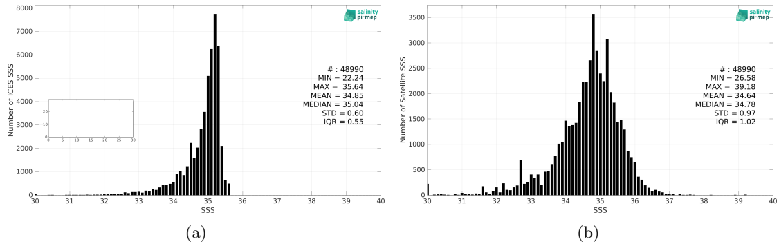
Figure 2: Histograms of SSS from ICES (a) and SMOS SSS L3 v335 - 10 Days - 25 km (CATDS-CPDC) (b) considering all match-up pairs per bins of 0.1 over the Arctic Ocean Pi-MEP region and for the full satellite product period.
