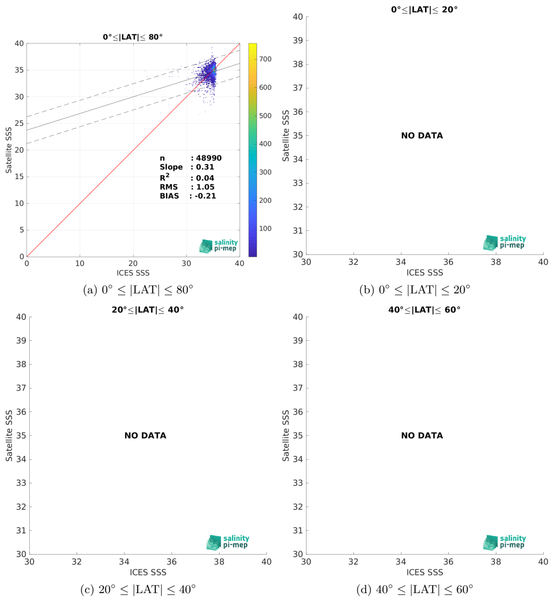
Figure 9: Contour maps of the concentration of SMOS SSS L3 v335 - 10 Days - 25 km (CATDS-CPDC) SSS (y-axis) versus ICES SSS (x-axis) at match-up pairs for different latitude bands. For each plot, the red line shows x=y . The black thin and dashed lines indicate a linear fit through the data cloud and the \pm 95\% confidence levels, respectively. The number match-up pairs n , the slope and R^2 coefficient of the linear fit, the root mean square (RMS) and the mean bias between satellite and in situ data are indicated for each latitude band in each plots.
