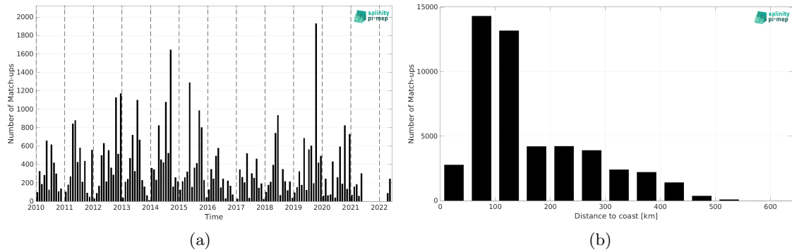
Figure 1: Number of match-ups between ICES and SMOS SSS L3 v335 - 10 Days - 25 km (CATDS-CPDC) SSS as a function of time (a) and as function of the distance to coast (b) over the Arctic Ocean Pi-MEP region and for the full satellite product period.
