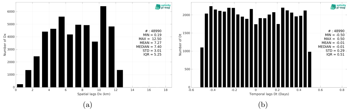
Figure 5: Histograms of the spatial (a) and temporal (b) lags between the location/time of the ICES measurement and the date of the corresponding SMOS SSS L3 v335 - 10 Days - 25 km (CATDS-CPDC) SSS pixel.
