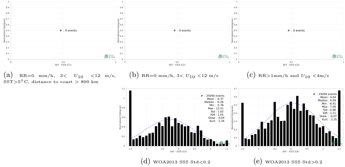
Figure 13: Normalized histogram of \Delta SSS (SMOS SSS L3 v335 - 10 Days - 25 km (CATDS-CPDC) - ICES) for 5 different subdatasets corresponding to: RR=0 mm/h, 3 < U_{10} < 12 m/s, SST>5°C, distance to coast > 800 km (a), RR=0 mm/h, 3 < U_{10} < 12 m/s (b), RR>1mm/h and U_{10} < 4 m/s (c), WOA2013 SSS Std<0.2 (d), WOA2013 SSS Std>0.2 (e).
