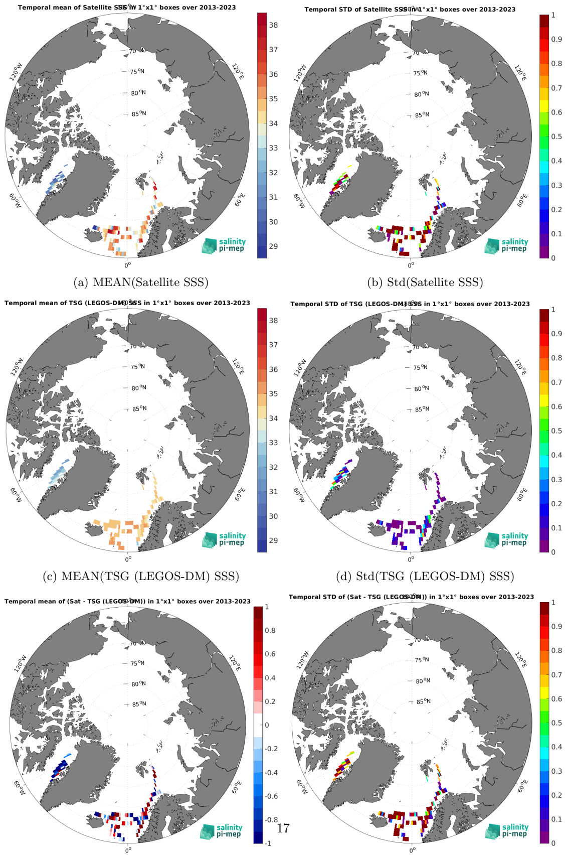
Figure 7: Temporal mean (left) and Std (right) of SSS from SMOS SSS L2Q v333 - 0.25 Deg (CATDS-CPDC) (top), TSG (LEGOS-DM) (middle), and of \Delta SSS (Satellite - TSG (LEGOS-DM)). Only match-up pairs are used to generate these maps.
