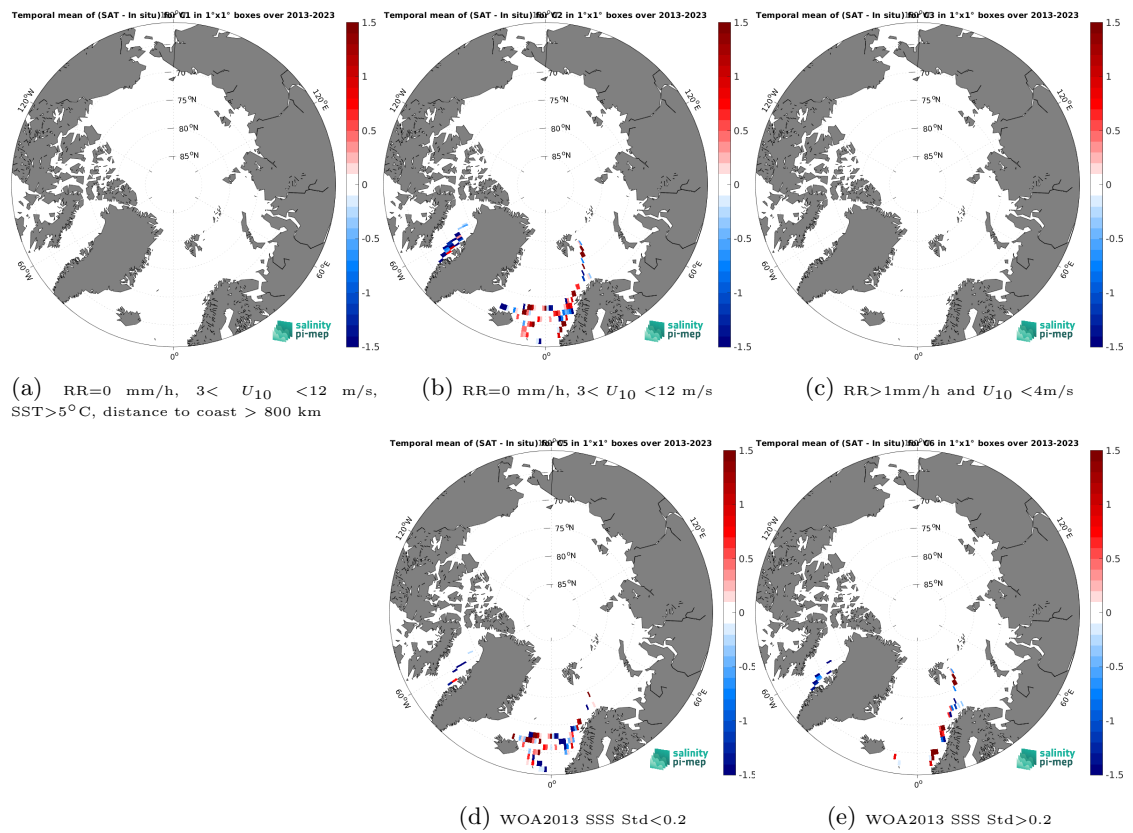
Figure 14: Temporal mean gridded over spatial boxes of size 1^\circ \times 1^\circ of \Delta SSS (SMOS SSS L2Q v333 - 0.25 Deg (CATDS-CPDC) - TSG (LEGOS-DM)) for 5 different subdatasets corresponding to: RR=0 mm/h, 3 < U_{10} < 12 m/s, SST > 5°C, distance to coast > 800 km (a), RR=0 mm/h, 3 < U_{10} < 12 m/s (b), RR > 1mm/h and U_{10} < 4 m/s (c), WOA2013 SSS Std < 0.2 (d), WOA2013 SSS Std > 0.2 (e).
