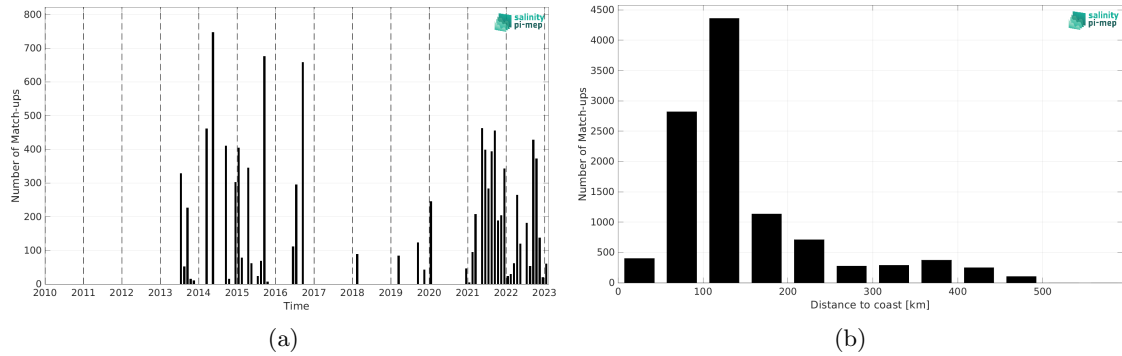
Figure 2: Number of match-ups between TSG (LEGOS-DM) and SMOS SSS L2Q v333 - 0.25 Deg (CATDS-CPDC) SSS as a function of time (a) and as function of the distance to coast (b) over the Arctic Ocean Pi-MEP region and for the full satellite product period.
