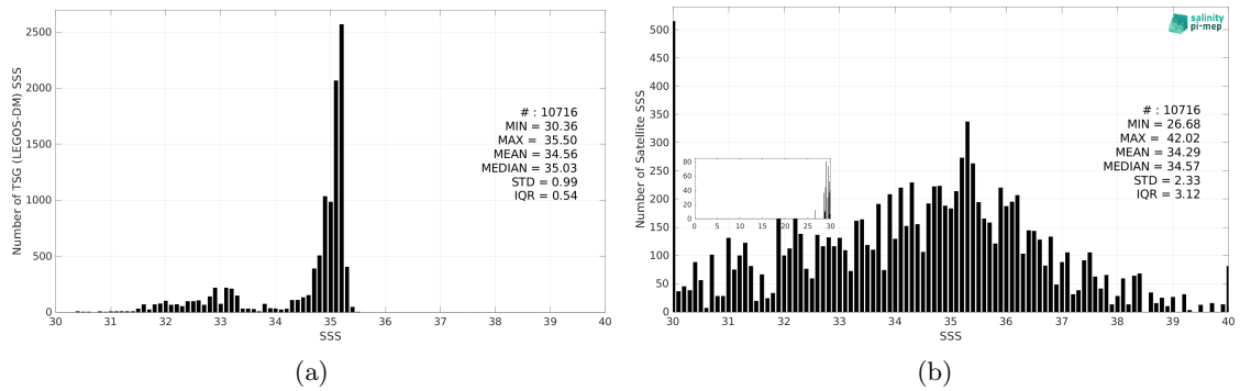
Figure 3: Histograms of SSS from TSG (LEGOS-DM) (a) and SMOS SSS L2Q v333 - 0.25 Deg (CATDS-CPDC) (b) considering all match-up pairs per bins of 0.1 over the Arctic Ocean Pi-MEP region and for the full satellite product period.
