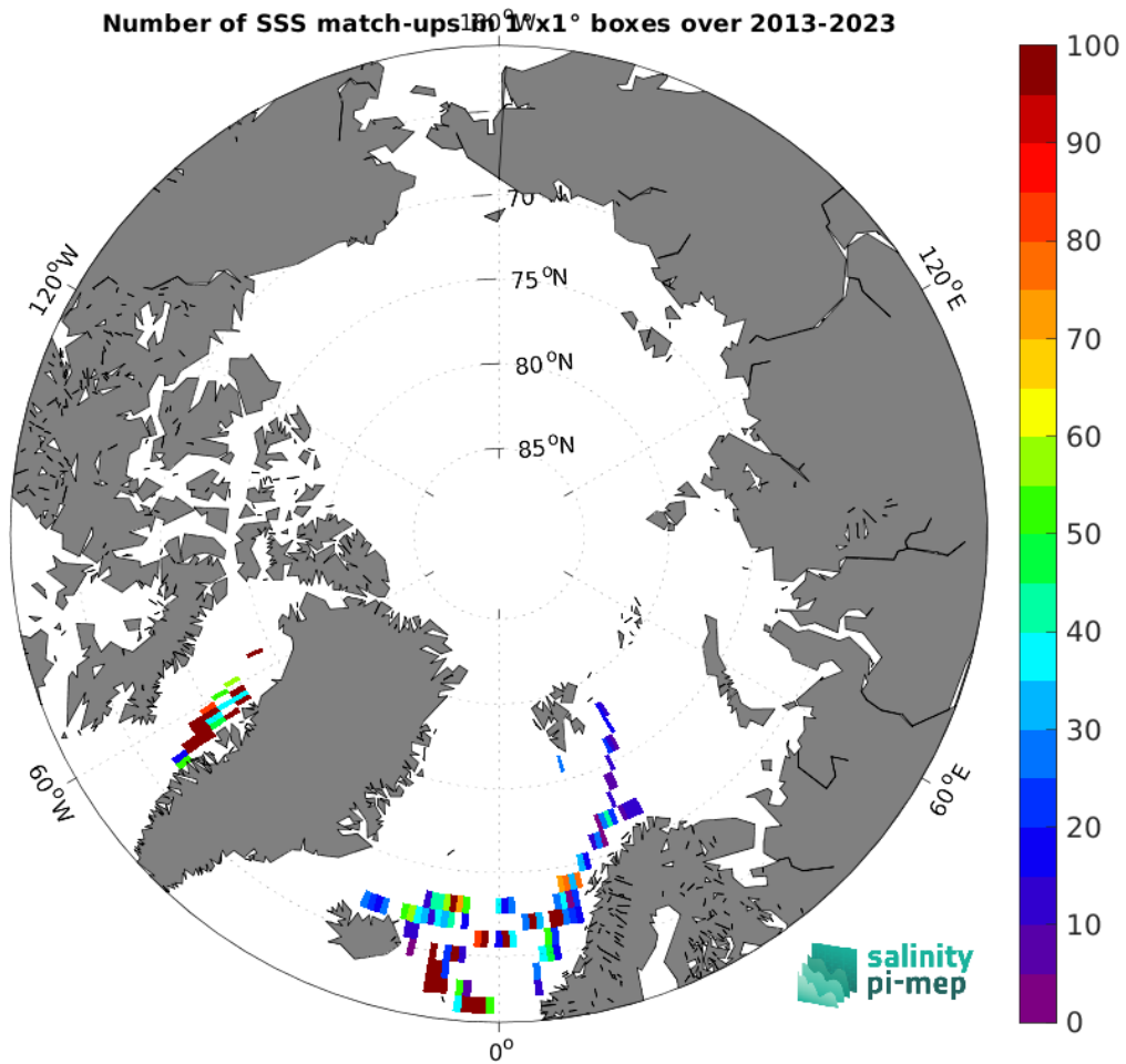
Figure 5: Number of SSS match-ups between TSG (LEGOS-DM) SSS and the SMOS SSS L2Q v333 - 0.25 Deg (CATDS-CPDC) SSS product for the Arctic Ocean Pi-MEP region over 1^\circ \times 1^\circ boxes and for the full satellite product period.
