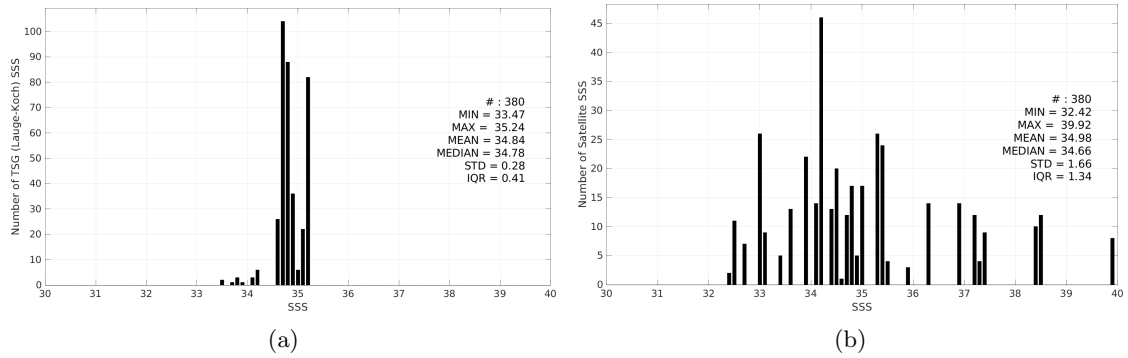
Figure 3: Histograms of SSS from TSG (Lauge-Koch) (a) and SMOS SSS L2Q v333 - 0.25 Deg (CATDS-CPDC) (b) considering all match-up pairs per bins of 0.1 over the Arctic Ocean Pi-MEP region and for the full satellite product period.
