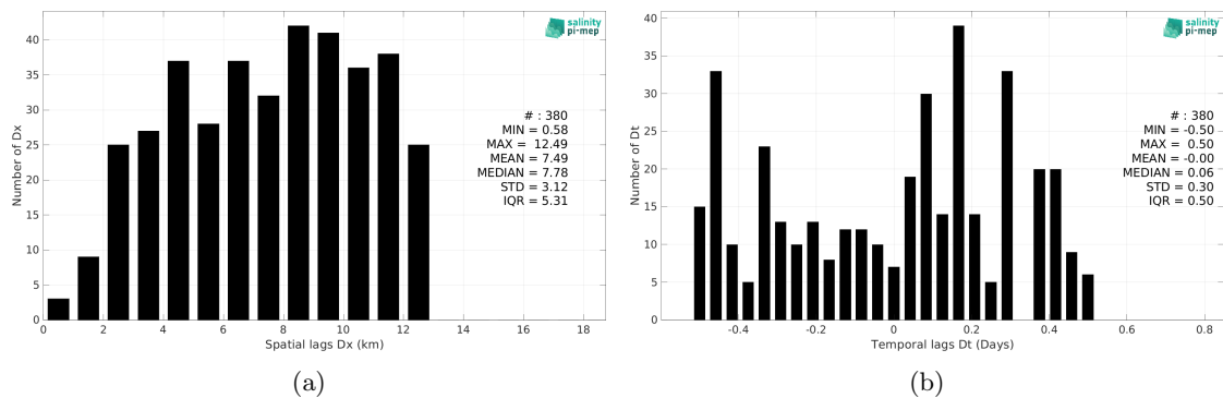
Figure 6: Histograms of the spatial (a) and temporal (b) lags between the location/time of the TSG (Lauge-Koch) measurement and the date of the corresponding SMOS SSS L2Q v333 - 0.25 Deg (CATDS-CPDC) SSS pixel.
