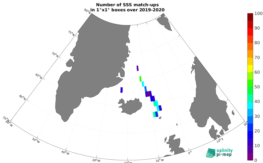
Figure 5: Number of SSS match-ups between TSG (Lauge-Koch) SSS and the SMOS SSS L2Q v333 - 0.25 Deg (CATDS-CPDC) SSS product for the Arctic Ocean Pi-MEP region over 1^\circ \times 1^\circ boxes and for the full satellite product period.
