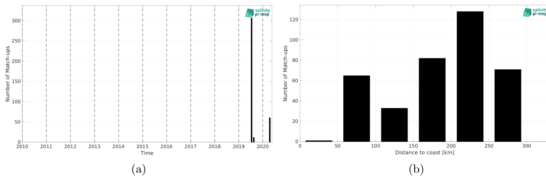
Figure 2: Number of match-ups between TSG (Lauge-Koch) and SMOS SSS L2Q v333 - 0.25 Deg (CATDS-CPDC) SSS as a function of time (a) and as function of the distance to coast (b) over the Arctic Ocean Pi-MEP region and for the full satellite product period.
