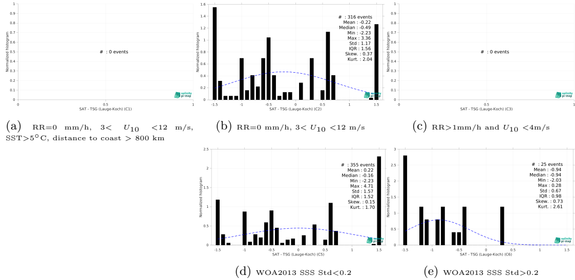
Figure 15: Normalized histogram of \Delta SSS (SMOS SSS L2Q v333 - 0.25 Deg (CATDS-CPDC) - TSG (Lauge-Koch)) for 5 different subdatasets corresponding to: RR=0 mm/h, 3 < U_{10} < 12 m/s, SST > 5°C, distance to coast > 800 km (a), RR=0 mm/h, 3 < U_{10} < 12 m/s (b), RR > 1mm/h and U_{10} < 4 m/s (c), WOA2013 SSS Std < 0.2 (d), WOA2013 SSS Std > 0.2 (e).
