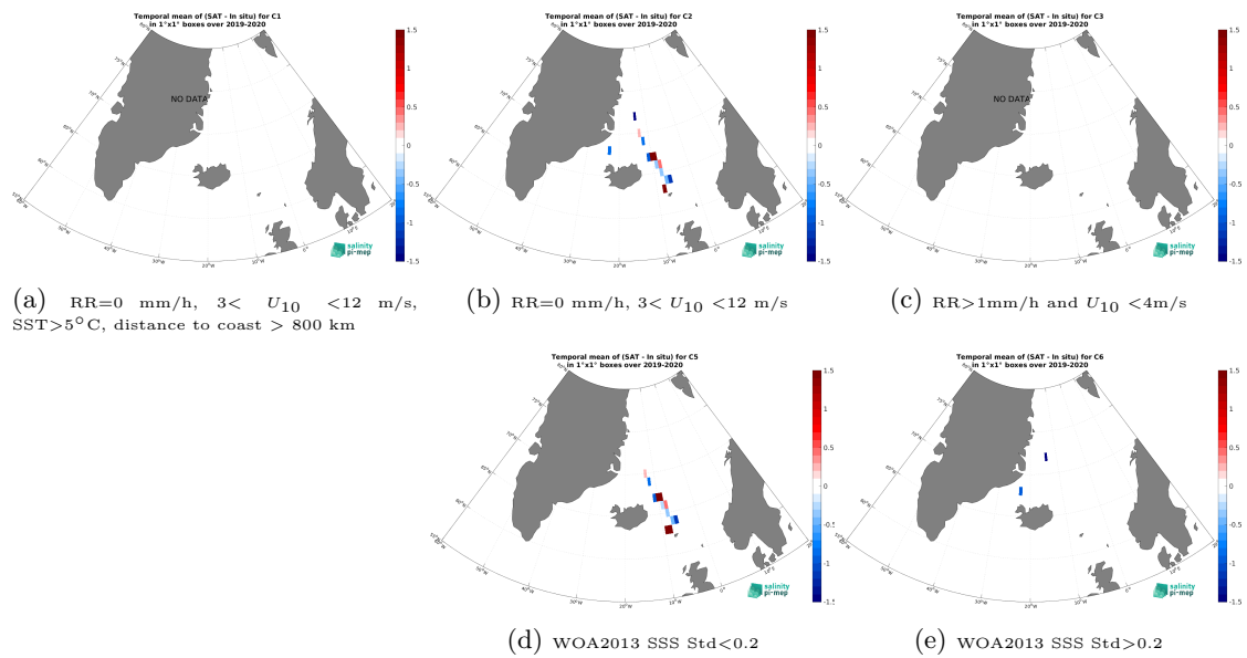
Figure 14: Temporal mean gridded over spatial boxes of size 1^\circ \times 1^\circ of \Delta SSS (SMOS SSS L2Q v333 - 0.25 Deg (CATDS-CPDC) - TSG (Lauge-Koch)) for 5 different subdatasets corresponding to:RR=0 mm/h, 3 < U_{10} < 12 m/s, SST > 5^\circ\text{C} , distance to coast > 800 km (a), RR=0 mm/h, 3 < U_{10} < 12 m/s (b), RR > 1 mm/h and U_{10} < 4 m/s (c), WOA2013 SSS Std < 0.2 (d), WOA2013 SSS Std > 0.2 (e).
