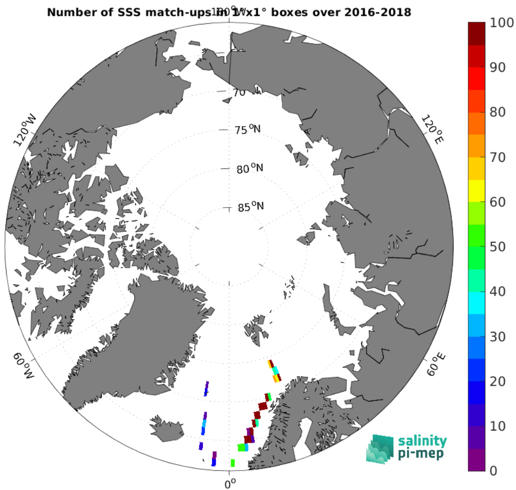
Figure 5: Number of SSS match-ups between TSG (GOSUD-Research-vessel) SSS and the SMOS SSS L2Q v333 - 0.25 Deg (CATDS-CPDC) SSS product for the Arctic Ocean Pi-MEP region over 1^\circ \times 1^\circ boxes and for the full satellite product period.
